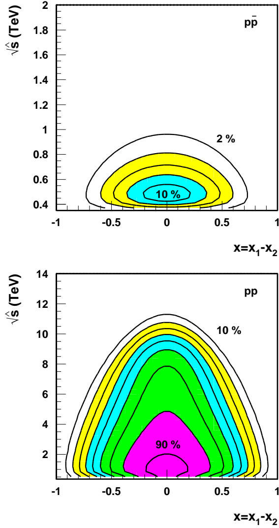
FIG. 11. Relative amount of gluon-gluon initiated processes as a function of x_1 - x_2 = 2P_3(t\bar{t}g)/\sqrt{\hat{s}} and \hat{s} in lowest order, for \sqrt{\hat{s}} = 2 TeV in proton-antiproton collisions and \sqrt{\hat{s}} = 14 TeV in proton-proton collisions. Contour lines go from 2% (white) to 10% (dark) in steps of 2% in the former case and from 10% (white) to 90% (dark) in steps of 10% in the later (CTEQ-1).
