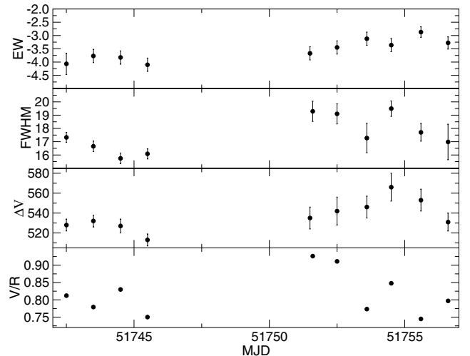
Fig. 10. H\alpha parameters – EW (in Å), FWHM (in Å), peak separation (in \text{km s}^{-1} ) and V/R ratio– for the monitoring campaign in July 2000. There seems to be a high degree of correlation in the evolution of EW , FWHM and peak separation, which is not shared by the V/R ratio.
