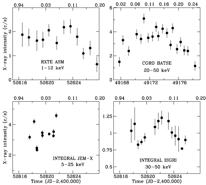
Fig. 1. Long-term light curve of EXO 2030+375 during the X-ray outburst. All light curves except that of CGRO BATSE (Norton et al. 1994) display simultaneous data. ISGRI data are normalized to the mean flux value.
