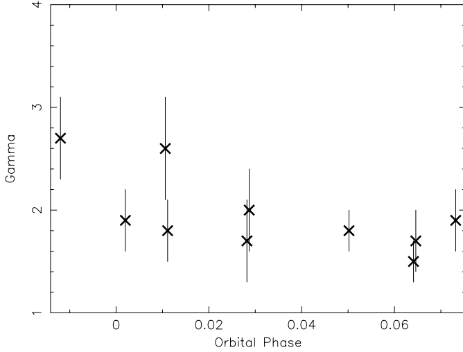
Fig. 5. Photon spectral index of the power law model in the energy range 9–25 versus orbital phase. Error bars are 1\sigma confidence region.
