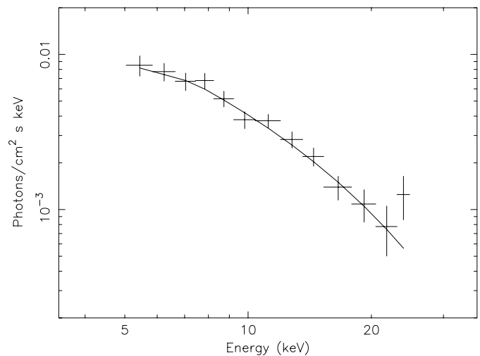
Fig. 4. Energy spectrum of observation 13 (SWID = 002000540010). The continuous line represents a powerlaw with a high energy cutoff.
