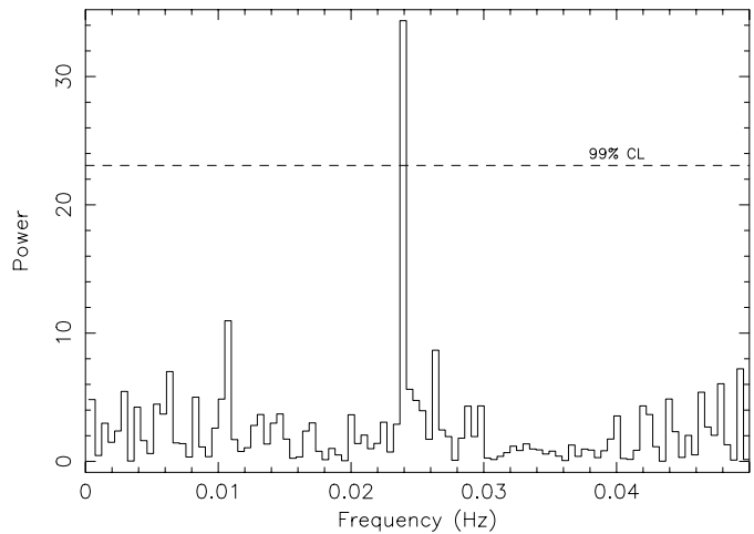
Fig. 3. EXO 2030+375 power spectrum for 1024 frequencies. The dashed line represents the 99% confidence level.
