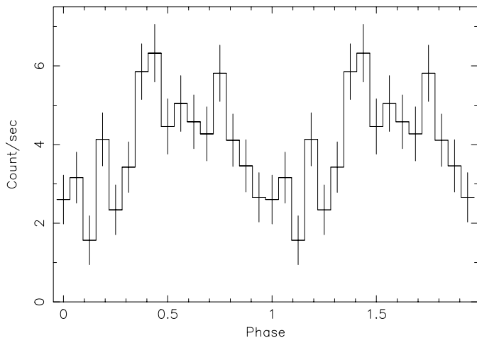
Fig. 2. EXO 2030+375 time-averaged pulse profile of the best detection, SWID = 002000540010.
