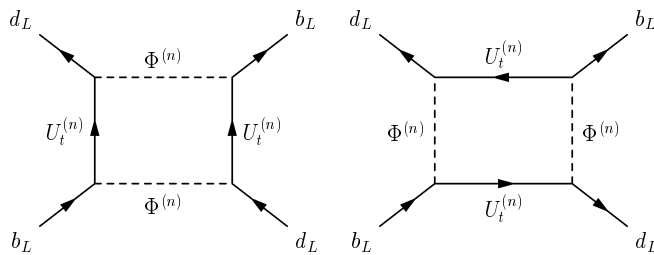
Figure 3.6: Diagrams that contribute to the B^0 - \bar{B}^0 mixing in UED.
