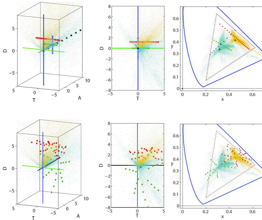
Figure 4.6: Training and test points for the simulation of the psychophysics. Small points represent the training samples of the database (cyan for CIE D65 and yellow for CIE A) and large points represent the different sets of test points. In these plots only a subset of randomly selected training points is shown for better visualization. Top: Black, green and blue dots in the top row are the considered points to simulate the nonlinearity of the A, T, and D mechanisms respectively. In these cases the response is computed using the CIE D65 training set (gray dots). Dark red dots are the considered points to simulate the nonlinearity in a reddish environment using the CIE A training set (light red dots). Top left plot shows the data in the tristimulus ATD space. A zoom around the origin is shown here for better visualization. However note that test points along the achromatic axis spread up to A = 80 . Top center plot show the data in the (T, D) plane. Top right plot shows the data in the CIE xy chromaticity diagram. In this case, the chromatic coordinates of the CIE D65 and CIE A illuminants are also shown for reference (larger gray and red dots respectively). Bottom: Green and red points in the bottom row are the considered points to compute the corresponding pairs using the CIE D65 training set (cyan dots) and the CIE A training set (yellow dots).
