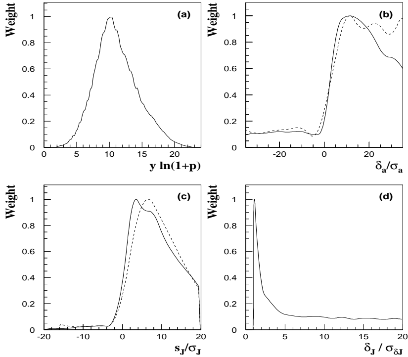
Figure 4.12: Single track weights of B decay products normalized to its maximum value as a function of: (a) the product of the rapidity by the logarithm of the momentum, y \ln(1+p) , for all the tight tracks; (b) the significance S for 2D-tight (dotted line) and 3D-tight (continuous line) tracks; (c) the track-jet abscissa over its error s_J/\sigma_J for 2D-tight (dotted line) and 3D-tight (continuous line) tracks; (d) the track-jet distance over its error \delta_J/\sigma_{\delta_J} for 3D-tight tracks.
