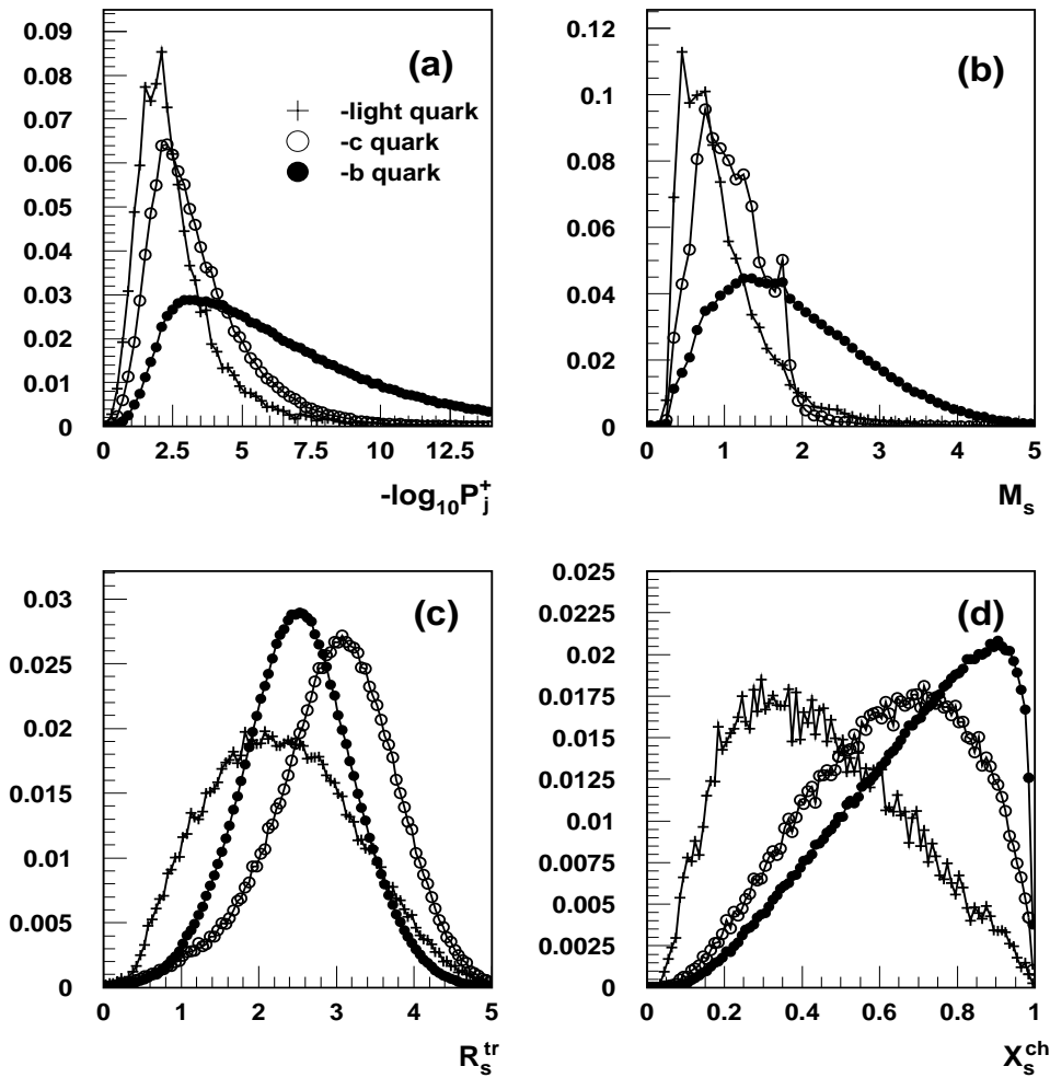
Figure 4.25: Distributions of discriminating variables used in the combined impact parameter tagging: (a) the jet lifetime probability, P_j^+ ; (b) the effective mass distribution of particles included in the secondary vertex, M_s ; (c) the rapidity distribution of tracks included in the secondary vertex with respect to the jet direction, R_s^{tr} ; (d) the fraction of the charged energy distribution of a jet included in the secondary vertex, X_s^{ch} .
