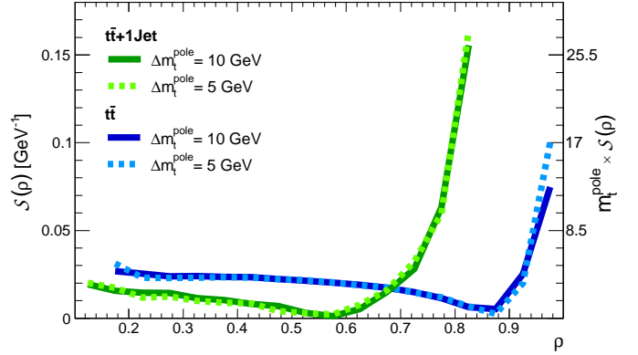
Fig. 5. The sensitivity \mathcal{S}(\rho_s) of \mathcal{R} with respect to the top-quark mass as defined in Eq. (5).
