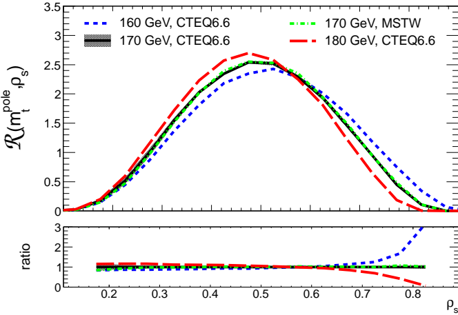
Fig. 4. \mathcal{R}(m_t^{\text{pole}}, \rho_s) calculated at NLO accuracy for different masses m_t^{\text{pole}} = 160, 170 and 180 GeV. For m_t^{\text{pole}} = 170 GeV the scale and PDF uncertainties evaluated as discussed in the text are shown. The ratio with respect to the result for m_t^{\text{pole}} = 170 GeV is shown in the lower plot.
