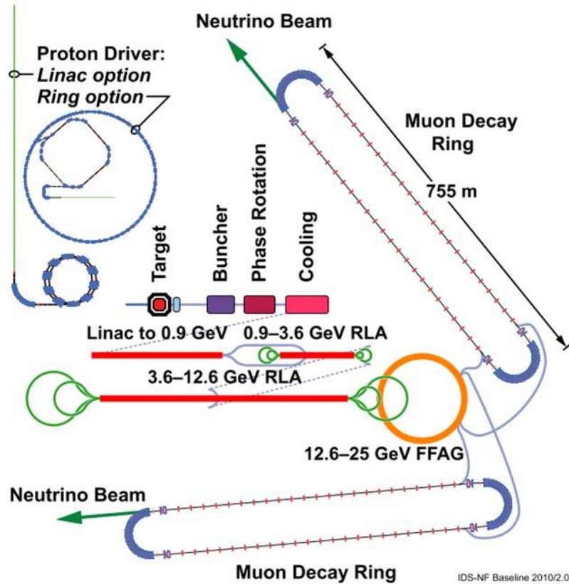
Figure 8: Original baseline layout of the Neutrino Factory.
