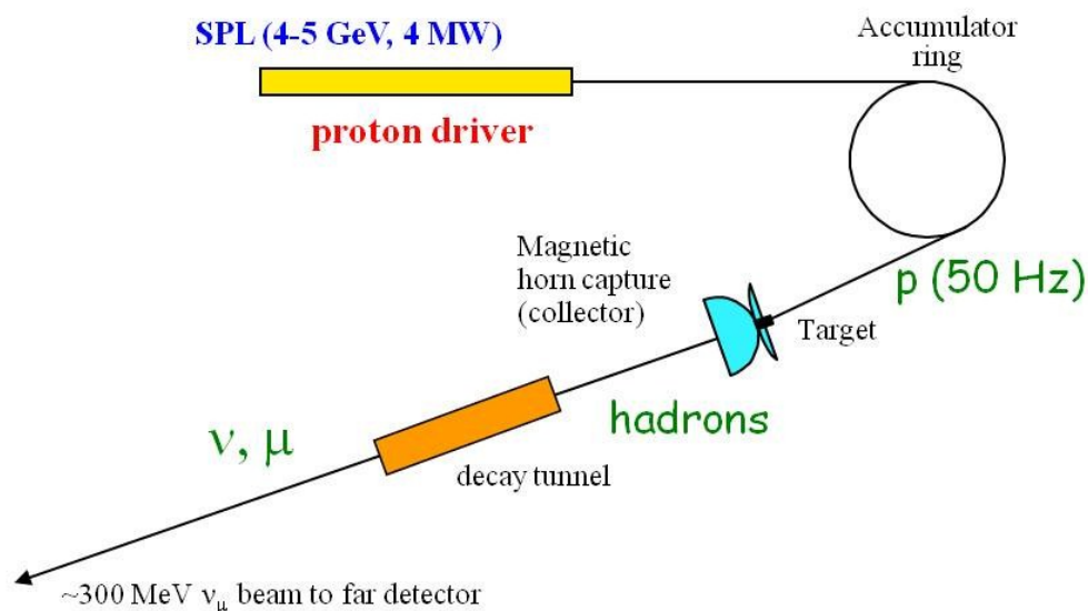
Figure 1: Layout of the CERN to Fréjus Super Beam.
