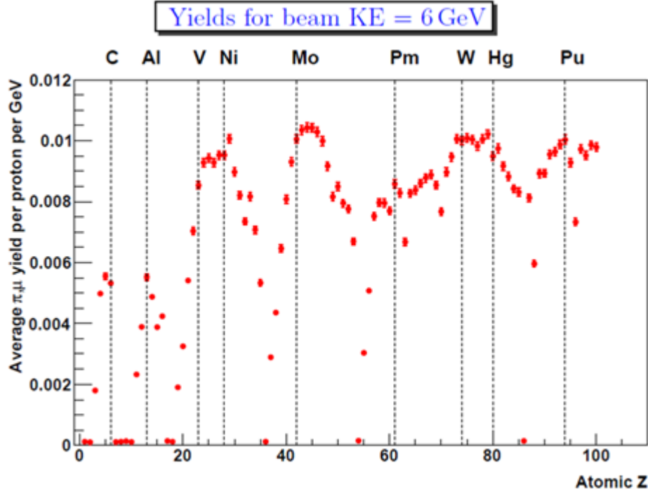
Figure 10: Pion production as a function of atomic number, assuming a cylindrical target 20cm long and 2cm in diameter.
