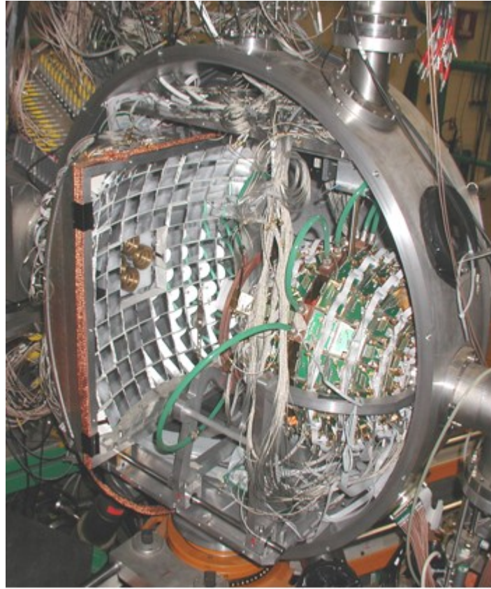
Figure 15: The 8\pi LP experiment used for measurement of the {}^7\text{Li}(d,p){}^8\text{Li} cross-section.
