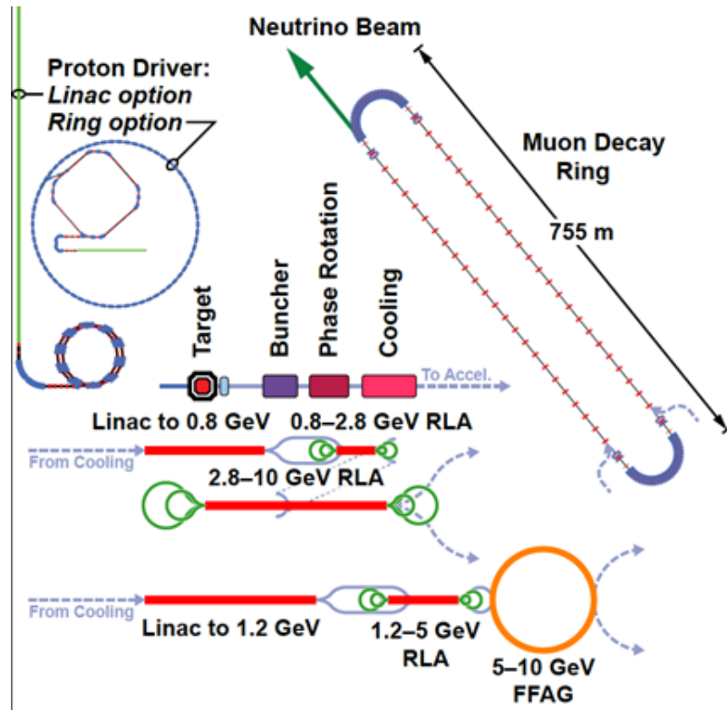
Figure 12: Updated layout for a Neutrino Factory for 10 GeV operation, with only one decay ring. The two options for muon acceleration are shown.
