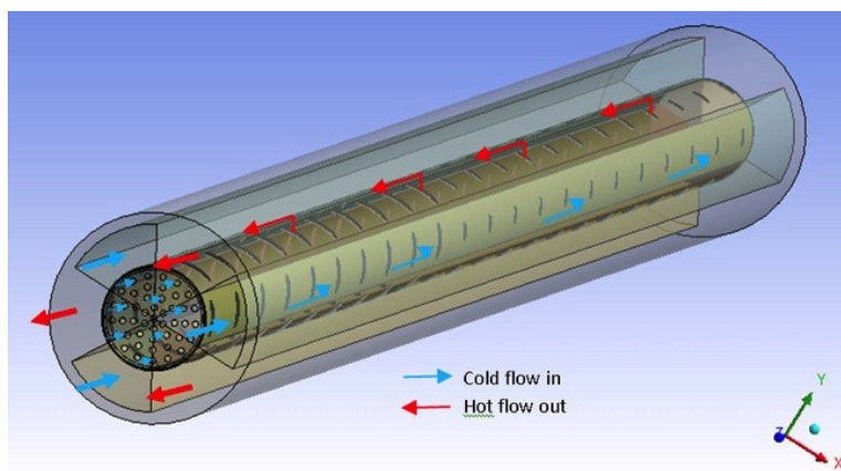
Figure 4: Proposed pebble bed target for the Super Beam.
