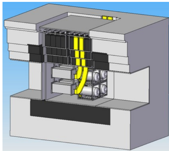
Figure 6: Conceptual design of the section of the target station for the 4 targets and horn systems. The beam enters from the left. The horn pulsing circuits will be mounted on top of the shielding, so the strip lines exit vertically.
