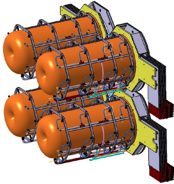
Figure 3: Conceptual engineering design of the 4 target and horn system for the Super Beam.
