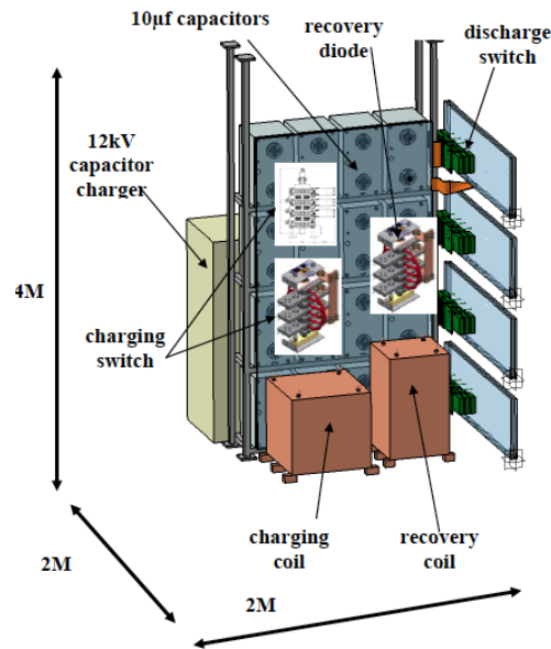
Figure 5: Design of the pulsing system for the Super Beam horns.
