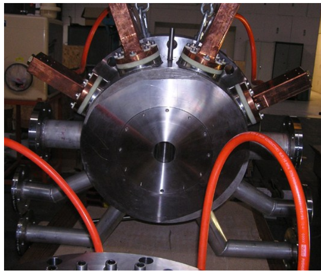
Figure 18: The SEISM 60 GHz ECR source prototype.
