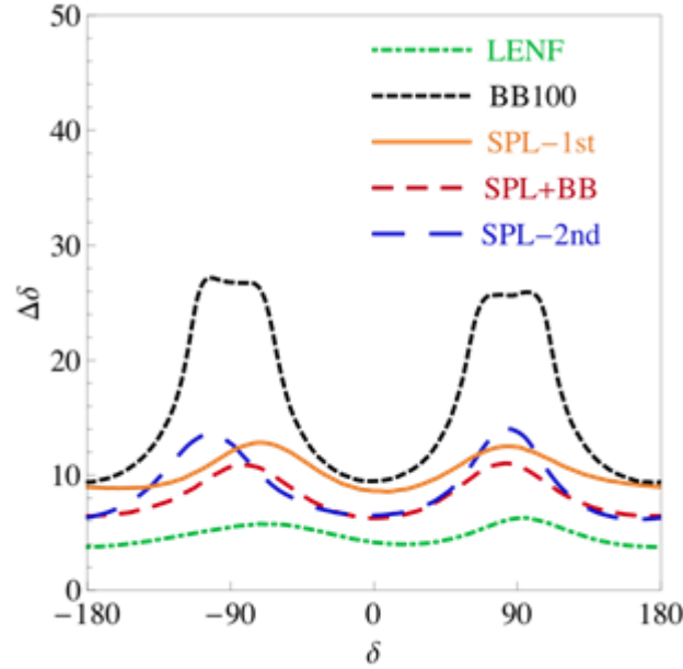
Figure 25: The 1\sigma measurement errors for the CP angle \delta as a function of \delta . The facilities studied are as follows. LENS: the Low Energy Neutrino Factory, with a 10 GeV muon energy, 1.4 \times 10^{21} decays per year and a single 100 kt mass Magnetised Iron Neutrino Detector (MIND) at a baseline of 2000 km; BB100: a \gamma=100 Beta Beam, with 1.3/3.5 \times 10^{18} decays per year of Ne/He and a 500 kt Water Cherenkov detector (MEMPHYS) at Fréjus; SPL-1st: a 4 MW SPL Super Beam with 500 kt water Cherenkov detector at Fréjus, corresponding approximately to the first oscillation maximum; SPL-2nd: as above, but with the detector at Canfranc, corresponding to approximately the second oscillation maximum; SPL+BB: the combination of BB100 and SPL-1st.
