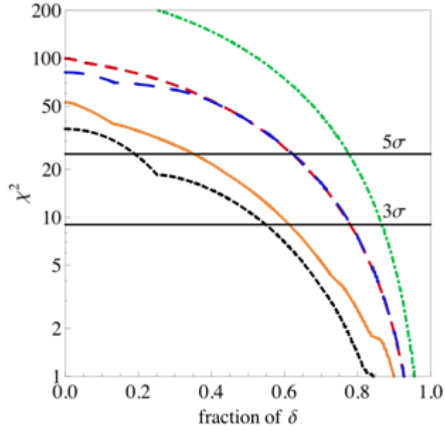
Figure 26: The range of \delta for which a 3 and 5 \sigma measurement of CP violation can be made by the same facilities as in Figure 25.
