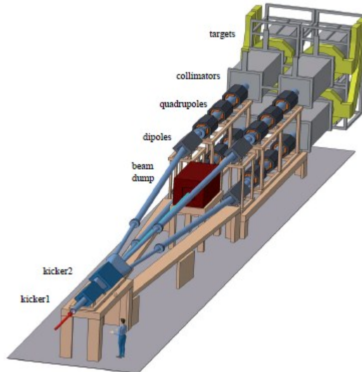
Figure 2: The Super-Beam beam transport and distribution system.
