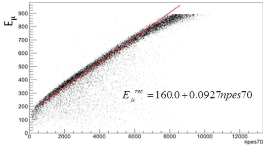
Figure 23: Performance of the MEMPHYS detector. The reconstructed energy of a muon from a neutrino interaction is compared with the real energy, as a function of the number of photoelectrons detected.
