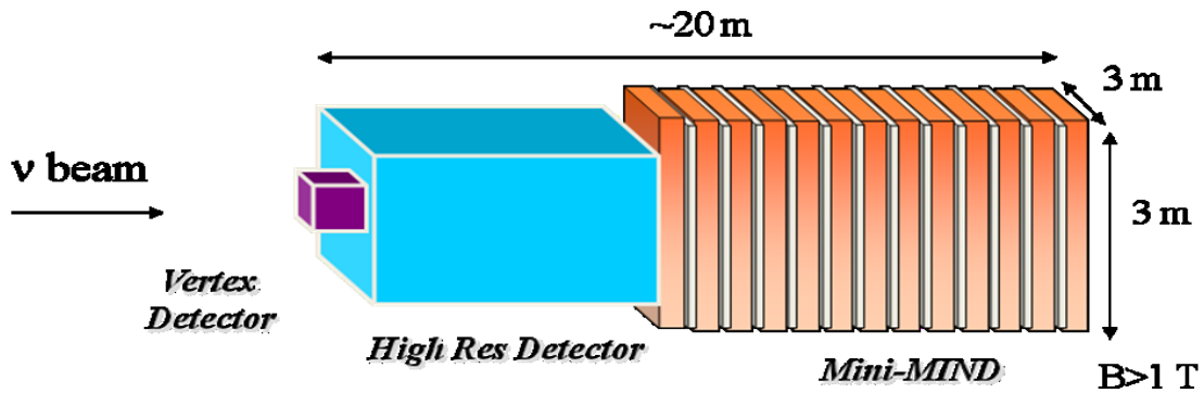
Figure 24: The near detector for a Neutrino Factory.
