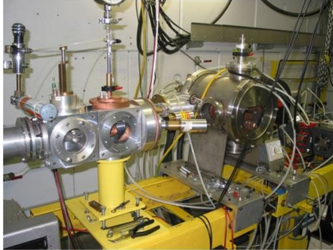
Figure 16: The prototype ion collection device constructed for Beta Beam studies.
