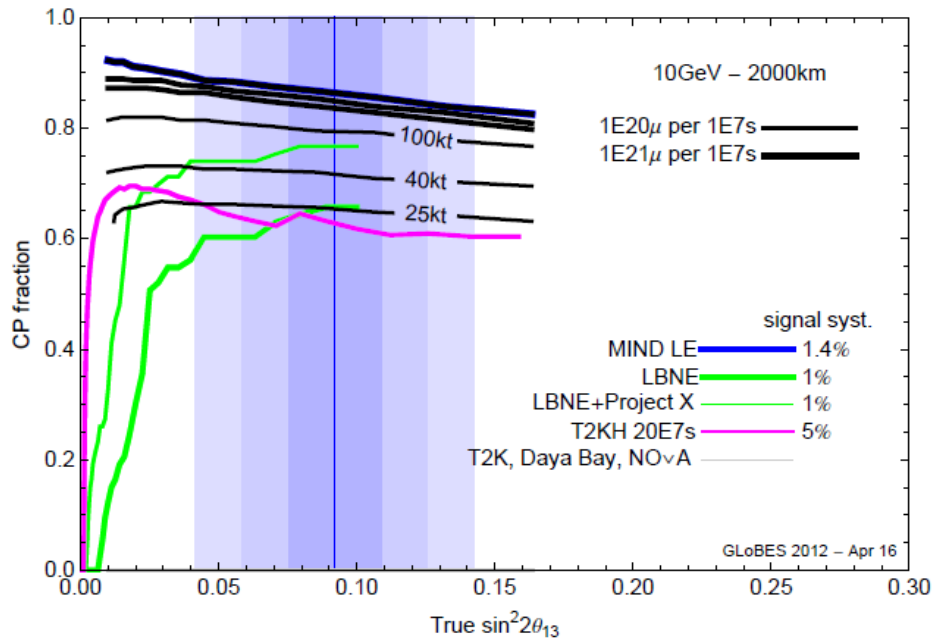
Figure 28: A study of possible staging scenarios for a Neutrino Factory. The plot shows the fraction of the CP angle for which a measurement can be made for various MIND detector masses and the number of neutrinos produced per year. The current measured value of \theta_{13} is shown as a vertical line. The potential of the Neutrino Factory is compared to other possible future facilities in the US (LBNE) and Japan (T2KH). The plot shows that a Neutrino Factory with a factor of 10 smaller neutrino flux than the full 4 MW version and a 25 kt MIND is already competitive.
