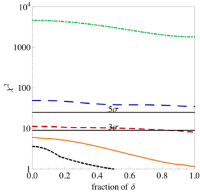
Figure 27: The range of \delta for which a 3 and 5 \sigma measurement of mass hierarchy can be made by for the same facilities as in Figure 25.
