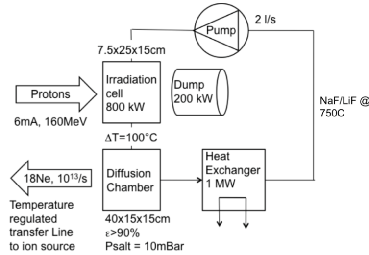
Figure 17: A NaF molten salt loop for the production of {}^{18}\text{Ne} ions.
