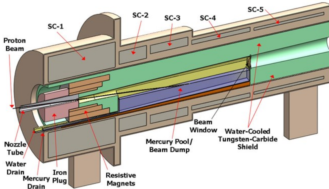
Figure 9: Conceptual layout of the Neutrino Factory pion production target and capture system.
