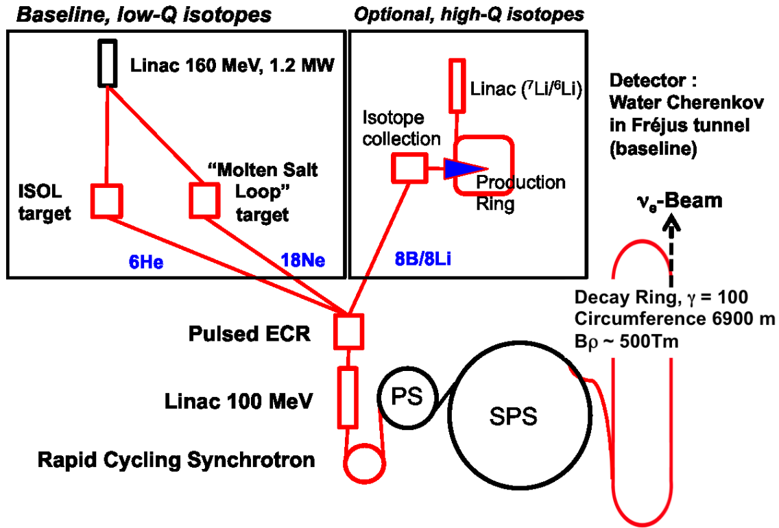
Figure 14: Layout of the CERN Beta Beam.
