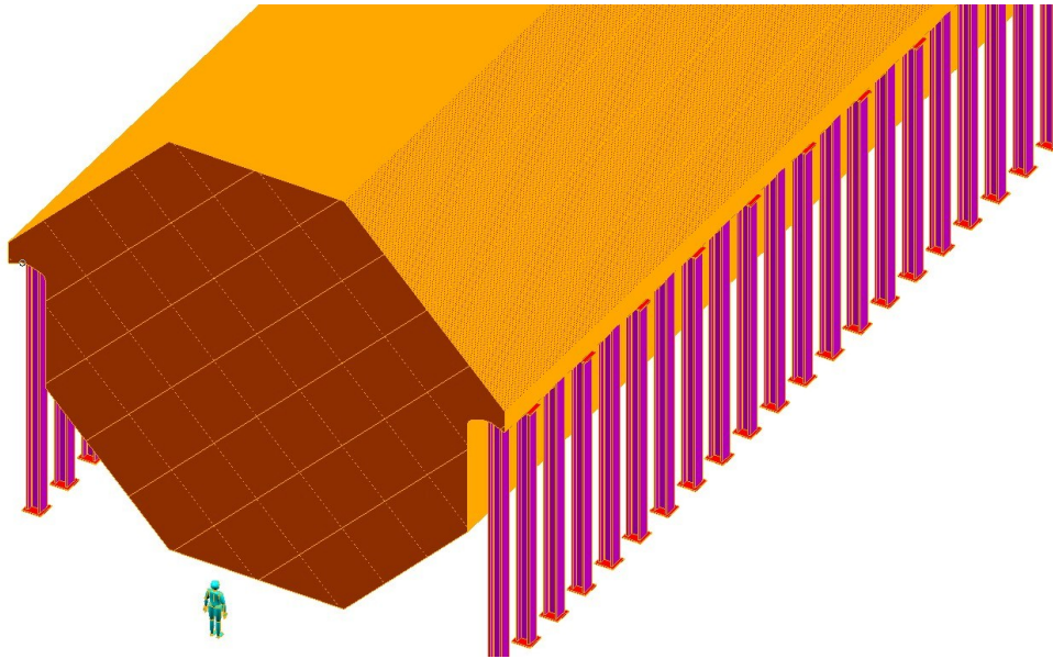
Figure 19: The Magnetised Iron Neutrino Detector for a Neutrino Factory.
