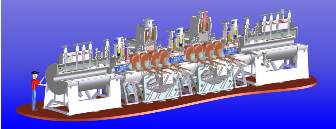
Figure 11: Engineering drawing of the MICE experiment [16]. The central region shows two ionization cooling cells, with instrumentation regions on either side for measuring the parameters of muons entering and leaving these cells.
