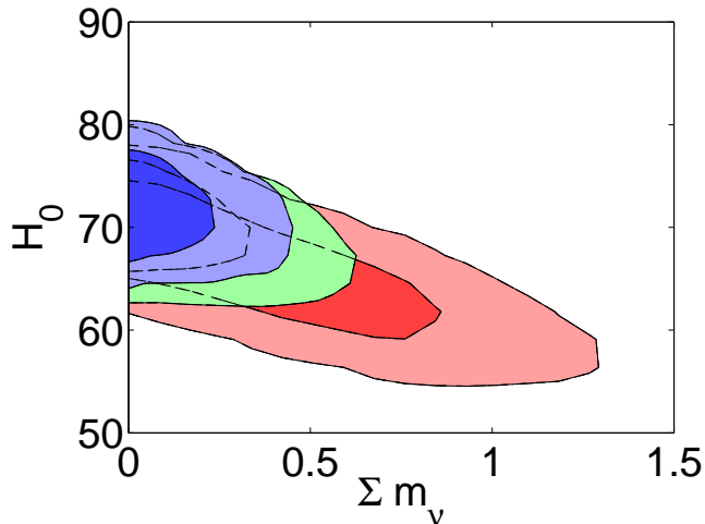
FIG. 1: The red contours show the 68% and 95% CL constraints in the (\sum m_\nu, H_0) plane from our basic WMAP data set. The blue contours show the results from the combination of WMAP and HST data, while the green contours depict the results from the combination of WMAP and SNLS3 data sets. Notice that the strong degeneracy present in the case of WMAP data alone gets alleviated when a prior on H_0 from HST data is added in the analysis. SNIa luminosity distant data are unable to independently determine the Hubble constant H_0 but measure the \Omega_m h^2 quantity, and, since WMAP measures \Omega_m h^2 , the combination of WMAP plus SNIa data is able to determine H_0 .
