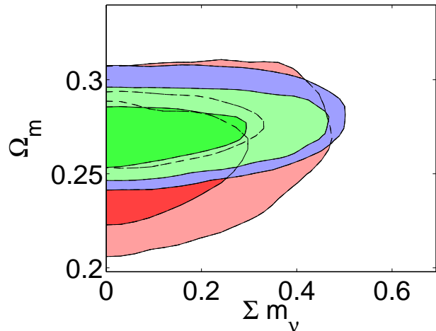
FIG. 2: The red contours show the 68% and 95% CL constraints in the (\sum m_\nu, \Omega_m) plane from WMAP plus HST data sets. The blue contours show the results from the combination of WMAP, HST and galaxy clustering measurements from SDSS-II interpreted in the form of BAO signals, while the green contours depict the results from the combination of WMAP, HST and BAO 2012 data sets. The errors on the \Omega_m parameter are significantly improved when considering either the SDSS-II BAO or the BAO 2012 measurements. Also, due to the higher mean value of \Omega_m when adding BAO information to the WMAP and HST measurements, a slightly higher neutrino mass is allowed.
