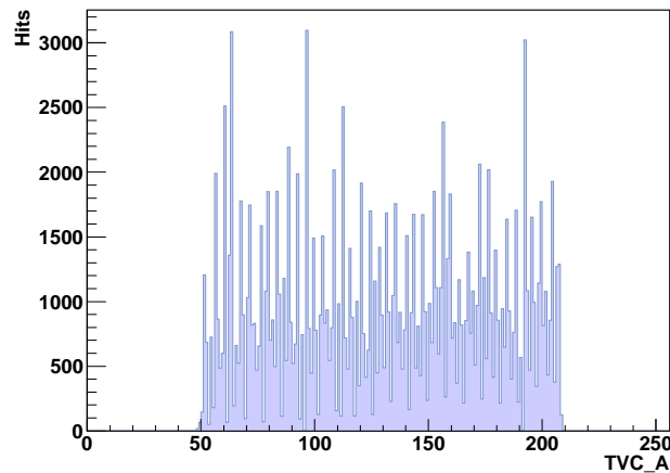
Figure 5.13: Example of a TVC distribution from random signals. Only about 150 channels are useful for timing. The average bin content of these distributions is used to determine the TVC_{min} and TVC_{max} parameters for the two TVC ramps in each ARS.
