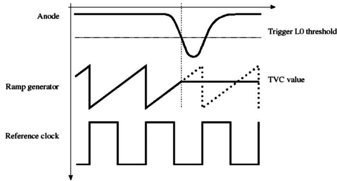
Figure 4.10: Time measurement done inside the ARS. A TVC value is generated when a signal exceeds the L0 threshold.
