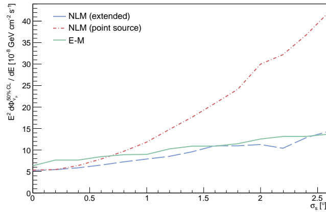
Figure 7.12: Discovery flux as a function of the source extension for a source located at \delta = -70^\circ . This is shown for the E-M algorithm and for the NLM method accounting for the source extension (dashed line) and assuming the point source hypothesis (dash-dot line).
