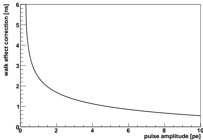
Figure 4.11: Time offset introduced by the walk-effect as a function of the PMT pulse amplitude expressed in units of photo-electrons.
