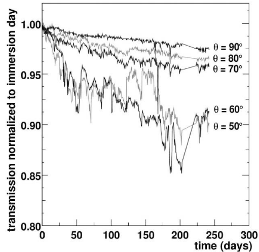
Figure 2.19: Light transmission into the OM as a function of time since the immersion day for five different zenith angles of the photodiodes. The measurements are normalized to unity at immersion day.
