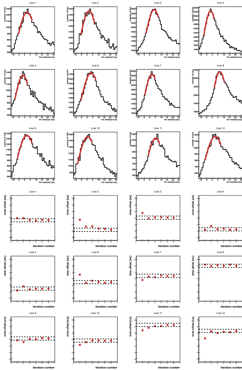
Figure 5.2: (Up) Distributions of probe-line time residuals after a first iteration of the method. The peak is fitted using a Gaussian function whose mean value is taken as T_{\text{line}}^{\text{off}} . (Down) Cumulative time offsets as a function of the iteration number. The dashed lines indicate \pm 1 ns distance from the last iteration point.
