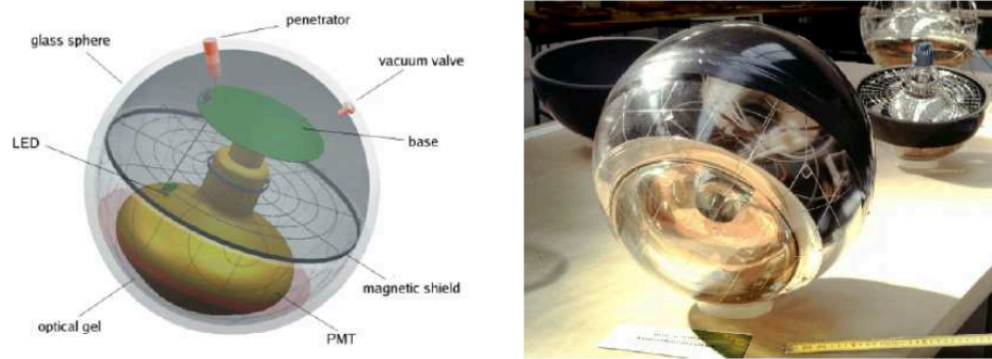
Figure 2.9: Schematic view of an Optical Module showing its different components (left). Picture from an OM at the integration site (right).
