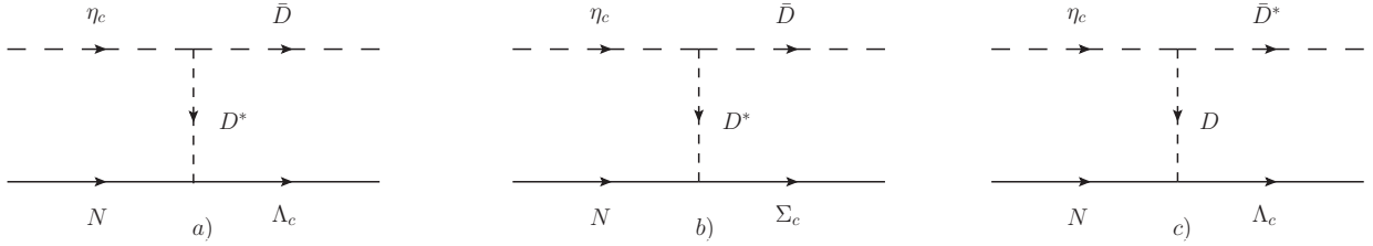
FIG. 4. Diagrams for the \eta_c N \rightarrow \bar{D}\Lambda_c, \bar{D}\Sigma_c, \bar{D}^*\Lambda_c interaction.
