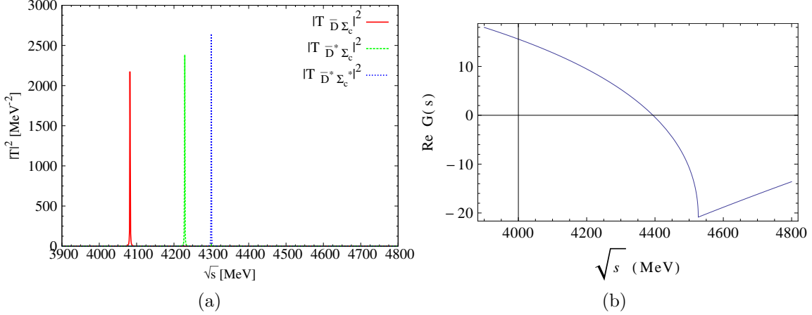
FIG. 7. The results of the J = 1/2 , I = 3/2 sector. (a): The squared amplitudes of three channels except for J/\psi\Delta channel. (b): The real parts of G function in \bar{D}^*\Sigma_c^* channel.
