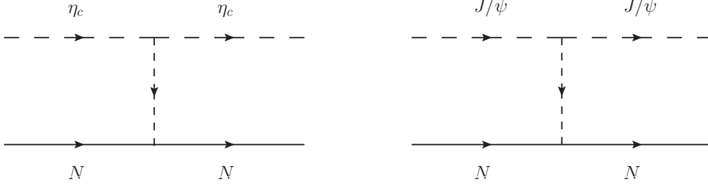
FIG. 3. Diagrams for the \eta_c N \rightarrow \eta_c N and J/\psi N \rightarrow J/\psi N interactions. No vector meson exchanged is allowed.
