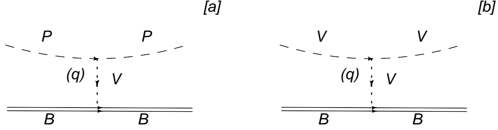
FIG. 2. Diagrams obtained in the effective chiral Lagrangians for interaction of pseudoscalar [a] or vector [b] mesons with the octet or decuplet of baryons.
