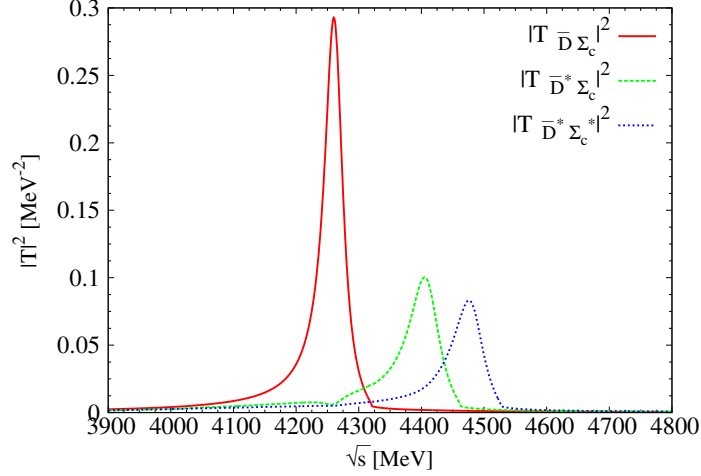
FIG. 8. The squared amplitudes of the J = 1/2 , I = 1/2 sector.
