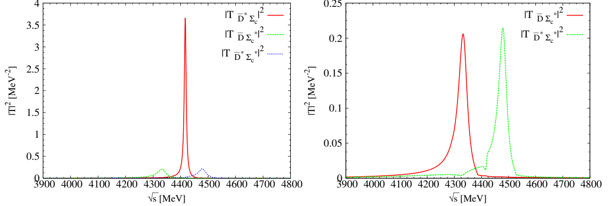
FIG. 9. The results of |T|^2 for the J = 3/2 , I = 1/2 sector. To the right the two small peaks of the left figure magnified.
