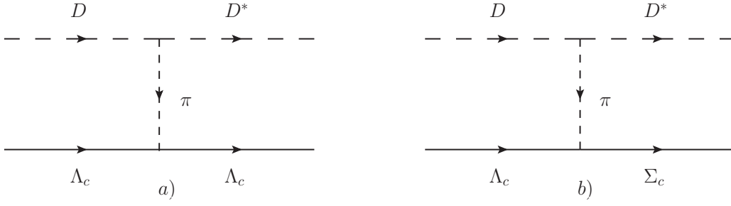
FIG. 5. Diagrams for the pion exchange in the transition of D , D^* .
