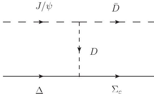
FIG. 6. Diagrams for the J/\psi\Delta \rightarrow \bar{D}\Sigma_c interaction.
