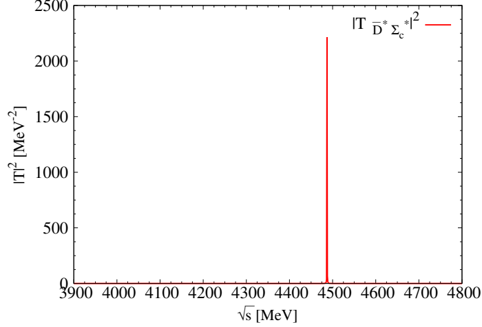
FIG. 10. The results of |T|^2 for the J = 5/2 , I = 1/2 sector.
