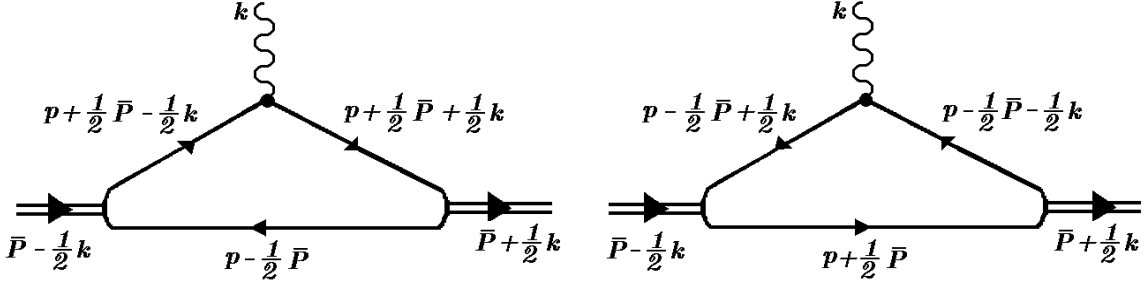
FIG. 7: Triangle diagram contributing to the pion form factor.
