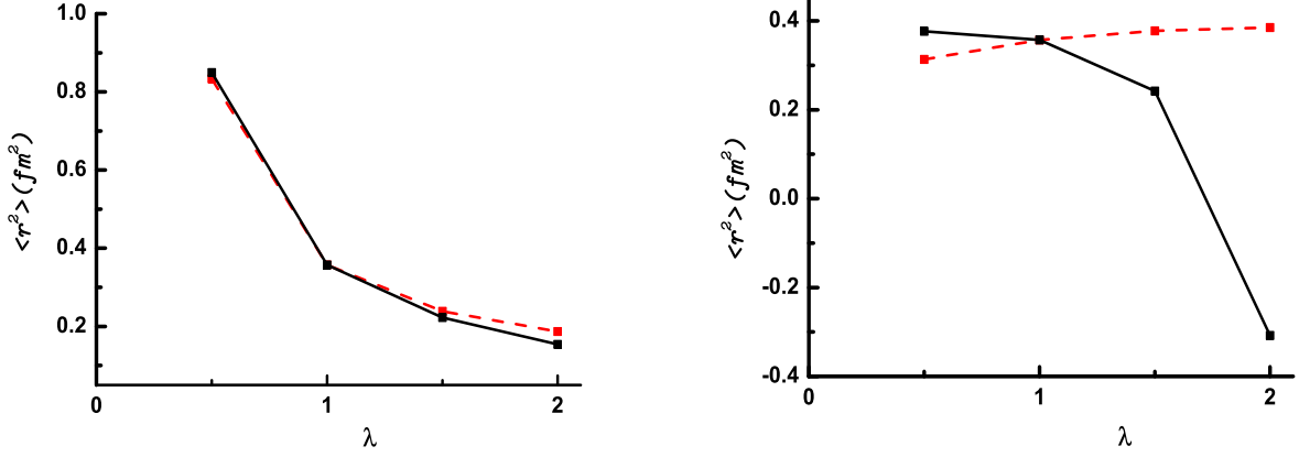
FIG. 10: Sensitivity of \langle r^2 \rangle in fm 2 for the pion in relation with the propagator parameters in the scenario S2. On the left we have \langle r^2 \rangle in relation with \lambda \cdot \Lambda_m for \lambda = 0.5, 1, 1.5 and 2 (dashed curve) and \langle r^2 \rangle in relation with \lambda \cdot \alpha_m for the same values of \lambda (full curve). On the right, the dotted curve represents the \langle r^2 \rangle in relation with \lambda \cdot \Lambda_z and the full curve gives the \langle r^2 \rangle for the pion in relation with \lambda \cdot \alpha_z , for \lambda = 0.5, 1, 1.5 and 2. The full curve gives the msr in fm 2 for the pion in relation with \lambda \cdot \alpha_z for the same values of \lambda .
