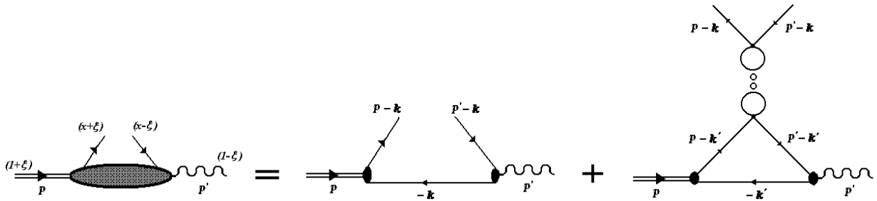
FIG. 3: Diagrams contributing to the TDA. We have depicted diagrams in which a quark u is change into a quark d by the bilocal current. There are similar diagrams in which the antiquark \bar{d} is changed into a \bar{u}
