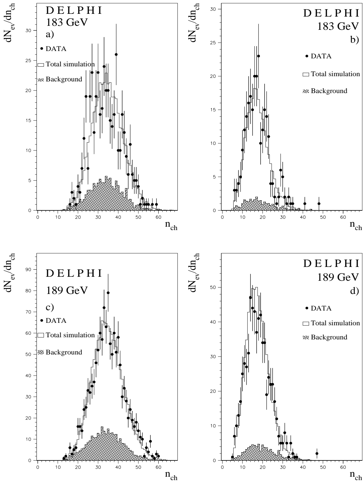
Figure 1: Charged particle multiplicity distributions for (a) the (4q) events and (b) the (2q) events at 183 GeV, for (c) the (4q) events and (d) the (2q) events at 189 GeV. The error bars in the data represent the statistical errors. The shaded areas represent the background contribution; the histograms are the sum of the expected signal and background
