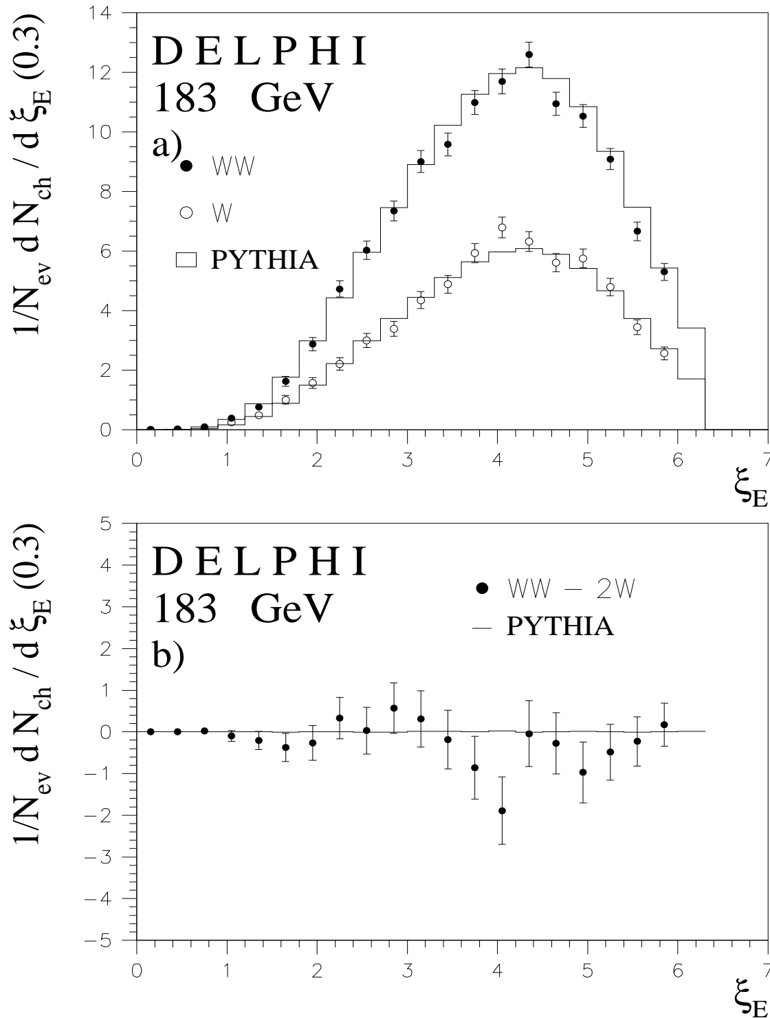
Figure 5: (a) Corrected \xi_E distributions of charged particles for (4q) events (closed circles) and (2q) events (open circles), at 183 GeV, compared to simulation without colour reconnection. The error bars in the data represent the statistical errors. The difference between (4q) and twice (2q) is shown in (b).
