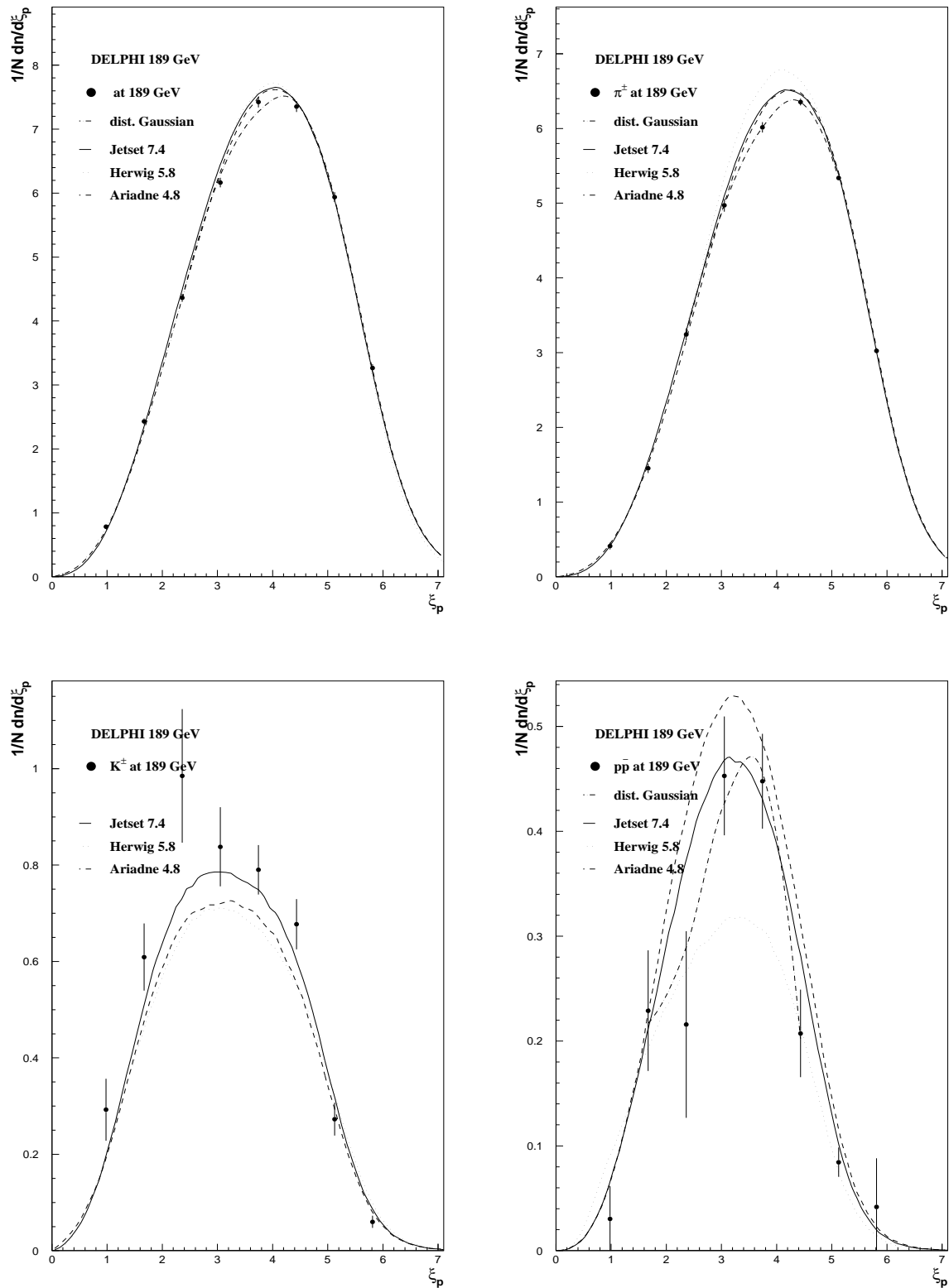
Figure 9: \xi_p distributions (efficiency corrected and background subtracted) for charged particles, pions, kaons and protons in q\bar{q} events at 189 GeV. Data (points) are compared to the prediction from JETSET (solid line). Only the statistical uncertainties are shown. The dashed dotted line shows a fit to equation (3).
