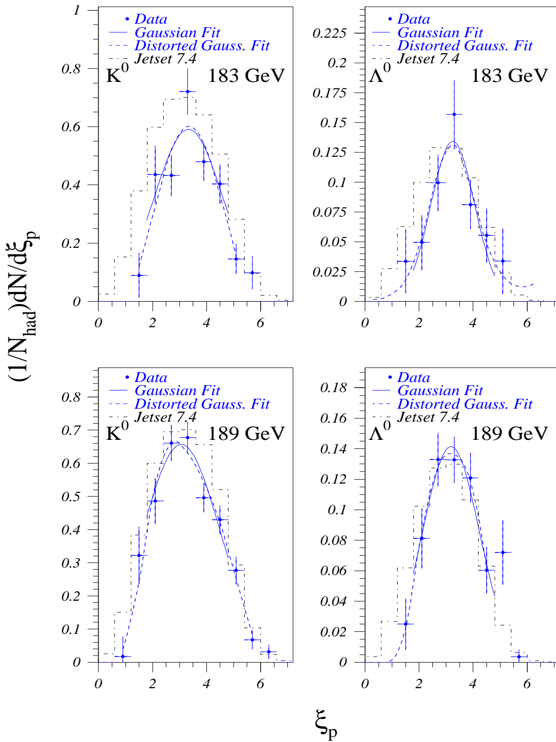
Figure 12: \xi_p distributions (efficiency corrected and background subtracted) for neutral Kaons and neutral Lambdas in e^+e^- \rightarrow q\bar{q} at 183 GeV and 189 GeV respectively, for data (points), and simulation using JETSET (dashed-dotted histogram). The full curves show the fit of the data to a Gaussian and the dashed ones to a distorted Gaussian. The error bars represent only the statistical error.
