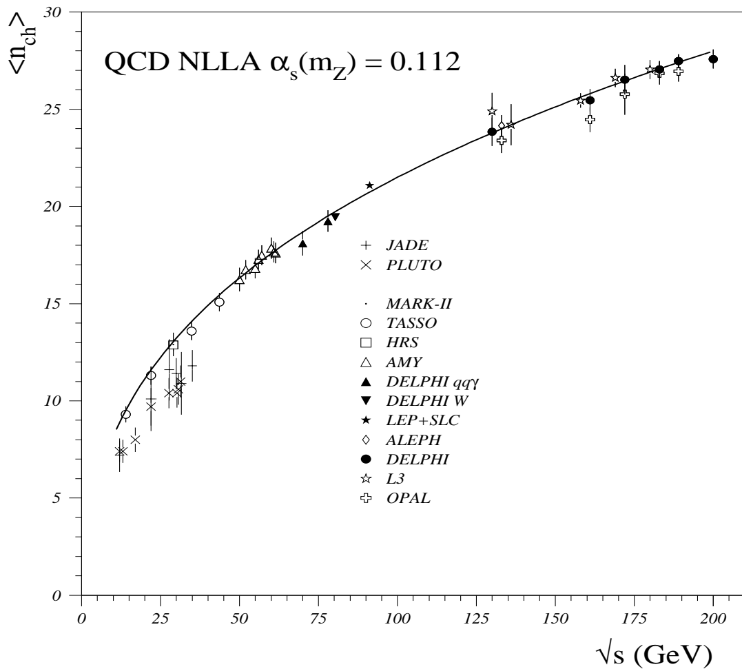
Figure 15: Measured average charged particle multiplicity in e^+e^- \rightarrow q\bar{q} events as a function of centre-of-mass energy \sqrt{s} . DELPHI high energy results are compared with other experimental results and with a fit to a prediction from QCD in Next to Leading Order. The error bars represent the sum in quadrature of the statistical and the systematic uncertainties. Some points are slightly shifted on the abscissa for clarity. The average charged multiplicity in W decays is also shown at an energy corresponding to the W mass. The measurements have been corrected for the different proportions of b\bar{b} and c\bar{c} events at the various energies.
