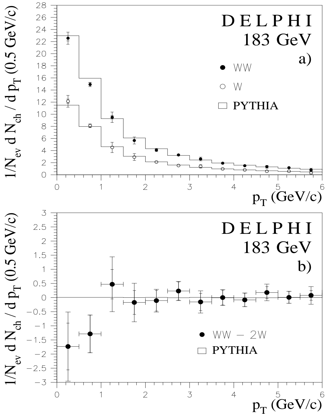
Figure 7: (a) Corrected p_T distributions of charged particles for (4q) events (closed circles) and (2q) events (open circles), compared to simulation without colour reconnection, at 183 GeV. The internal error bars in the data represent the statistical error and the external error bars represent the sum in quadrature of the statistical and systematic errors. The difference between (4q) and twice (2q) is shown in (b).
