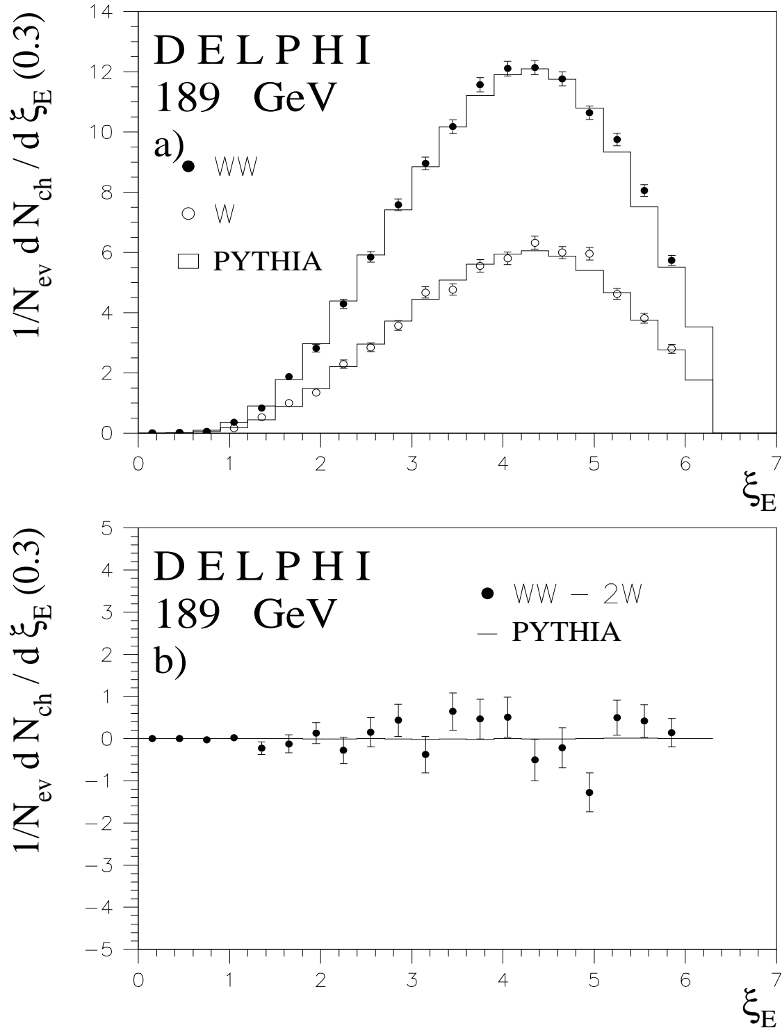
Figure 4: (a) Corrected \xi_E distributions of charged particles for (4q) events (closed circles) and (2q) events (open circles), at 189 GeV, compared to simulation without colour reconnection. The error bars in the data represent the statistical errors. The difference between (4q) and twice (2q) is shown in (b).
