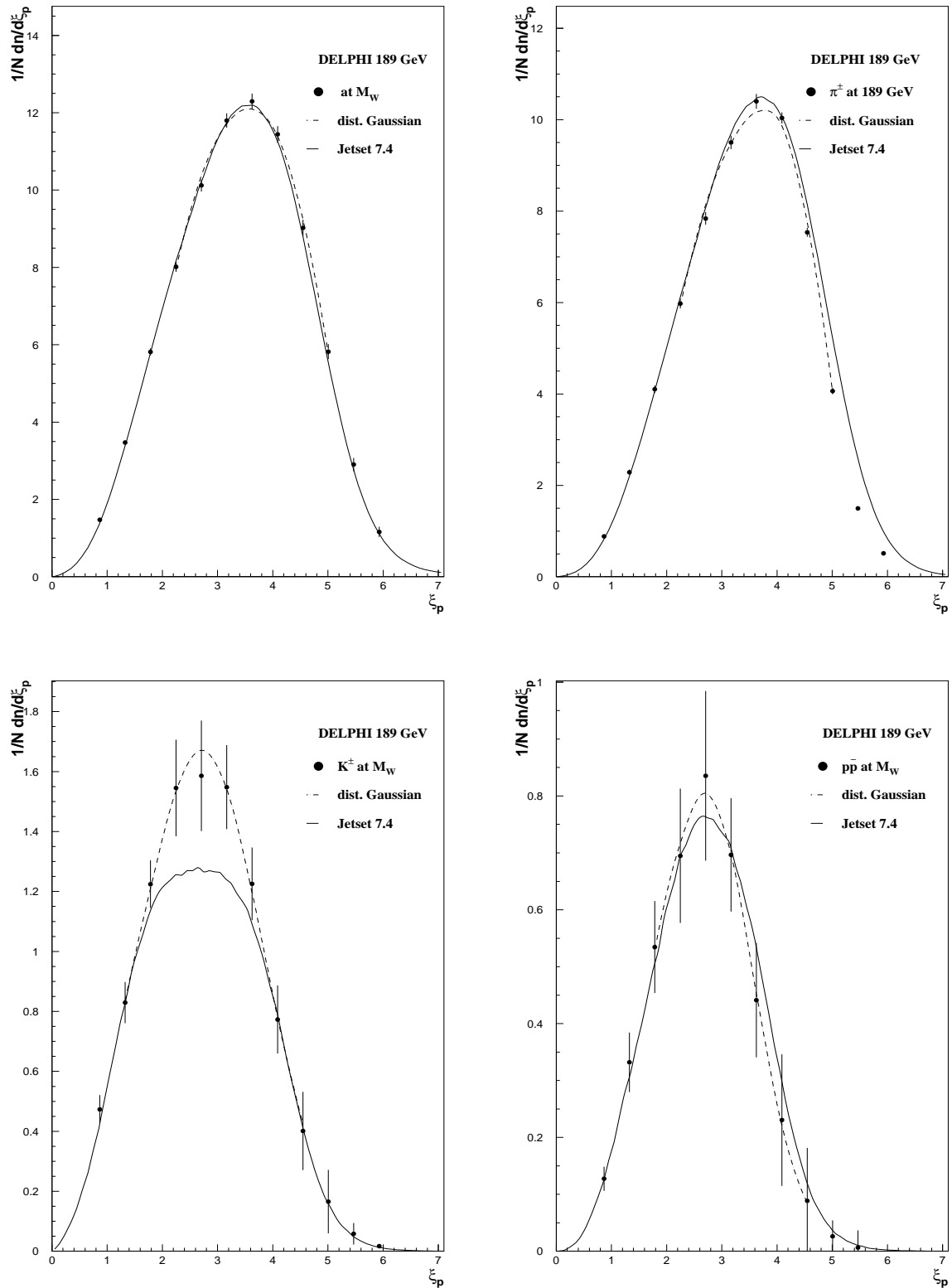
Figure 10: \xi_p distributions (efficiency corrected and background subtracted) for charged particles, pions, kaons and protons in fully hadronic WW events at 189 GeV. Data (points) which have been boosted back to the W rest-frame, compared to the prediction from JETSET (solid line). Only the statistical uncertainties are shown. The dashed dotted line shows a fit to equation (3).
