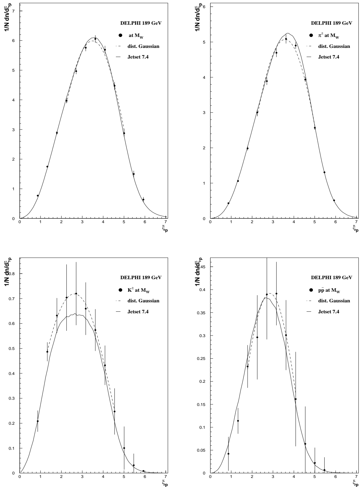
Figure 11: \xi_p distributions (efficiency corrected and background subtracted) for charged particles, pions, kaons and protons in semileptonic WW events at 189 GeV. Data (points) which have been boosted back to the W rest-frame, compared to the prediction from JETSET (solid line). Only the statistical uncertainties are shown. The dashed dotted line shows a fit to equation (3).
