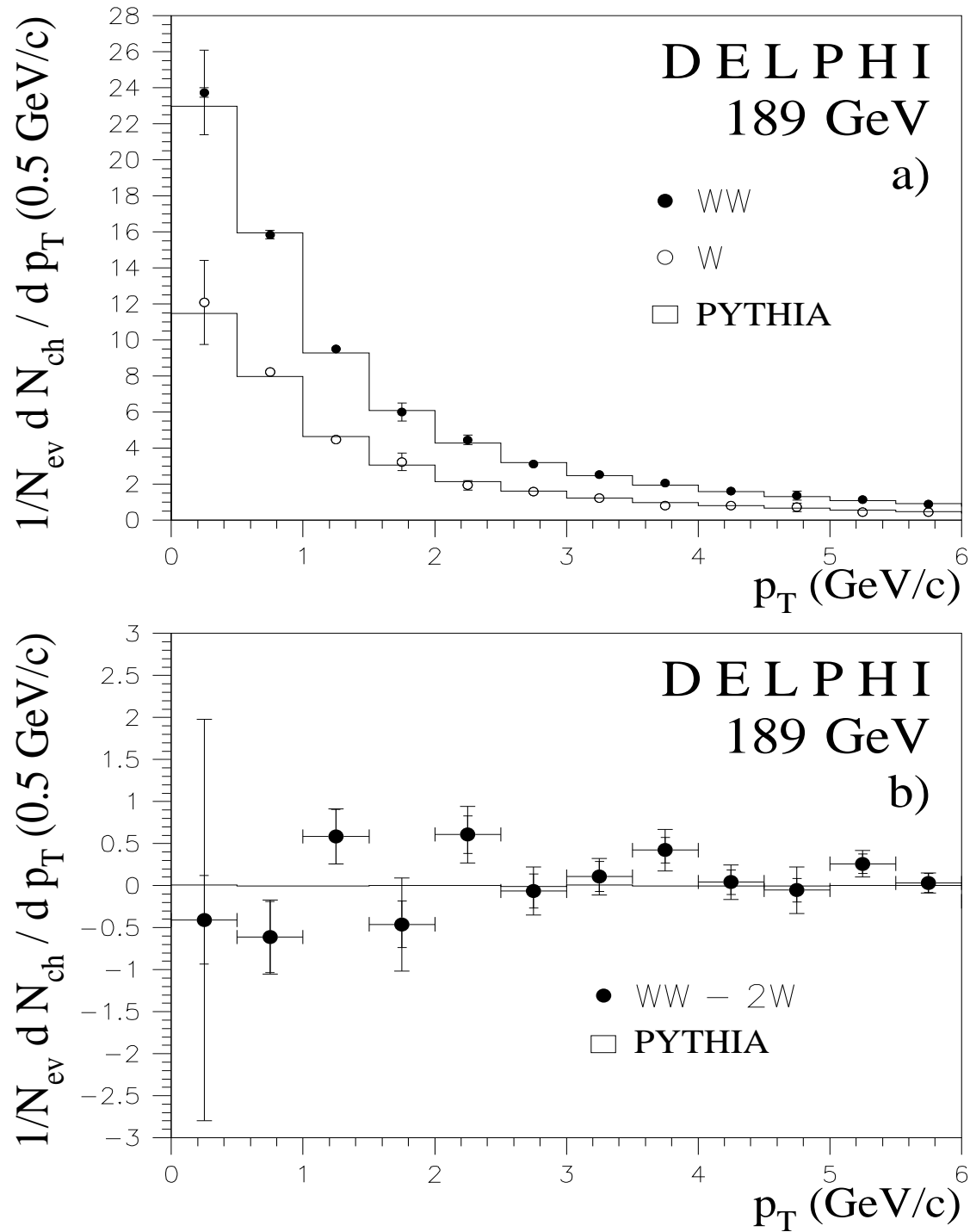
Figure 6: (a) Corrected p_T distributions of charged particles for (4q) events (closed circles) and (2q) events (open circles), compared to simulation without colour reconnection, at 189 GeV. The internal error bars in the data represent the statistical error and the external error bars represent the sum in quadrature of the statistical and systematic errors. The difference between (4q) and twice (2q) is shown in (b).
