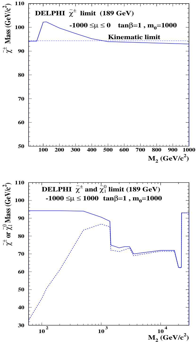
Figure 4: Limits on M_{\tilde{\chi}_1^\pm} and M_{\tilde{\chi}_1^0} for \tan\beta=1 and m_0 = 1000 GeV/c 2 are shown as functions of M_2 . The upper figure shows the lower limit on M_{\tilde{\chi}_1^\pm} (solid curve) for -1000 GeV/c 2 \leq \mu \leq 0 resulting from searches for neutralinos and charginos. The dashed line shows the kinematic limit for chargino pair-production. The lower part of the figure shows the limit on M_{\tilde{\chi}_1^\pm} (solid curve) and M_{\tilde{\chi}_1^0} (dashed curve) for -1000 GeV/c 2 \leq \mu \leq 1000 GeV/c 2 . The region of M_2 < 55 GeV/c 2 is excluded (see figure 2).
