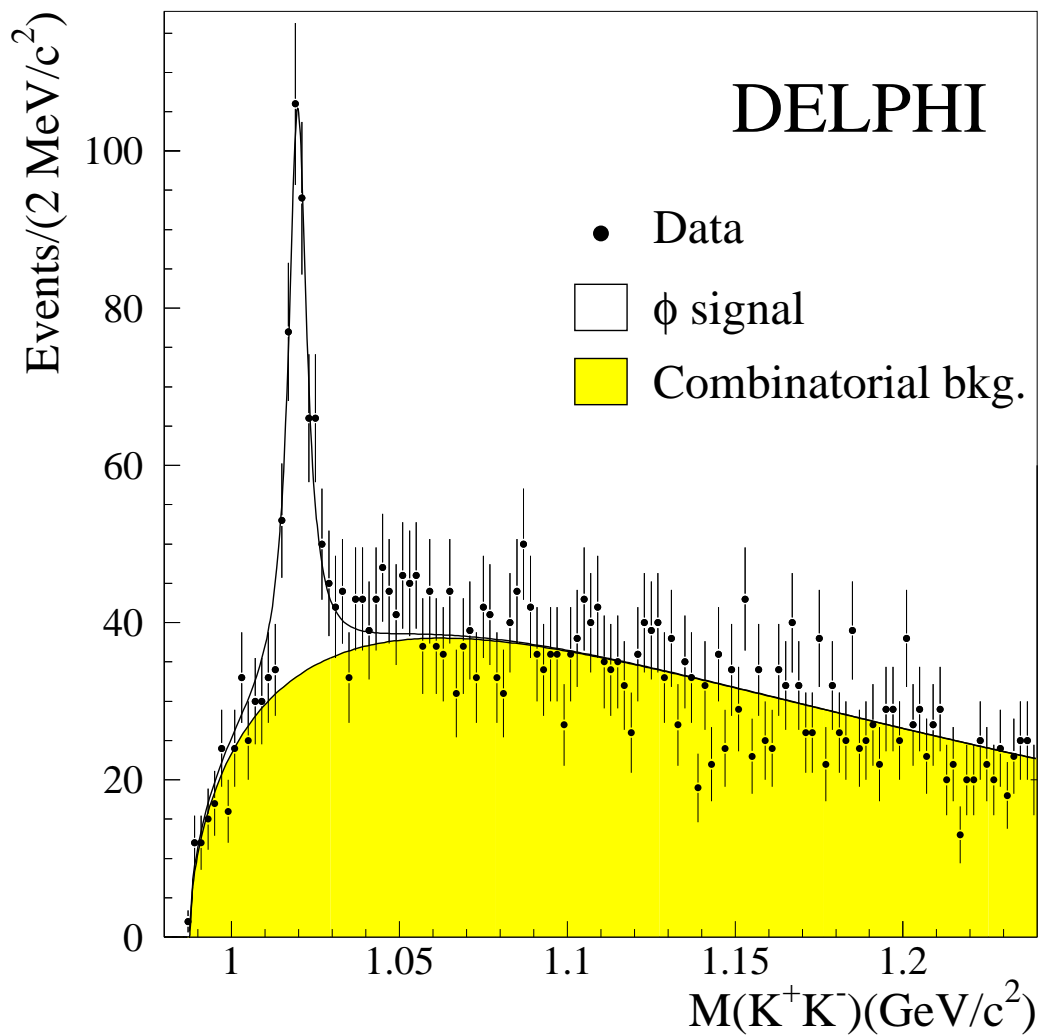
Figure 4: K^+K^- invariant mass distribution of the \phi lh candidates. The curves show the result of the fit described in the text (the signal and the combinatorial background components are represented by the white and shaded histograms respectively).
