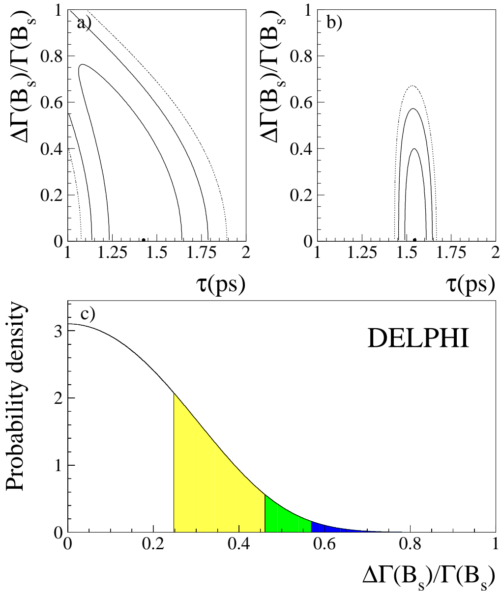
Figure 10: a) 68%, 95% and 99% C.L. contours of the negative log-likelihood in the plane \tau(\equiv 1/\Gamma_{B_s})-\Delta\Gamma_{B_s^0}/\Gamma_{B_s^0} evaluated on the D_s\ell sample. b) Same as a) but with the constraint \tau = \tau_{B_d^0} . c) Probability density distribution for \Delta\Gamma_{B_s^0}/\Gamma_{B_s^0} ; the three shaded regions show the limits at 68 %, 95% and 99% C.L. respectively.
