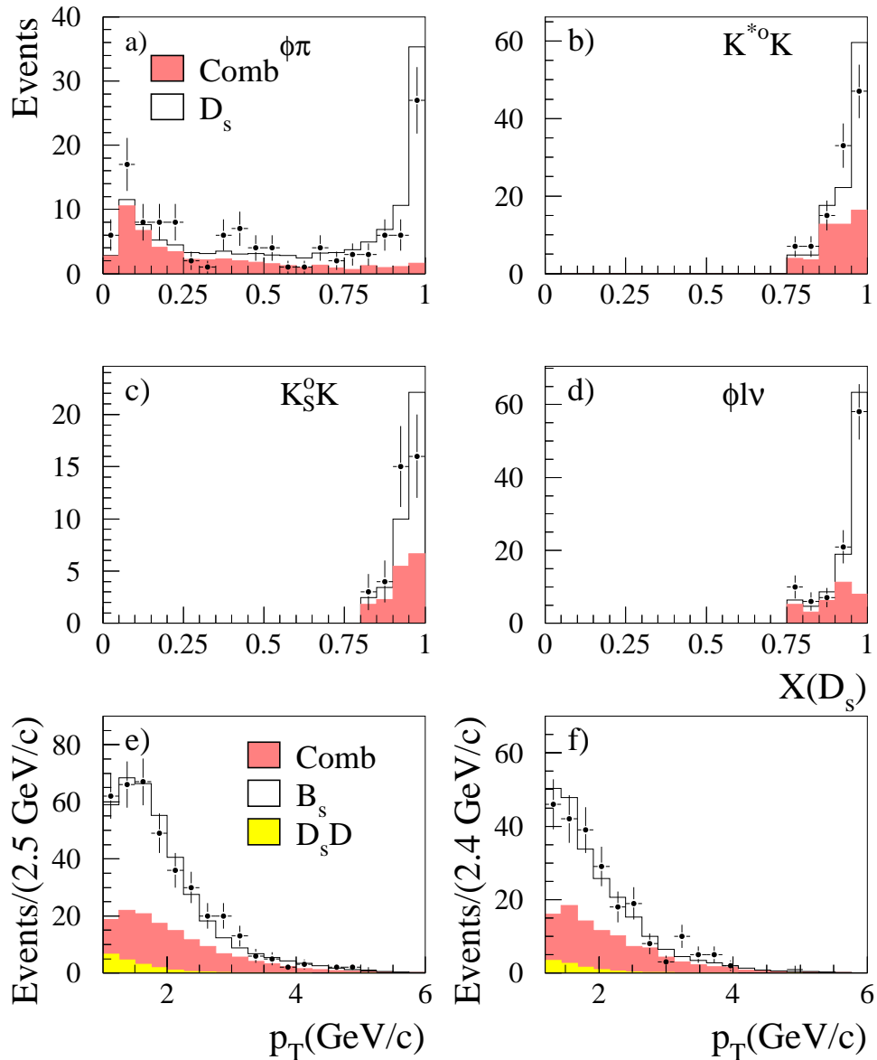
Figure 5: The plots illustrate the agreement between data and simulation for the variables used in the estimate of the B_s^0 purity on an event by event basis. a), b), c) and d) show the X_{D_s} distributions for the channels \phi\pi , \bar{K}^{*0}K , K_S^0 K and \phi l^+ respectively. White histograms and shaded histograms represent the signal and the background respectively. e) and f) show the p_T distributions for the samples selected with p_T > 1 GeV/c ( \phi\pi^+ and \phi l^+\nu ) and p_T > 1.2 GeV/c (all the others) respectively. For the p_T distribution the D_s\bar{D} and the combinatorial background are considered separately.
