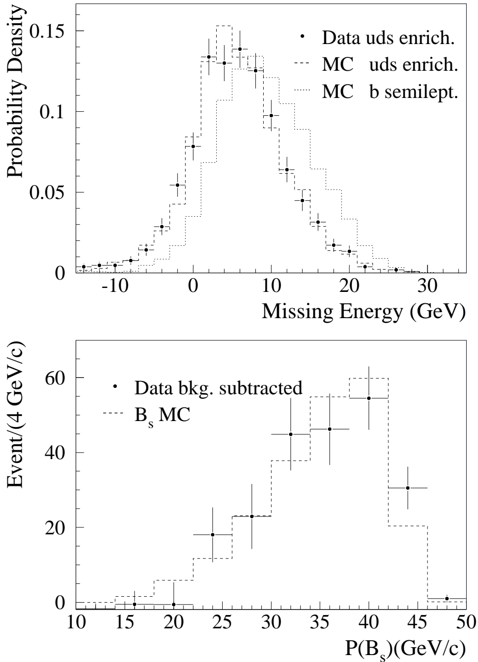
Figure 6: The plot on the top shows the comparison between data and the simulation for the missing energy distribution after correction (see Section 3.6). The data (dots with error bars) and the simulation (dashed histogram) are enriched in light quark events. The dotted histogram shows the missing energy distribution in simulated b semileptonic decays. The plot on the bottom shows the comparison between the B_s^0 momentum distribution for simulated events and the one estimated from data in the signal region by subtracting the B_s^0 momentum distribution of events in the D_s side bands from that of the events in the signal region.
