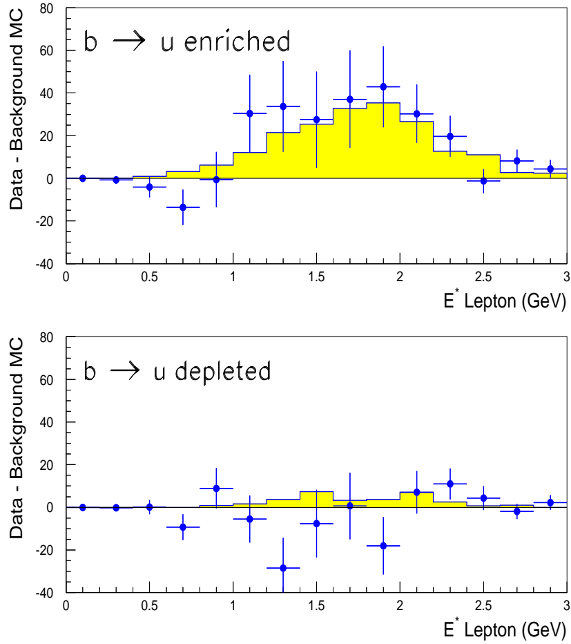
Figure 7: Background subtracted E_\ell^* distributions: the b \rightarrow u enriched decays with M_X < 1.6 \text{ GeV}/c^2 (upper plot) and b \rightarrow u depleted decays with M_X < 1.6 \text{ GeV}/c^2 (lower plot). The background was rescaled by the fitted normalisation factor. The shaded histograms show the expected E_\ell^* distribution for signal B \rightarrow X_u \ell \bar{\nu} decays normalised to the amount of signal corresponding to the fitted |V_{ub}|/|V_{cb}| value.
