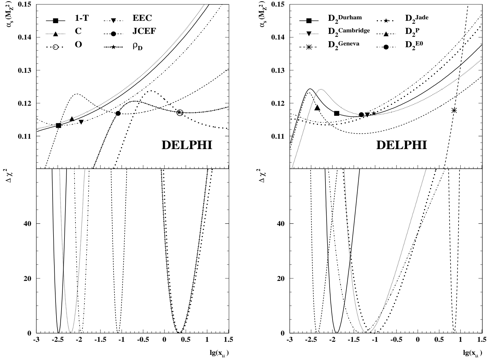
Figure 5: (left side) \alpha_s(M_Z^2) and \Delta\chi^2 = \chi^2 - \chi_{\min}^2 from \mathcal{O}(\alpha_s^2) fits to the double differential distributions in \cos\vartheta_T and 1 - T , C, O, EEC, JCEF, \rho_D . Additionally, the \chi^2 minima are indicated in the \alpha_s(M_Z^2) curves. (right side) The same for the double differential distributions in \cos\vartheta_T and the differential 2-jet rate applying the Durham, Cambridge, Geneva, Jade, P and E0 jet algorithm.
