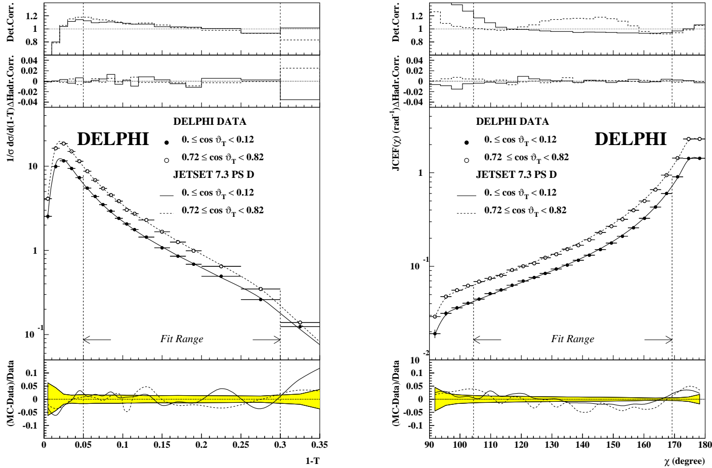
Figure 2: left part: Measured 1-T distribution in two bins of \cos \vartheta_T . The upper part shows the detector corrections in the two \cos \vartheta_T bins. The part below shows the size of the relative hadronization correction in the two \cos \vartheta_T bins with respect to the average correction. In the central part the measured 1-T distributions are compared to JETSET 7.3 PS D. The lower part shows the ratio (Monte Carlo simulation-data)/data for the two \cos \vartheta_T bins. right part: Same curves as shown in the left part but for JCEF in two bins of \cos \vartheta_T .
