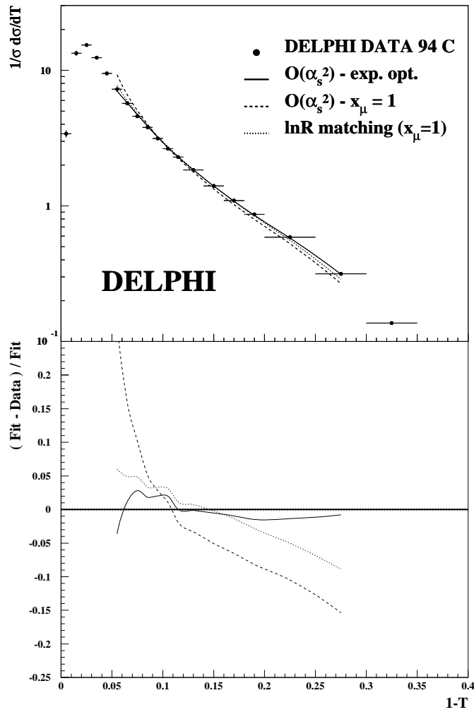
Figure 13: left part: Comparison of DELPHI data with three different QCD Fits: i ) \mathcal{O}(\alpha_s^2) using an experimentally optimized renormalization scale, ii ) \mathcal{O}(\alpha_s^2) using a fixed renormalization scale x_\mu = 1 and iii ) \ln R matched NLLA ( x_\mu = 1 ) for the thrust Distribution. The lower part shows the relative difference (\text{Fit} - \text{Data}) / \text{Fit} . Whereas the \mathcal{O}(\alpha_s^2) curve describes the data over the whole fit range, the slope of the curves for the fixed scale and \ln R matching show a similar systematic distortion with respect to the data. right part: The same for the C-Parameter. Here the distortion is even stronger.
