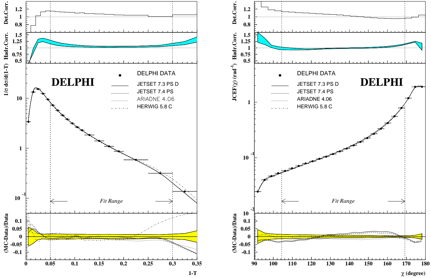
Figure 1: left part : Measured 1-T distribution integrated over \cos\vartheta_T . The upper part shows the detector correction including effects due to initial state radiation. The part below shows the size of the hadronization correction. The width of the band indicates the uncertainty of the correction. In the central part the measured 1-T distribution is compared to the expectation from four hadronization generators, JETSET 7.3 PS D with DELPHI modification of heavy particle decays, JETSET 7.4 PS, ARIADNE 4.06 and HERWIG 5.8c. Also shown is the 1-T range used in the QCD fit. The lower part shows the ratio (Monte Carlo simulation-data)/data for the four hadronization generators. The width of the band indicates the size of the experimental errors. right part : Same curves as shown in the left part but for JCEF integrated over \cos\vartheta_T .
