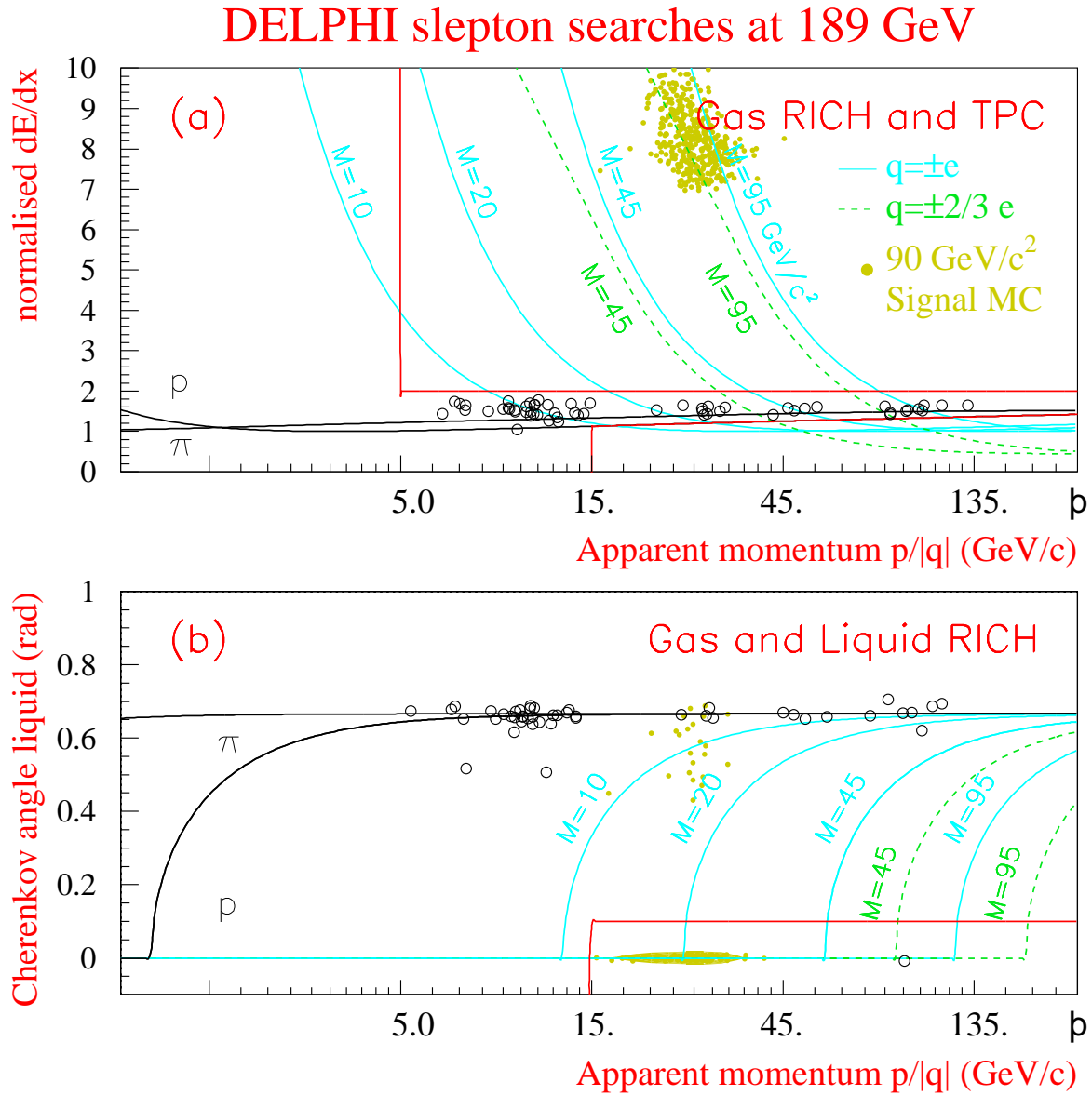
Figure 1: (a) Normalised energy loss as a function of the apparent momentum p/|q| after the Gas Veto for the 189 GeV data. (b) Measured Cherenkov angle in the liquid radiator as a function of the apparent momentum after the Gas Veto: if four photons or less were observed in the liquid radiator, the Cherenkov angle was set equal to zero. The rectangular areas in (a) indicate selections (1)·(2) and (1)·(4), and that in (b) shows selection (1)·(3). The selection criteria are explained in the text. Open circles are data. The small filled circles indicate the expectation for a 90 \text{GeV}/c^2 signal with charge \pm e , resulting in a large dE/dx (upper plot) and no photons (except for a few accidental rings) in the liquid Cherenkov counter (lower plot).
