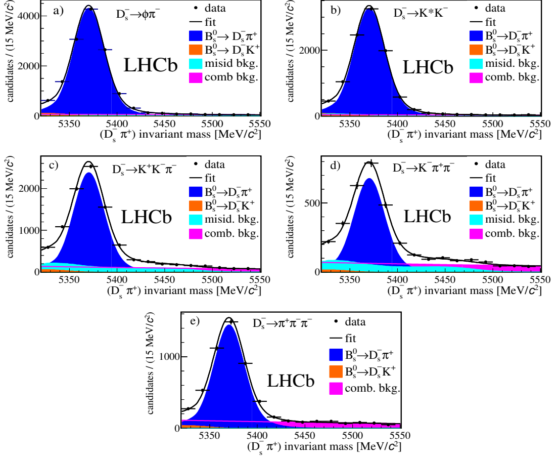
Figure 1: Invariant mass distributions for B_s^0 \rightarrow D_s^- \pi^+ candidates with the D_s^- meson decaying as a) D_s^- \rightarrow \phi(K^+ K^-) \pi^- , b) D_s^- \rightarrow K^{*0}(K^+ \pi^-) K^- , c) D_s^- \rightarrow K^+ K^- \pi^- nonresonant, d) D_s^- \rightarrow K^- \pi^+ \pi^- , and e) D_s^- \rightarrow \pi^- \pi^+ \pi^- . The fits and the various background components are described in the text. Misidentified backgrounds refer to background from B^0 and \Lambda_b^0 decays with one misidentified daughter particle.
