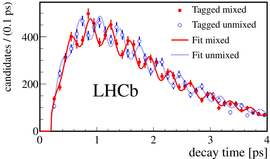
Figure 2: Decay time distribution for the sum of the five decay modes for candidates tagged as mixed (different flavour at decay and production; red, continuous line) or unmixed (same flavour at decay and production; blue, dotted line). The data and the fit projections are plotted in a signal window around the reconstructed B_s^0 mass of 5.32 - 5.55 \text{ GeV}/c^2 .
