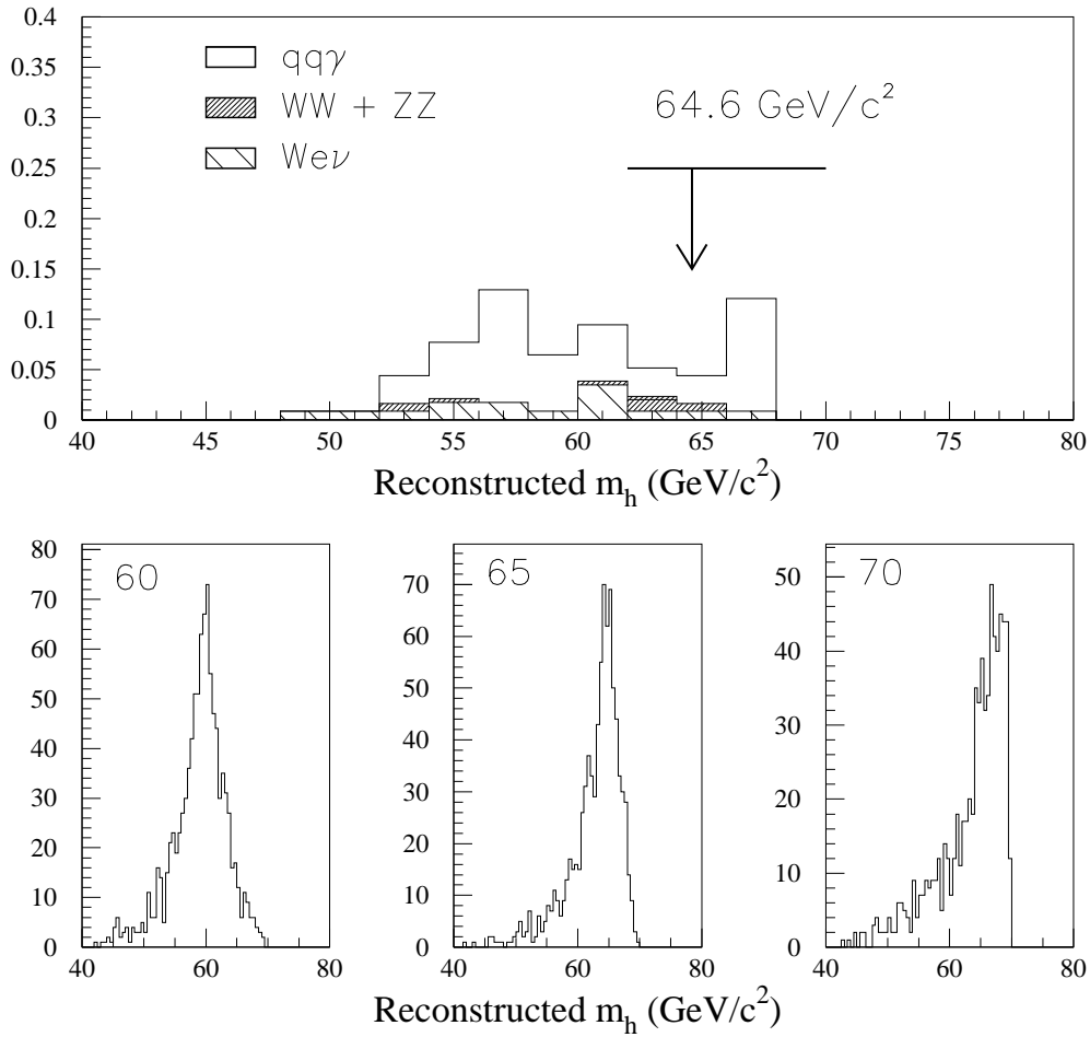
Figure 7: h\nu\bar{\nu} channel: distribution of the reconstructed mass of the Higgs boson at the end of the analysis at \sqrt{s} = 161 \text{ GeV} . The Higgs boson is assumed to recoil against an on-shell Z. The upper plot shows the distribution of the simulated background. The arrow indicates the mass of the selected event and the transverse error bar the uncertainty on the measurement. The bottom plots are the distributions of simulated signal events with masses of 60, 65 and 70 \text{GeV}/c^2 .
