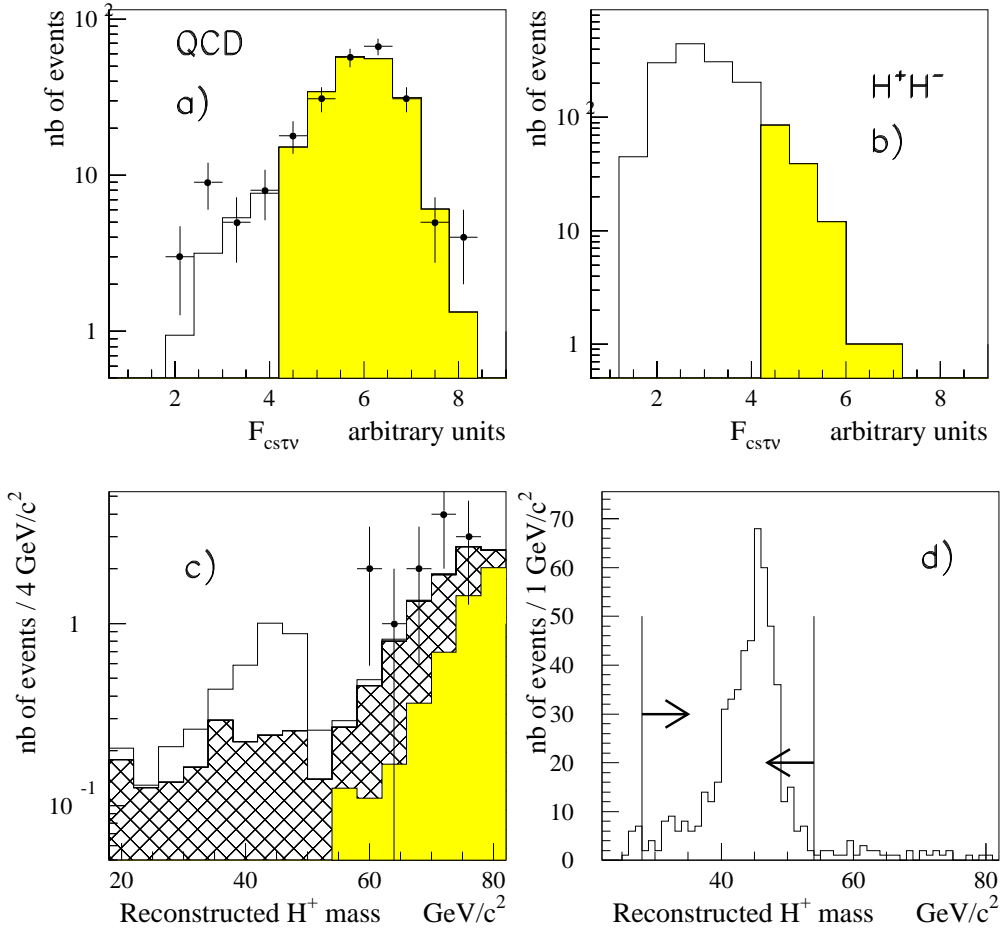
Figure 19: H^+H^- \rightarrow cs\tau\nu_\tau analysis: a) and b): distribution of the multidimensional function F_{cs\tau\nu} after the requirements on the \tau jet (in grey, the events rejected by the selection on F_{cs\tau\nu} ); c) and d): distribution of the reconstructed H^+ mass after the fit. Plots in a) and c) compare data (dots) to background simulation (solid line) normalised to the experimental luminosity. In c) the grey histogram is the WW contamination and the hatched histogram is the q\bar{q}(\gamma) contribution. Also added is the normalised distribution of simulated signal events at 48 \text{ GeV}/c^2 (in white). Plots in b) and d) show unnormalised signal distributions with m_{H^\pm} = 48 and 51 \text{ GeV}/c^2 in b) and m_{H^\pm} = 48 \text{ GeV}/c^2 in d). Arrows in d) indicate the final selection.
