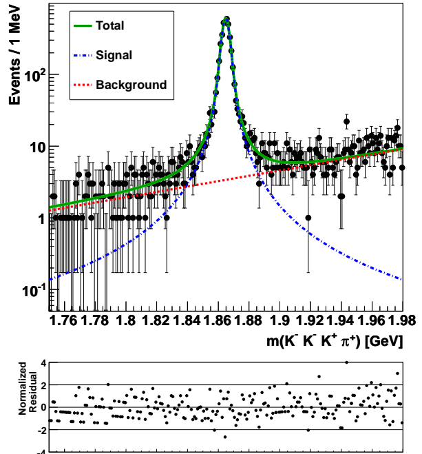
FIG. 1: (color online) Results of the extended, unbinned maximum likelihood fit to the reconstructed D^0 mass distribution. Normalized residuals are defined as (N_o - N_p)/\sqrt{N_p} , where N_o and N_p are observed and predicted numbers of events, respectively.
