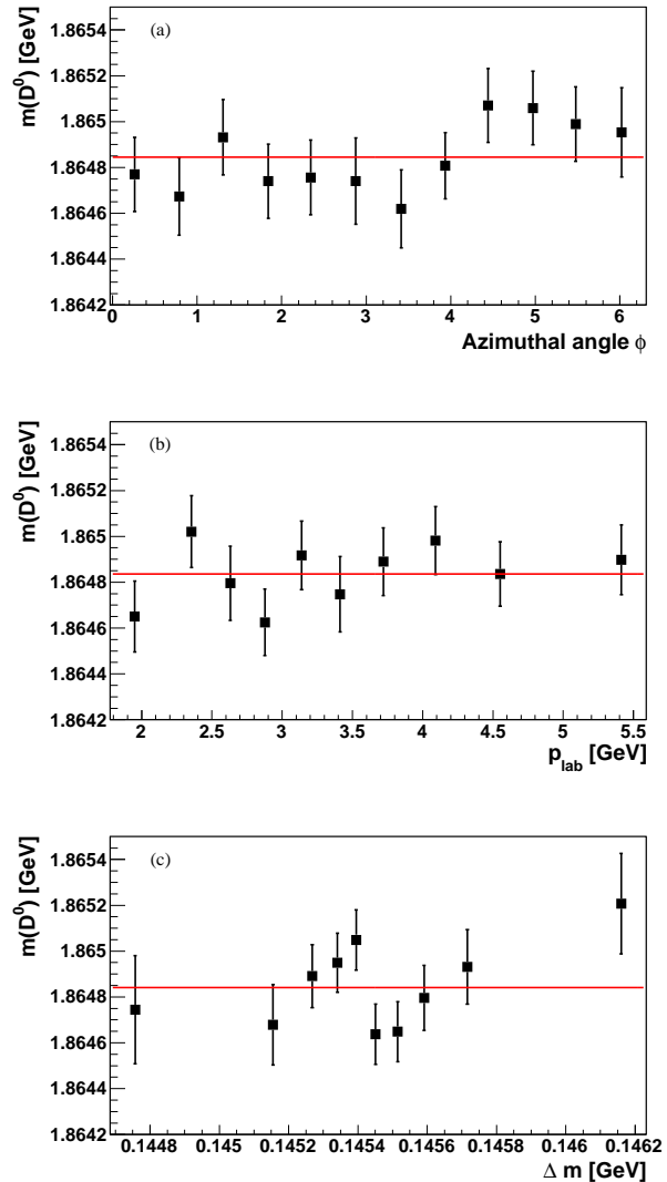
FIG. 2: The value of m(D^0) obtained from fits to data divided into disjoint subsets in (a) \phi , (b) p_{\text{lab}}(D^0) , and (c) \Delta m . Each point represents an individual fit, and the horizontal line indicates the nominal fit result; the points are plotted at the mean value in the range, and the uncertainty in the mean values is smaller than the marker size.
