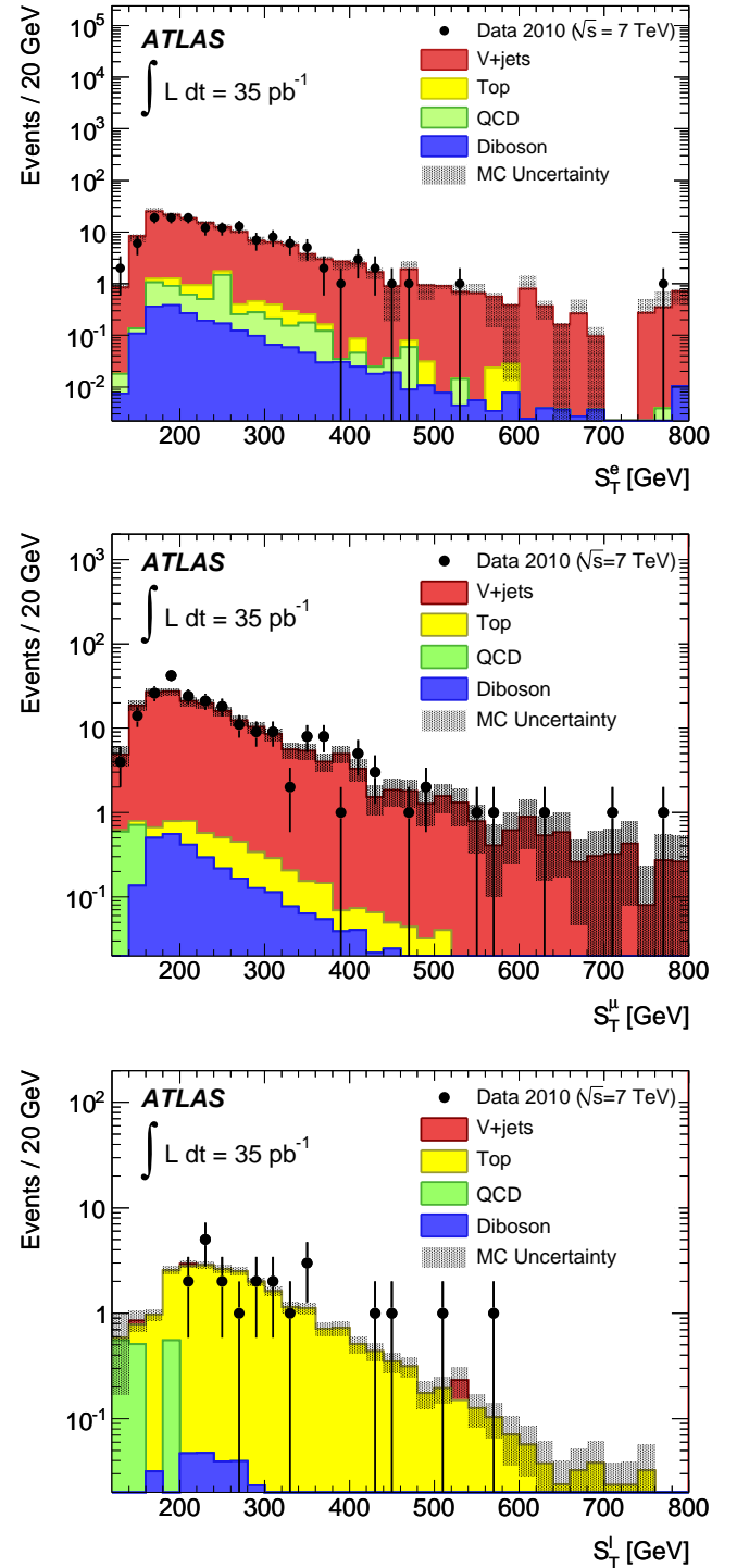
FIG. 1: S_T^\ell distributions for the eejj (top) and the \mu\mu jj final states (middle) in the Z control region. The bottom figure shows the S_T^\ell distribution for the dilepton t\bar{t} control region. The data are indicated by the points and the Standard Model backgrounds are shown with cumulative distributions. The QCD background is estimated from data, while the other background contributions are obtained from simulated samples. The top background includes both t\bar{t} and single top events. The expected contribution from a potential LQ signal is negligible and is not included in the figure. The MC uncertainty band shows the combined statistical and systematic uncertainties on the prediction in each bin.
