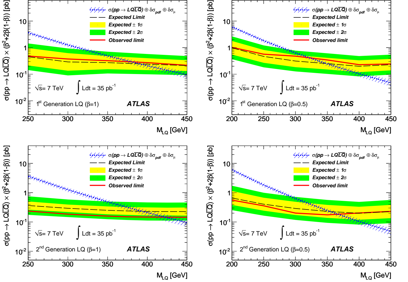
FIG. 5: 95% CL upper bounds on the LQ pair production cross sections as a function of LQ mass for the combination of the eejj and the evjj channels (top), and for the \mu\mu jj and the \mu\nu jj channels (bottom). The figures on the left (right) show the limit for \beta = 1.0 (0.5). The expected limit is indicated by the dashed line. The light yellow (dark green) solid band contains 68% (95%) of possible outcomes from pseudo-experiments in which the yield is Poisson-fluctuated around the background-only expectation. Systematics uncertainties are included. The observed limit is indicated by the solid line. The theory prediction is indicated by the dotted line, which includes systematic uncertainties due to the choice of the PDF and to the renormalization and factorization scales ( \Delta\sigma_\mu ).
