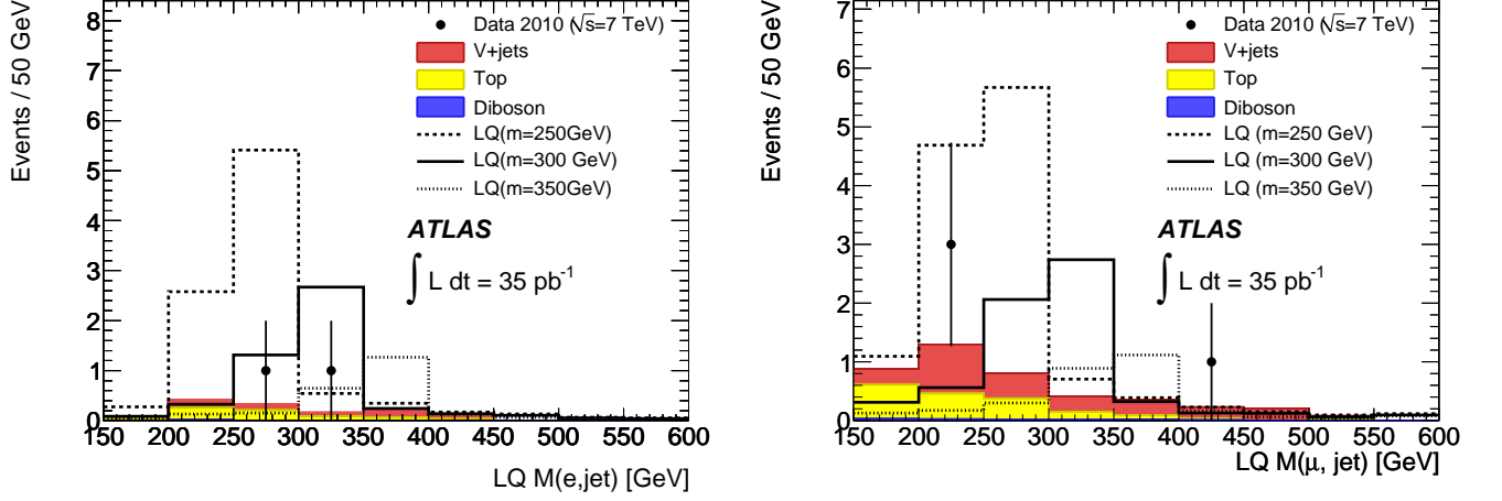
FIG. 4: M_{LQ} distribution for the e\nu jj (left) and the \mu\nu jj final state (right) after all selections. The data are indicated by the points and the Standard Model backgrounds are shown with cumulative distributions. The expected LQ signals for various masses are also shown.
