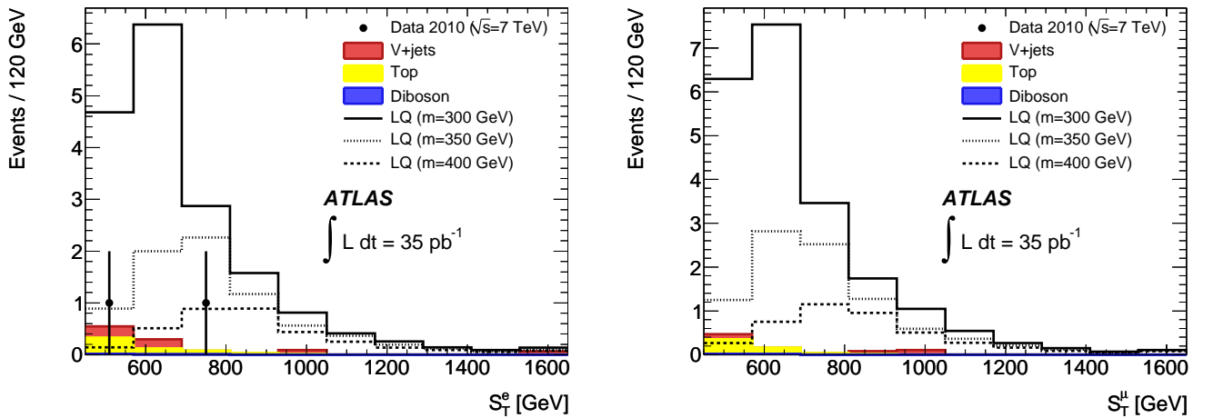
FIG. 3: S_T^e distribution for the eejj (left) and the \mu\mu jj final states (right) after all selections. The data are indicated by the points and the Standard Model backgrounds are shown with cumulative distributions. The expected LQ signals for various masses are also shown.
