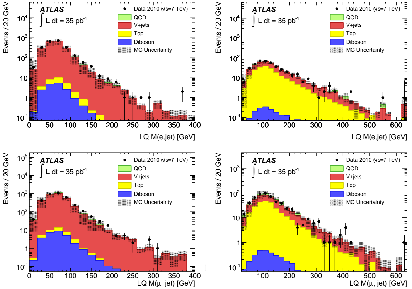
FIG. 2: Reconstructed M_{LQ} distributions for the e\nu jj (top) and the \mu\nu jj (bottom) final states in the W + 2 jets (left) and t\bar{t} (right) control regions. The data are indicated by the points and the Standard Model backgrounds are shown with cumulative distributions. The QCD background is estimated from data, while the other background contributions are obtained from simulated samples. The top background includes both t\bar{t} and single top events. The expected contribution from a potential LQ signal is negligible and is not included in the figure. The MC uncertainty band indicates the combined statistical and systematic uncertainties on the prediction in each bin.
