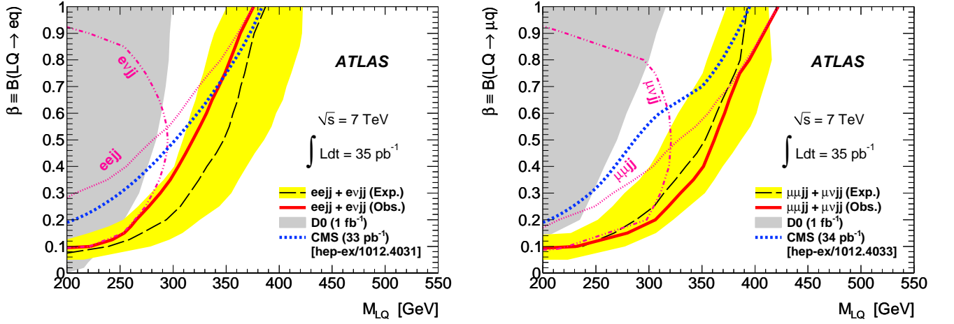
FIG. 6: 95% CL exclusion region obtained from the combination of the two electron channels (left) and the muon channels (right) shown in the \beta versus leptoquark mass plane. The gray area indicates the D0 exclusion limit [9, 10], and the thick dotted line the CMS exclusion [11, 12]. The dotted and dotted-dashed lines show the individual limits for the lljj and the l\nu jj channels, respectively. The combined expected limit is indicated by the thick dashed line. The solid band contains 68% of possible outcomes from pseudo-experiments in which the yield is Poisson-fluctuated around the background-only expectation. Systematic uncertainties are included. The combined observed limit is indicated by the solid line.
