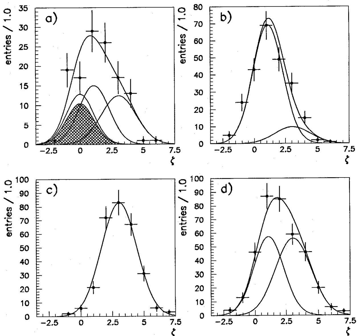
Figure 9: Projection of the data distribution onto the \zeta axis. Points with error bars (data) are compared to the fit represented by the uppermost curve. This curve is the sum of the p , K , \pi contributions, shown with Gaussians centered at \zeta = 0.0, 1.1, 3.05 respectively. The four plots correspond to the four samples used in the fit: a) \mu p sample (the signal content is hatched); b) \mu K sample; c) \mu\pi sample; d) \mu X sample.
