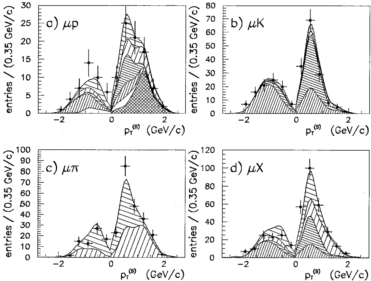
Figure 8: Projection of the data distribution onto the p_T^{(s)} axis (where p_T^{(s)} is signed transverse momentum of the muon. Its positive values correspond to the right sign combination (muon and hadron have opposite charges), whereas negative values to the wrong sign one (same sign \mu -hadron pairs). Points with error bars (data) are compared to the fit (uppermost curve) decomposed into six classes shown with different hatching. The four plots shown correspond to the four samples used in the fit.
