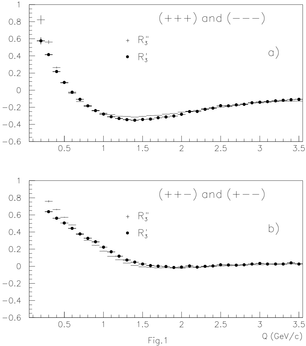
Figure 1: Q -dependence of R''_3 , the total three-particle correlation, and R'_3 , the three-particle correlation arising from two-body correlations, (a) for like-sign and (b) for unlike-sign triplets.
