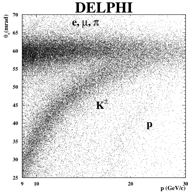
Figure 2: Mean Cherenkov angle versus particle momentum.
