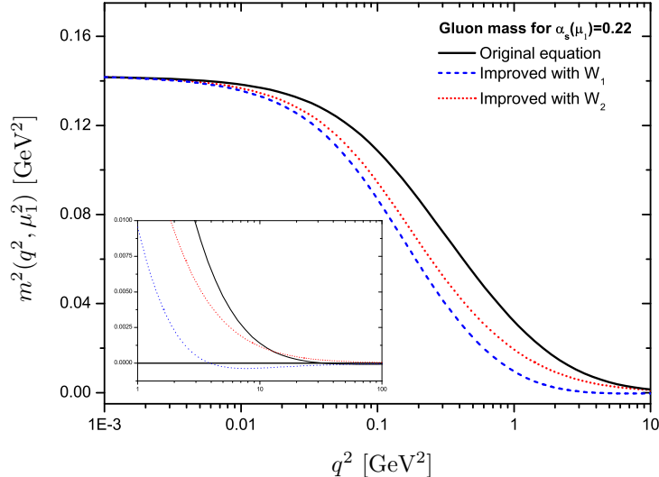
FIG. 10: (color online) Comparison of the numerical results obtained for m^2(q^2, \mu_1^2) using the original gluon mass equation (black continuous); the improved versions with W_1 of Eq. (6.6)(blue dashed) and W_2 of Eq. (6.7) (red dotted). The inset shows a zoom in the UV tail of the same quantities.
