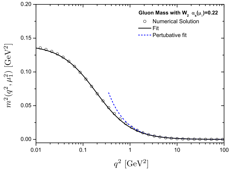
FIG. 11: (color online) The numerical solution for m^2(q^2) obtained using the RG-improved Ansatz W_2 of Eq. (6.7) (black circles). The (black) continuous curve represents the fit of Eq. (6.9) while the (blue) dashed curve is the asymptotic fit for the ultraviolet tail given by Eq. (6.10).
