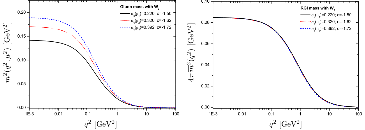
FIG. 9: (color online) The numerical solution for m^2(q^2, \mu^2) (left panel) using the model of Eq. (6.7) for the three renormalization scale \mu_i ; the corresponding RGI mass 4\pi\bar{m}^2(q^2) given by Eq. (2.30) is shown on the right panel.
