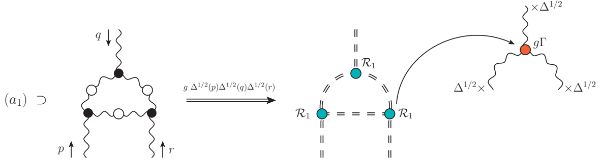
FIG. 4: Schematic representation of the conversion of a typical diagram into its RGI equivalent.
