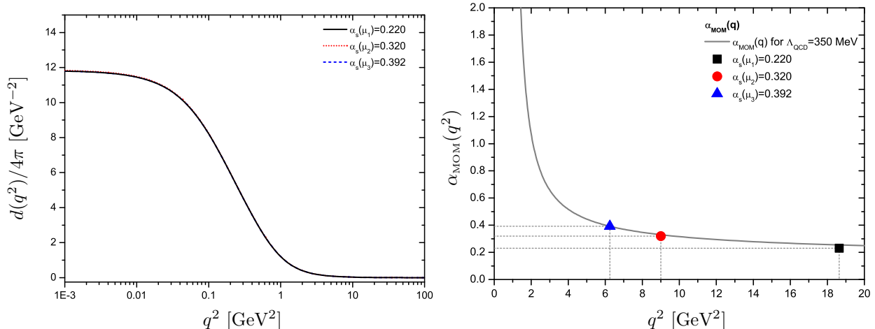
FIG. 6: (color online) Left panel: The RGI combination d(q^2)/4\pi obtained using Eq. (2.29) for the three renormalization points \mu_i chosen. Right panel: The running coupling in the MOM scheme, \alpha_{\text{MOM}}(q) [73] for \Lambda_{\text{QCD}} = 350 MeV and N_f = 0 . Each point represent the values used for \alpha_s(\mu_i) in our calculations.
