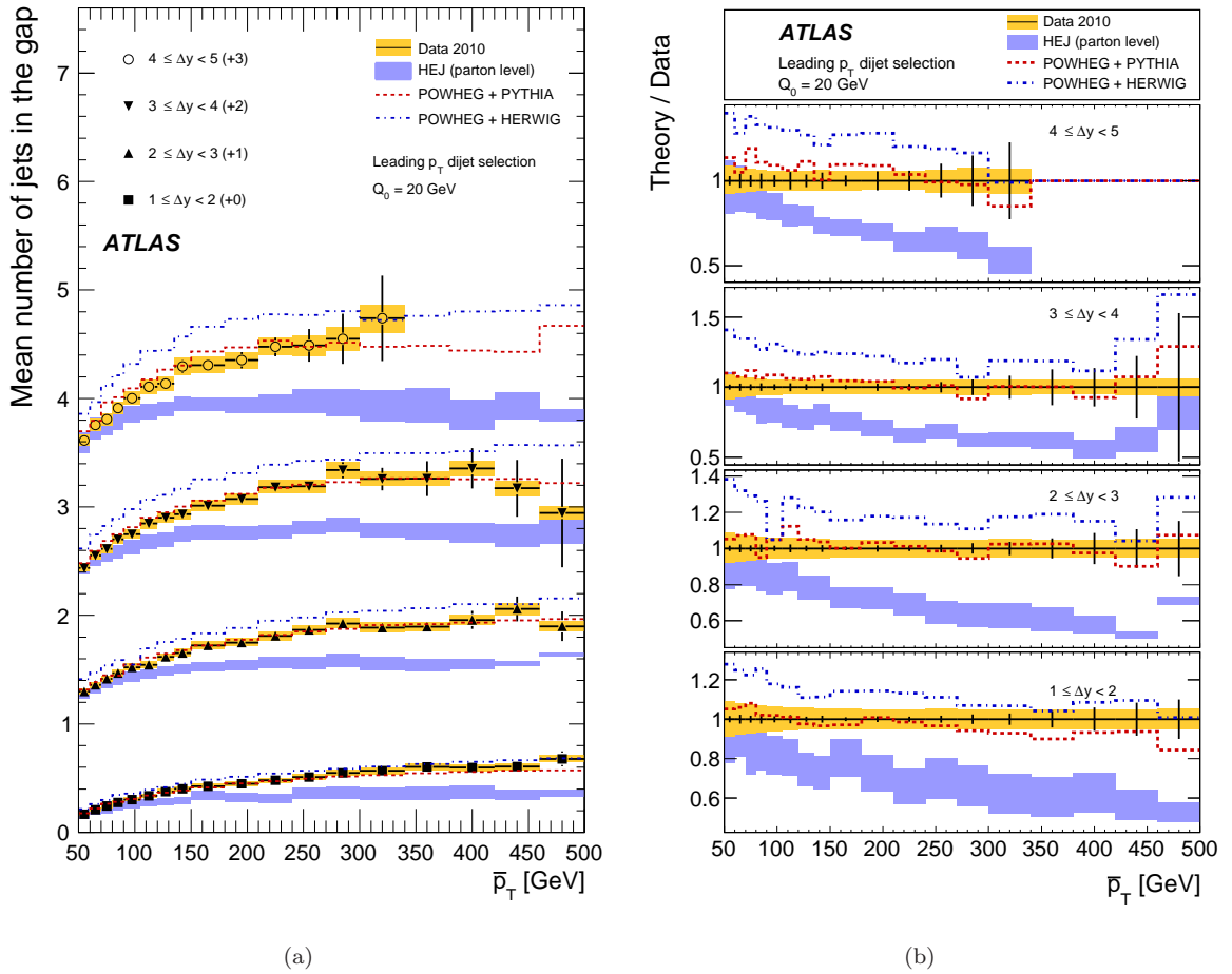
Figure 6. Mean number of jets in the gap as a function of \bar{p}_T for various \Delta y slices. The dijet system is defined as the two leading- p_T jets in the event. The data are compared to the HEJ and POWHEG predictions in (a). The ratio of these theory predictions to the data are shown in (b). The data and theory are presented in the same way as Fig. 3.
