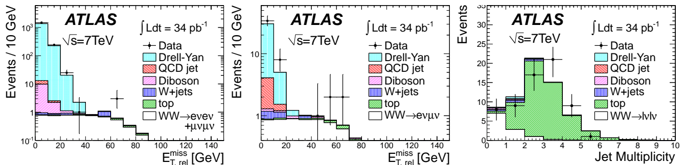
FIG. 1. E_{T,\text{rel}}^{\text{miss}} distributions for the selected ee and \mu\mu (left) and e\mu (center) events and the multiplicity distribution for jets with p_T > 20 GeV and |\eta| < 3.0 for all three dilepton channels combined (right). The distributions show events with all selection criteria applied except for E_{T,\text{rel}}^{\text{miss}} in the E_{T,\text{rel}}^{\text{miss}} distribution and the jet veto in the jet multiplicity distribution. Simulation is used for the QCD jet and W +jets background contributions in these plots as opposed to the data-driven method used for W +jets in the signal region described in the text. The QCD jet contribution is negligible in the signal region.
