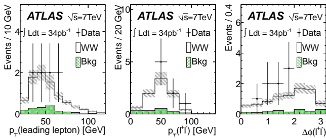
FIG. 2. Distributions of the leading lepton p_T (left), transverse momentum of the dilepton system (center), and azimuthal angle between the leptons (right) for the sum of the selected ee , \mu\mu and e\mu samples compared to the expectation. The gray band indicates the combined statistical and systematic uncertainty on the sum of the signal and background expectations.
