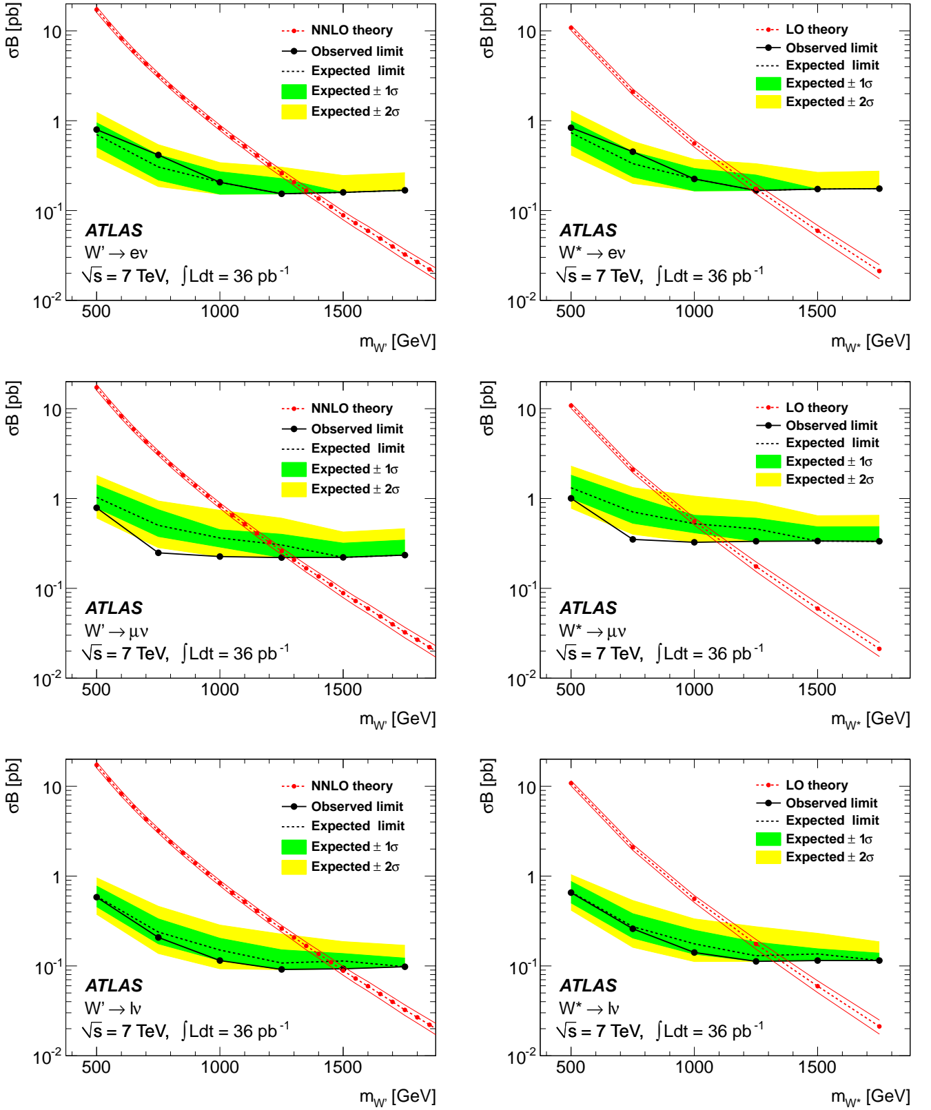
Figure 4: Limits at 95% CL for W' (left) and W^* (right) production in the decay channels W'/W^* \rightarrow e\nu (top), W'/W^* \rightarrow \mu\nu (center), and the combination of these (bottom). The solid lines show the observed limits with all uncertainties. The expected limit is indicated with dashed lines surrounded by 1\sigma and 2\sigma shaded bands. Dashed lines show the theory predictions (NNLO for W' , LO for W^* ) between solid lines indicating their uncertainties. The W' \sigma_B uncertainties are obtained by varying renormalization and factorization scales and by varying PDFs. Only the latter are included for W^* .
