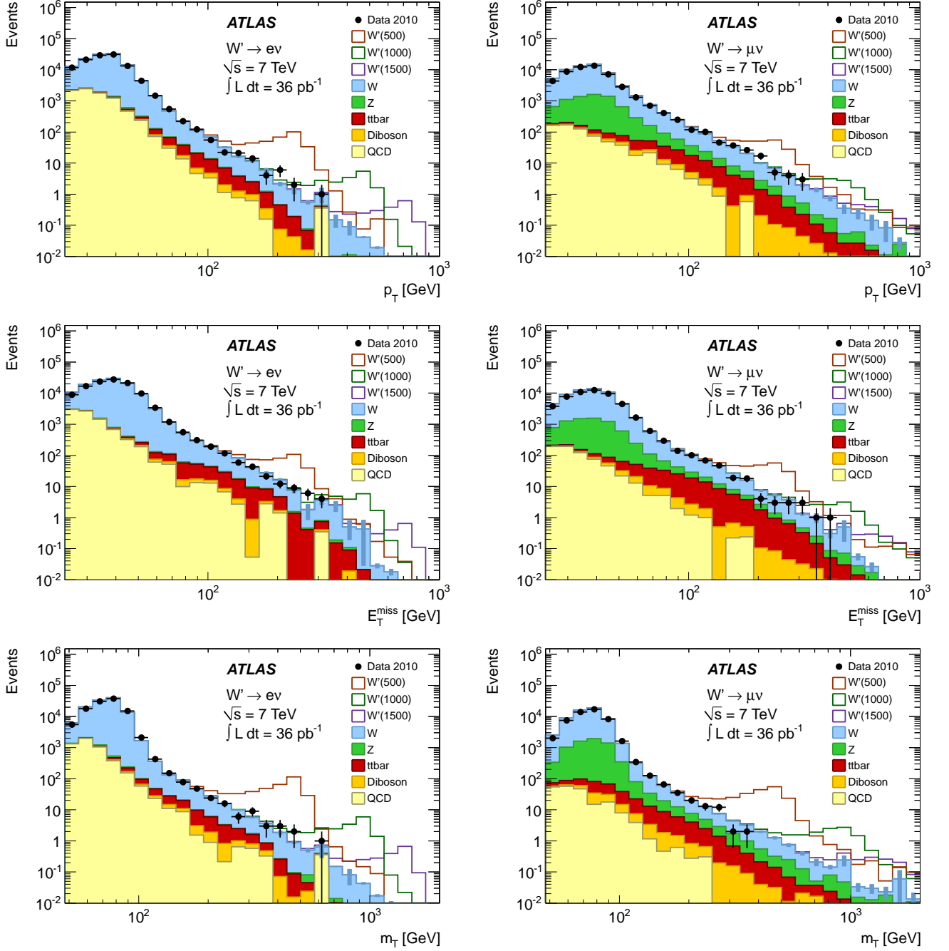
Figure 1: Spectra of p_T (top), missing E_T (center) and m_T (bottom) for the electron (left) and muon (right) channels after final event selection. The points represent ATLAS data and the filled histograms show the stacked backgrounds. Both direct production of leptons and indirect from \tau -leptons are included. Open histograms are W' signals added to the background with masses in GeV indicated in parentheses in the legend. The QCD background is estimated from data. The signal and other background samples are normalized using the integrated luminosity of the data and the NNLO (near-NNLO for t\bar{t} ) cross sections listed in Table 1.
