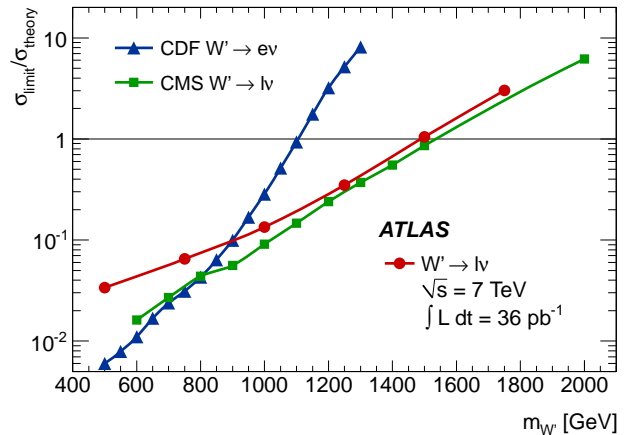
Figure 5: Normalized cross section limits ( \sigma_{\text{limit}}/\sigma_{\text{theory}} ) for W' as a function of mass for this measurement and those from CDF and CMS. The cross section calculations assume the W' has the same couplings as the standard model W boson. The region above each curve is excluded at 95% CL.
