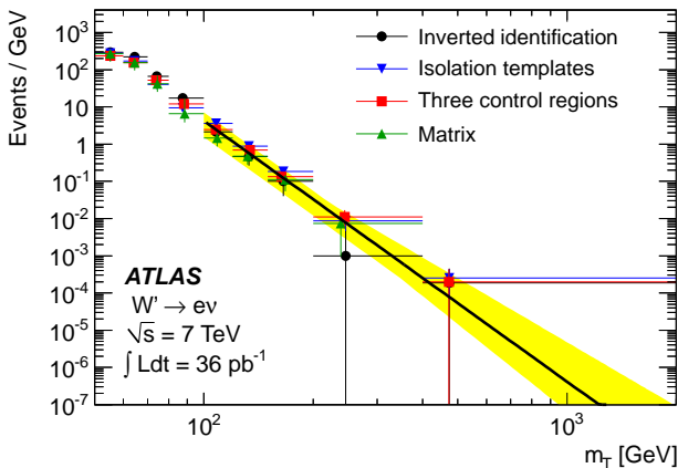
Figure 2: Estimated QCD background as a function of m_T in the electron channel after final selection as obtained from the four data-driven methods (see text). The power-law fit to all four sets of results and its 1\sigma uncertainty band are also shown.
