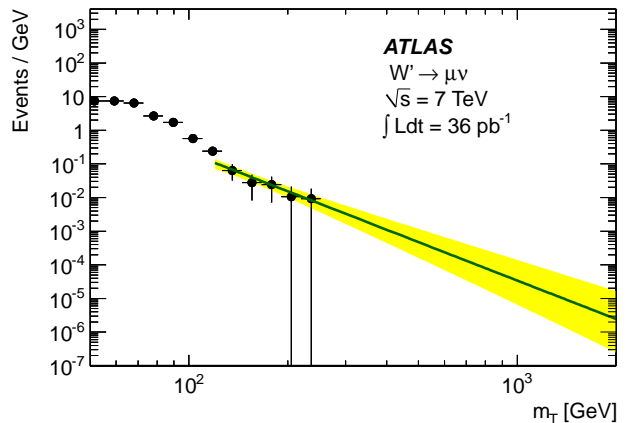
Figure 3: Estimated QCD background as a function of m_T in the muon channel after final selection as obtained from the data-driven method (see text). The unbinned power-law fit to the data and its 1\sigma uncertainty band are also shown.
