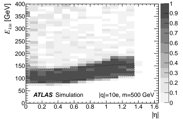
Figure 5: Probability to pass all selection criteria as a function of pseudorapidity and kinetic energy at origin, for a HIP with charge 10e and mass 500 GeV. The dark region corresponds to the kinetic range where the particle stops in or near the second layer of the EM calorimeter barrel and is parametrised with three energy values (dashed parallelogram, see Table 1).
