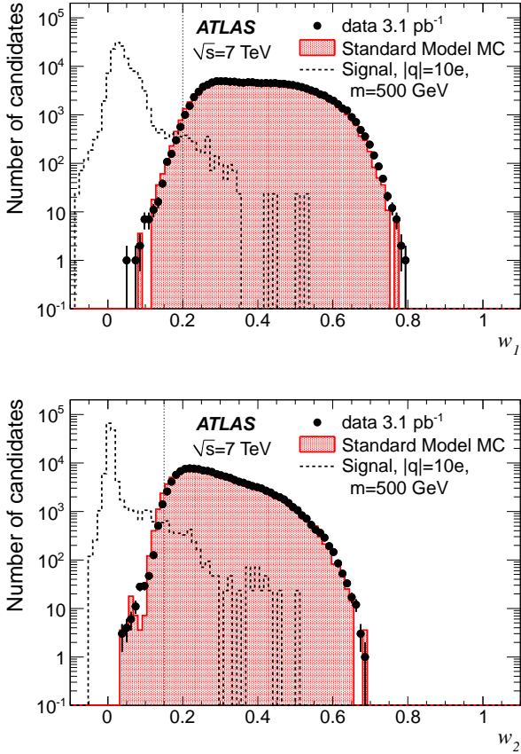
Figure 3: Distributions of w_1 and w_2 following the loose selection. Data (dots) are compared with area-normalised signal ( |q| = 10e and m = 500 GeV, dashed lines) and Standard Model background (shaded area) simulations. Negative values are caused by pedestal fluctuations. Dotted lines show the selection cut values.
