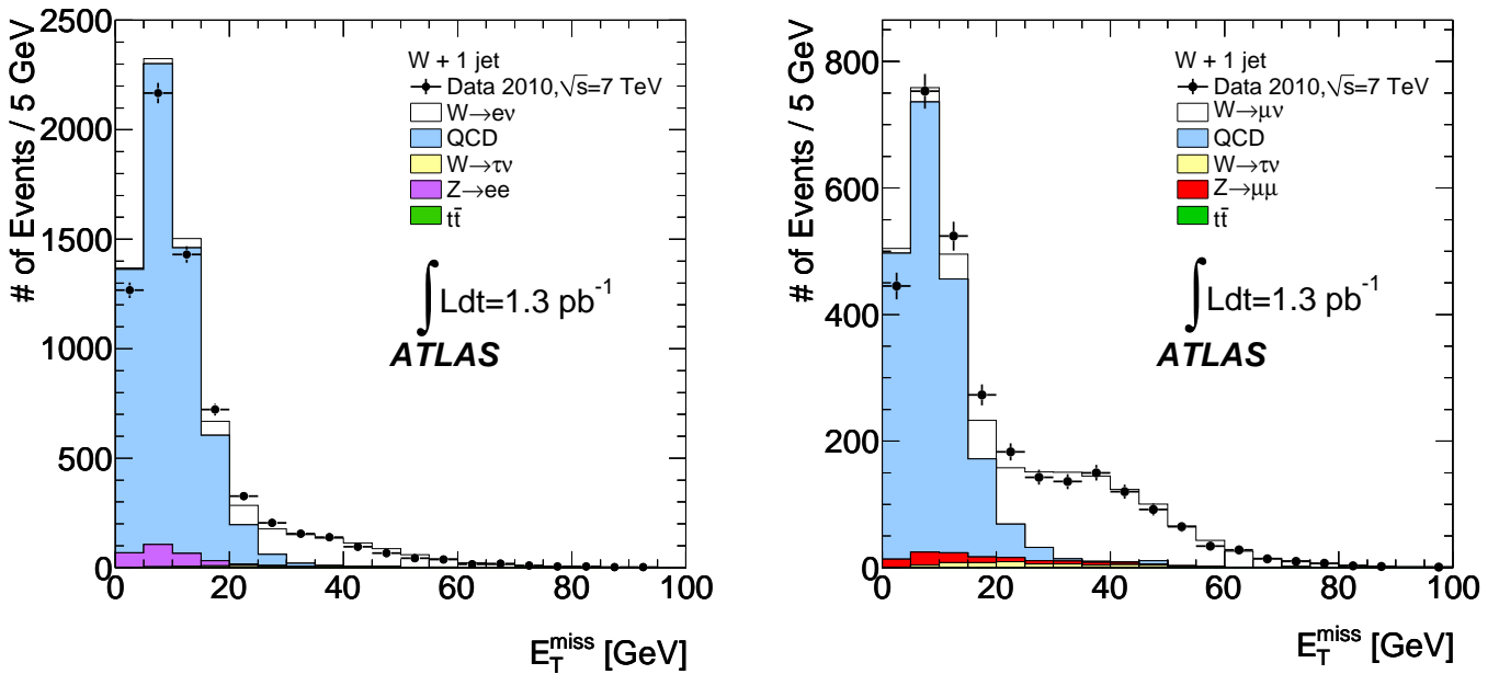
Figure 1: Results of fitting the signal and background templates to the E_T^{\text{miss}} distribution in the electron (left) and muon (right) channels for the 1-jet bin. In the electron channel, the fit was performed for E_T^{\text{miss}} > 10 GeV. All templates were from simulated events, except for the QCD background template in the electron channel which was obtained from the data.
