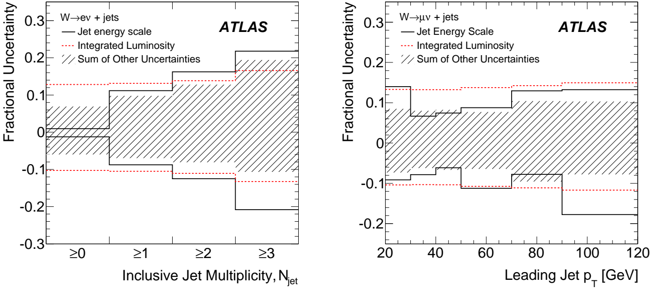
Figure 2: Summary of the systematic uncertainties on the cross section measurement shown as a function of jet multiplicity in the electron channel (left) and leading-jet p_T in the muon channel (right). The jet energy scale uncertainty includes the uncertainty on E_T^{\text{miss}} . The main contribution to the “sum of other uncertainties” in the electron channel comes from the QCD background (especially at high jet multiplicities), the electron identification efficiency and the electron energy scale. For the muon channel, the main contribution is from the muon reconstruction efficiency.
