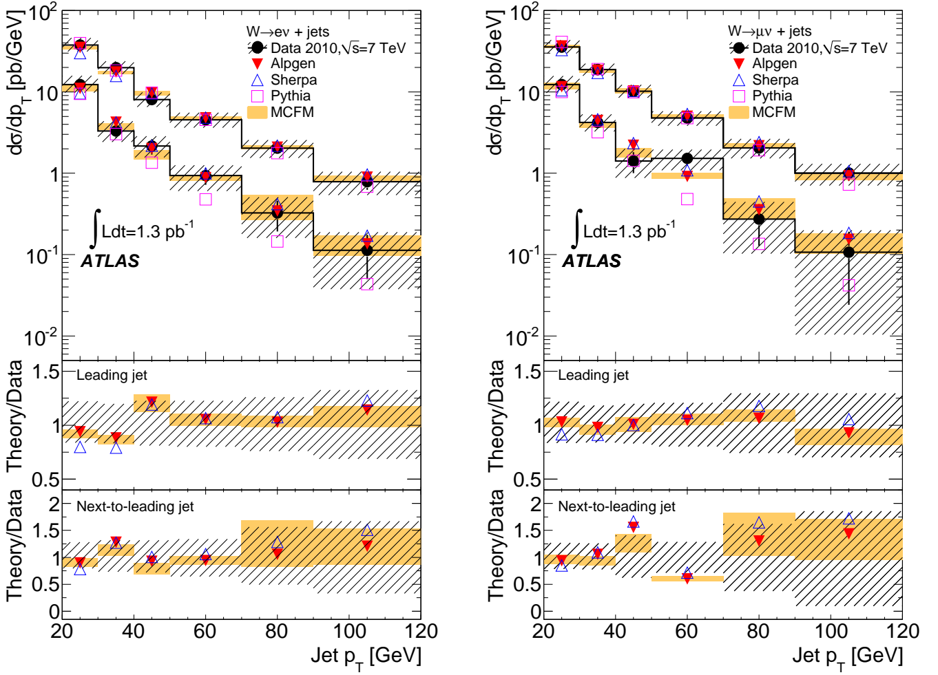
Figure 5: W +jets cross-section as a function of the p_T of the two leading jets in the event. The p_T of the leading jet is shown for events with \geq 1 jet while the p_T of the next-to-leading jet is shown for events with \geq 2 jets. Left: electron channel. Right: muon channel. The cross sections are quoted in a limited and well-defined kinematic region, described in the text. For the data, the statistical uncertainties are shown by the vertical bars, and the combined statistical and systematic uncertainties are shown by the hashed regions. Also shown are theoretical predictions from PYTHIA, ALPGEN, SHERPA and MCFM, and the ratio of theoretical predictions to data (PYTHIA is not shown in the ratio). The theoretical uncertainties are shown only for MCFM, which provides NLO predictions for N_{\text{jet}} \leq 2 and a LO prediction for N_{\text{jet}} = 3 .
