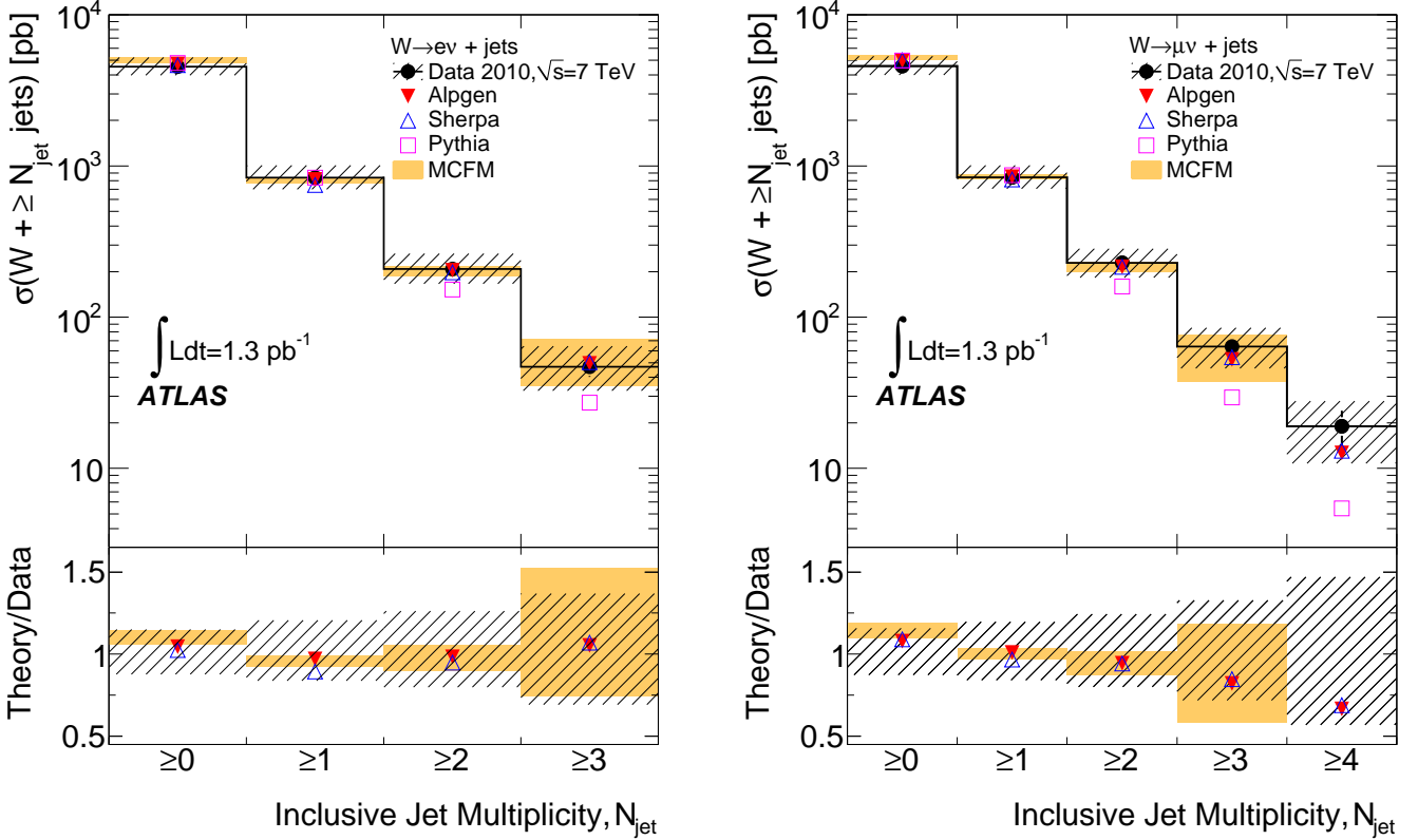
Figure 3: W +jets cross-section results as a function of corrected jet multiplicity. Left: electron channel. Right: muon channel. The cross sections are quoted in a limited and well-defined kinematic region, described in the text. For the data, the statistical uncertainties are shown by the vertical bars, and the combined statistical and systematic uncertainties are shown by the hashed regions. Note that the uncertainties are correlated from bin to bin. Also shown are predictions from PYTHIA, ALPGEN, SHERPA and MCFM, and the ratio of theoretical predictions to data (PYTHIA is not shown in the ratio). The theoretical uncertainties are shown only for MCFM, which provides NLO predictions for N_{\text{jet}} \leq 2 and a LO prediction for N_{\text{jet}} = 3 .
