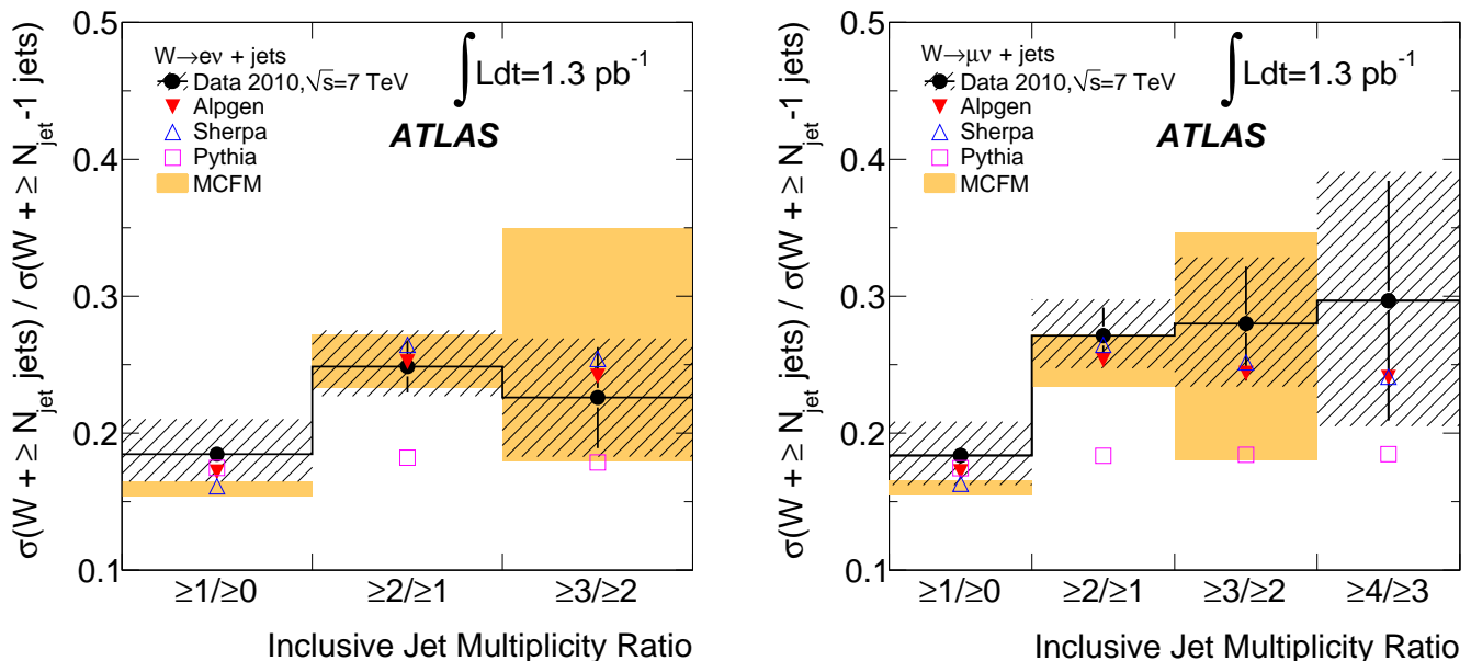
Figure 4: W +jets cross-section ratio results as a function of corrected jet multiplicity. Left: electron channel. Right: muon channel. The cross sections are quoted in a limited and well-defined kinematic region, described in the text. For the data, the statistical uncertainties are shown by the vertical bars, and the combined statistical and systematic uncertainties are shown by the hashed regions. Also shown are theoretical predictions from PYTHIA, ALPGEN, SHERPA, and MCFM. The theoretical uncertainties are shown only for MCFM, which provides NLO predictions for N_{\text{jet}} \leq 2 and a LO prediction for N_{\text{jet}} = 3 .
