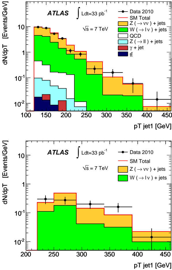
Figure 4: Measured leading-jet p_T distributions for the LowPt (top) and HighPt (bottom) analyses compared to background predictions. Only statistical uncertainties on the data are shown. The systematic uncertainties on the total number of predicted events are 9% for the LowPt region and 12% for the HighPt region.
