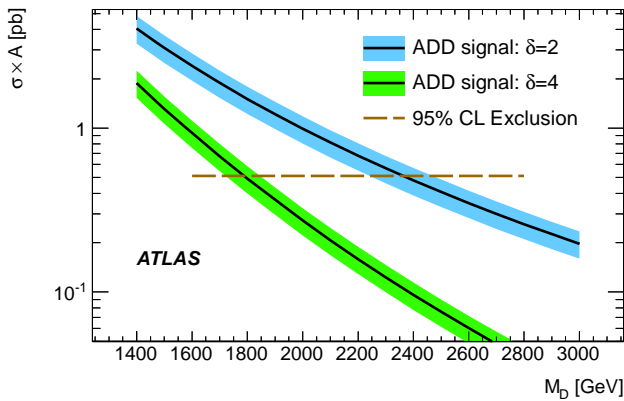
Figure 5: Left: Signal cross section times acceptance as a function of M_D predicted by the effective ADD theory for 2 and 4 extra dimensions. The bands surrounding the curves reflect the systematic uncertainties. The observed limit is shown as a dashed line. Right: 95% CL observed lower limits on M_D for different numbers of extra dimensions for ATLAS, CDF [36], and LEP [37, 38, 39, 40, 41].
