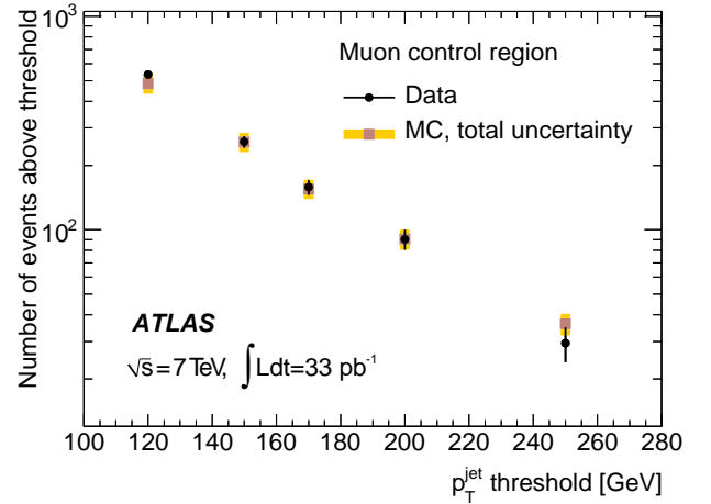
Figure 1: Observed number of events (black circles) in the muon control sample compared to the sum of the different W/Z plus jets predictions (squares) as a function of the highest jet p_T threshold, in events with no second-leading jet with p_T > 60 GeV. The band indicates the total systematic uncertainty on the MC prediction.
