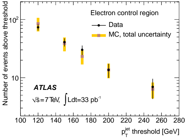
Figure 2: Observed number of events (black circles) in the electron control sample compared to the sum of the different W/Z plus jets predictions (squares) as a function of the highest jet p_T threshold, in events with no second-leading jet with p_T > 60 \text{ GeV} . The band indicates the total uncertainty on the MC prediction.
