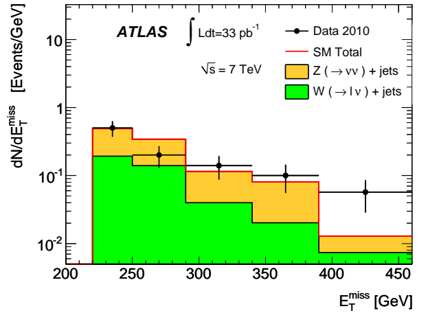
Figure 3: Measured E_T^{\text{miss}} distributions for the LowPt (top) and HighPt (bottom) analyses compared to background predictions. Only statistical uncertainties on the data are shown. The systematic uncertainties on the total number of predicted events are 9% for the LowPt region and 12% for the HighPt region.
