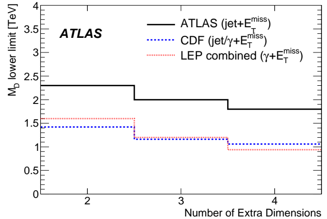
Figure 5: Left: Signal cross section times acceptance as a function of M_D predicted by the effective ADD theory for 2 and 4 extra dimensions. The bands surrounding the curves reflect the systematic uncertainties. The observed limit is shown as a dashed line. Right: 95% CL observed lower limits on M_D for different numbers of extra dimensions for ATLAS, CDF [36], and LEP [37, 38, 39, 40, 41].
