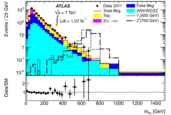
Fig. 1. Observed and predicted e\mu invariant mass distributions. Signal simulations are shown for m_{\tilde{\nu}_\tau} = 650 \text{ GeV} and m_{Z'} = 700 \text{ GeV} . The couplings \lambda'_{311} = 0.10 and \lambda_{312} = 0.05 are used for the RPV \tilde{\nu}_\tau model. The production cross section is assumed to be the current published limit of 0.178 \text{ pb} for the LFV Z' model [8]. The ratio plot at the bottom includes only statistical uncertainties.
