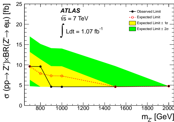
Fig. 3. The observed 95% C.L. upper limits on \sigma(pp \rightarrow Z') \times \text{BR}(Z' \rightarrow e\mu) . The expected limits are also shown together with the expected \pm 1 and \pm 2 standard deviation uncertainty bands. The observed and expected limits overlap as discussed in the text.
