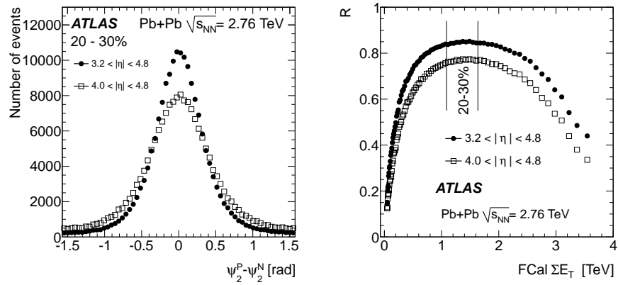
Figure 3: (left) Distribution of the difference between the event planes at positive and negative \eta obtained using Layer 1 FCal towers, both with full and half acceptance. (right) FCal \Sigma E_T dependence of the resolution correction for event planes from Layer 1 FCal towers in full acceptance (full symbols) and half acceptance (open symbols).
