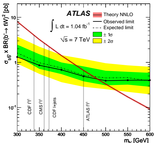
FIG. 5: Expected and observed cross section exclusion upper limits at 95% C.L. for a fourth-generation b' quark. Systematic uncertainties on the expected limit are shown with shaded bands. Previously published limits from CDF [3, 4], CMS [5], and ATLAS [7] are also shown.
