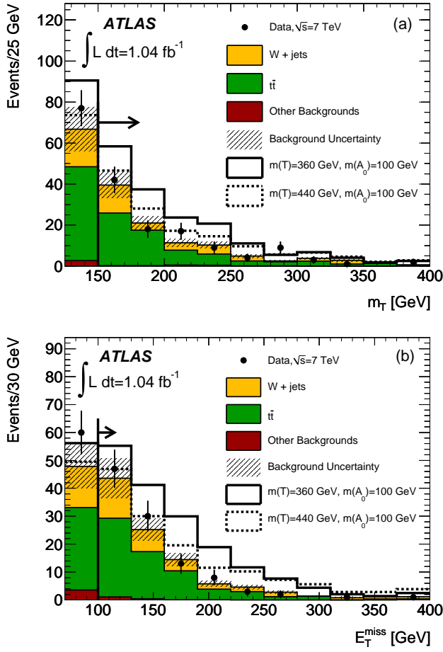
FIG. 1: (a) Transverse mass of the lepton and missing energy and (b) E_T^{\text{miss}} after applying all selection criteria except the cut on the variable shown. MC background contributions are stacked on top of each other and normalized according to the data-driven corrections discussed in the text. The lines with the arrows indicate the selection criteria that define the signal region ( m_T > 150 GeV and E_T^{\text{miss}} > 100 GeV). ‘Other Backgrounds’ includes both multi-jet backgrounds and Z +jets, single top and diboson production. Expectations from two signal mass points are stacked separately on top of the SM background. The last bin includes the overflow.
