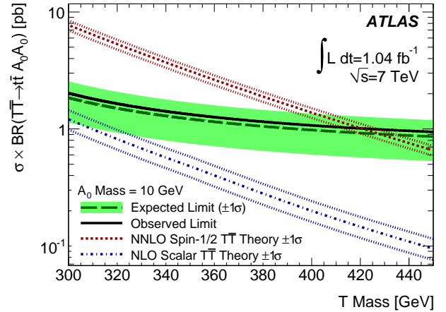
FIG. 3: Cross-section times branching ratio excluded at the 95% confidence level versus T mass for an A_0 mass of 10 GeV. Theoretical predictions for both spin- \frac{1}{2} and scalar T pair production are also shown.
