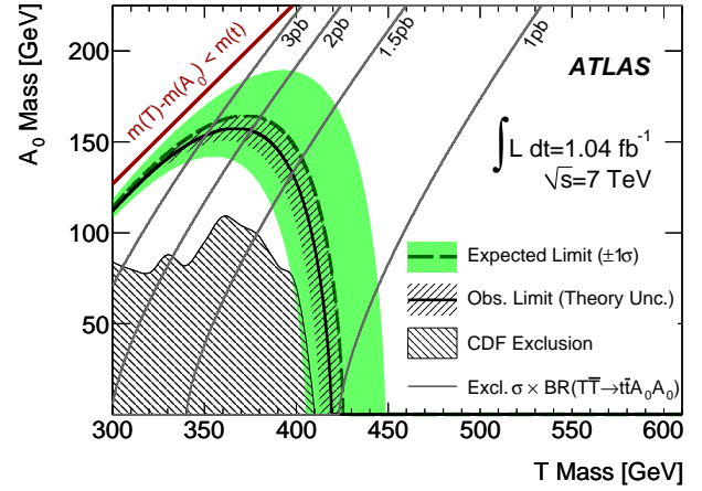
FIG. 2: Excluded region (under the curve) at the 95% confidence level as a function of T and A_0 masses, compared with the CDF exclusion [10, 11]. Theoretical uncertainties on the T\bar{T} cross-section are not included in the limit, but the effect of these uncertainties is shown. The gray contours show the excluded cross-section times branching ratio as a function of the two masses.
