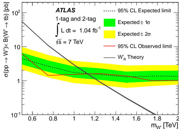
FIG. 2: 95% CL limit on the cross section, \sigma(pp \rightarrow W'_R) \times \text{BR}(W'_R \rightarrow tb) , times branching ratio for W'_R \rightarrow tb as a function of the W'_R boson mass. The theory curve is also shown.
