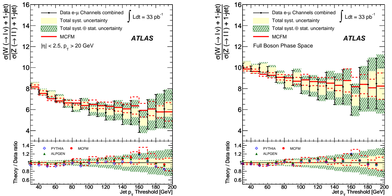
Figure 4: Left: Combined electron and muon results for R_{\text{jet}} in a common fiducial region. The results are compared to predictions from MCFM (corrected to particle level). Data are shown with black error bars indicating the statistical uncertainties. The yellow band shows all systematic uncertainties added in quadrature and the green band shows statistical and systematic uncertainties added in quadrature. The theory uncertainty (dashed line) includes contributions from PDF and renormalisation and factorisation scales. Right: Combined electron and muon results for R_{\text{jet}} extrapolated to the total phase space. Note that these threshold data and their associated uncertainties are correlated between bins.
