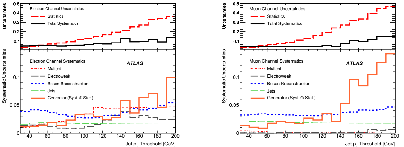
Figure 2: Relative systematic uncertainties on R_{\text{jet}} in the electron channel (left) and in the muon channel (right). The top plot displays the total systematic and statistics uncertainty (shown as red dashed line) versus jet p_{\text{T}} threshold. The lower plot shows the breakdown of the systematic uncertainties. Boson reconstruction contains the uncertainties related with the leptons and E_{\text{T}}^{\text{miss}} (including trigger and lepton identification). Jets contains systematics of the jet correction as well as the jet energy scale and resolution. Uncertainties from each group were added in quadrature.
