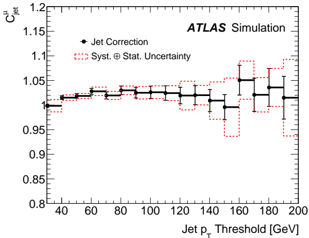
Figure 1: Detector jet spectrum correction ( C_{\text{jet}}^{\mu} ) on R_{\text{jet}} in the muon channel derived from ALPGEN. The uncertainty is shown as a dashed red line, it accounts for the difference between PYTHIA and ALPGEN generators.
