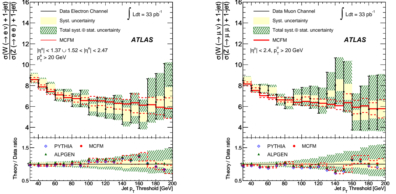
Figure 3: Results for R_{\text{jet}} in the electron channel (left) and in the muon channel (right) for their respective fiducial regions. The results are compared to NLO predictions from MCFM (corrected to particle level using PYTHIA). Data are shown as black points at the lower bin edge corresponding to the jet p_T threshold with black error bars indicating the statistical uncertainties. The yellow band shows all systematic uncertainties added in quadrature and the green band shows statistical and systematic uncertainties added in quadrature. The theory uncertainty (dashed line) shown on the MCFM prediction includes uncertainties from PDF and renormalisation and factorisation scales. Note that these threshold data and their associated uncertainties are correlated between bins.
