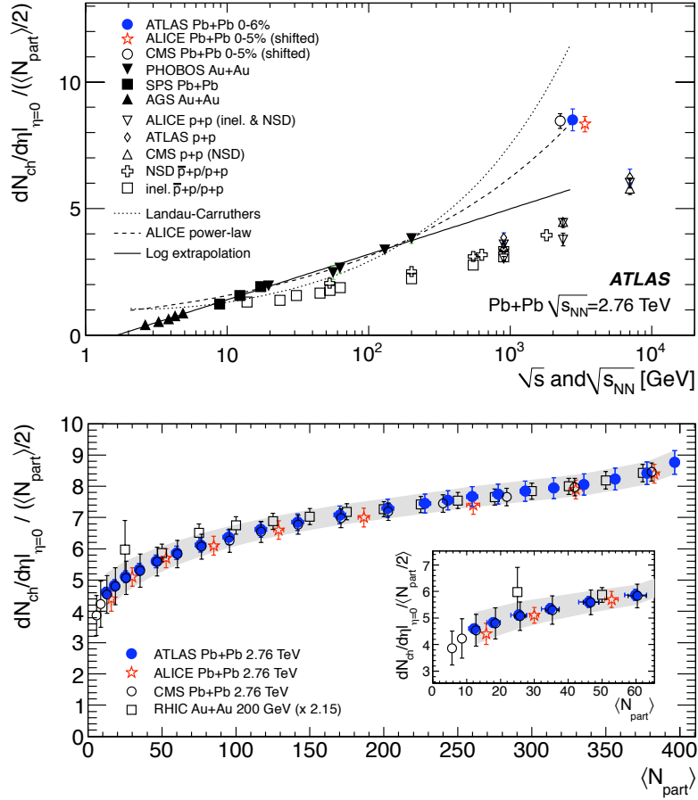
Figure 3: Top: \sqrt{s_{\text{NN}}} dependence of the charged particle dN_{\text{ch}}/d\eta per colliding nucleon pair dN_{\text{ch}}/d\eta|_{\eta=0}/(\langle N_{\text{part}} \rangle/2) from a variety of measurements in p+p and \bar{p} +p (inelastic and non-single diffractive results from [2] and references therein, as well as [31]-[35]) and central A+A collisions, including the ATLAS 0-6% centrality measurement reported here for |\eta| < 0.5 and the previous 0-5% centrality ALICE [8] and CMS [9] measurements (points shifted horizontally for clarity). The curves show different expectations for the \sqrt{s_{\text{NN}}} dependence in A+A collisions: results of a Landau hydrodynamics calculation [7] (dotted line), an s^{0.15} extrapolation of RHIC and SPS data proposed by ALICE [8] (dashed line), a logarithmic extrapolation of RHIC and SPS data from [30] (solid line). Bottom: dN_{\text{ch}}/d\eta|_{\eta=0}/(\langle N_{\text{part}} \rangle/2) vs \langle N_{\text{part}} \rangle for 2% centrality intervals over 0-20% and 5% centrality intervals over 20-80%. Error bars represent combined statistical and systematic uncertainties on the dN_{\text{ch}}/d\eta|_{\eta=0} measurements, whereas the shaded band indicates the total systematic uncertainty including \langle N_{\text{part}} \rangle uncertainties. The RHIC measurements (see text) have been multiplied by 2.15 to allow comparison with the \sqrt{s_{\text{NN}}} = 2.76 TeV results. The inset shows the \langle N_{\text{part}} \rangle < 60 region in more detail.
