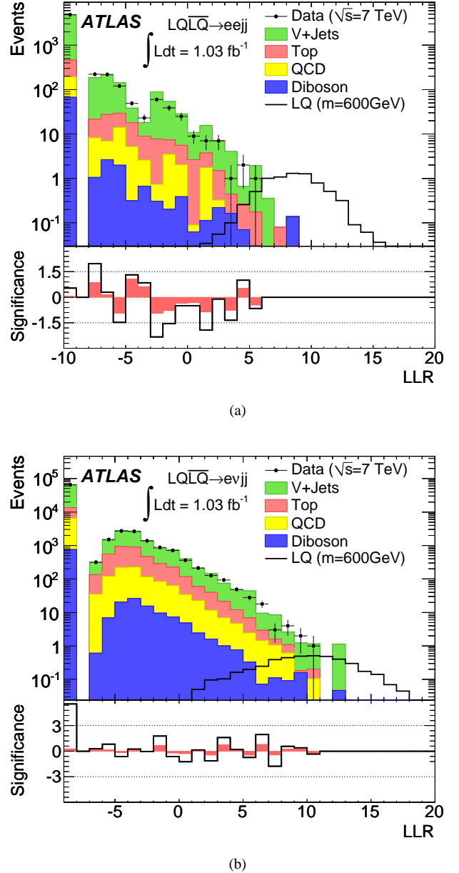
Figure 3: LLR distributions for the eejj (a) and for the evjj (b) final states. The data are indicated with the points and the filled histograms show the SM background. The MJ background is estimated from data, while the other background contributions are obtained from simulated samples as described in the text. The LQ signal corresponding to a LQ mass of 600 GeV is indicated by a solid line, and is normalized assuming \beta = 1.0(0.5) in the eejj ( evjj ) channel. The lowest bin corresponds to background events regions of the phase space for which no signal events are expected. The solid line (band) in the lower plots shows the Gaussian statistical (statistical + systematic) significance of the difference between data and the prediction.
