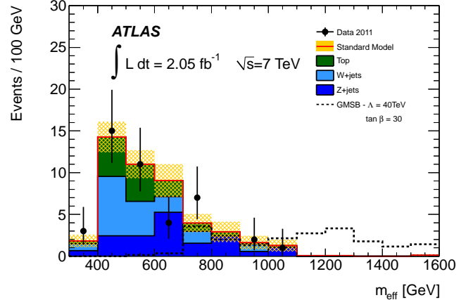
(a) m_{\text{eff}} distribution after the \Delta\phi requirement
