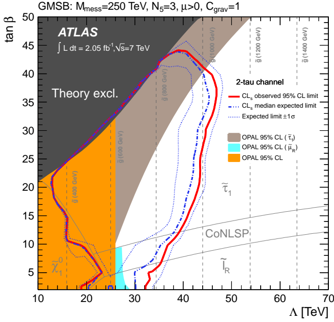
Figure 3: Expected and observed 95% CL limits on the minimal GMSB model parameters \Lambda and \tan\beta . The dark grey area indicates the region which is theoretically excluded due to unphysical sparticle mass values. The different NLSP regions are indicate. In the CoNLSP region the \tilde{\tau}_1 and the \tilde{\ell}_R are the NLSP. Additional model parameters are M_{\text{mess}} = 250 TeV, N_5 = 3 , \mu > 0 and C_{\text{grav}} = 1 . The previous OPAL [19] limits are also shown.
