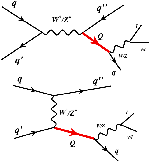
Figure 1: Vector-like quark production and decay diagrams for s -channel (top) and t -channel (bottom). The thick line indicates the vector-like quark.
