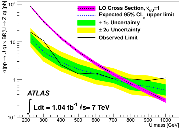
Figure 3: Upper limits at 95% confidence level on the cross section times branching ratio \sigma(pp \rightarrow Qq) \times BR(Q \rightarrow Vq) for the CC (top) and NC (bottom) channels as a function of mass. The function-of-mass (LO) theoretical cross section assumes \tilde{\kappa}_{uD} = 1 and \tilde{\kappa}_{uU} = 1 on the top and bottom respectively. The width of the dark band around it corresponds to the theoretical uncertainty described in the text. The expected cross section upper limit is determined by the median result of background-only pseudoexperiments, and is shown with its 1\sigma and 2\sigma uncertainties, respectively.
