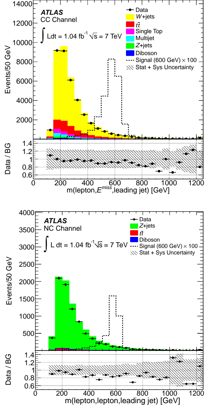
Figure 2: Invariant mass distribution of VLQ candidates in both the CC (top) and NC (bottom) channels, summed over both the electron and muon final states. The dashed line shows the signal shape, normalized by 100 times the leading order theoretical cross section. The bottom part of each plot shows the ratio of the data to the background model. The last bin contains events with invariant mass candidates equal to or higher than 1200 GeV.
