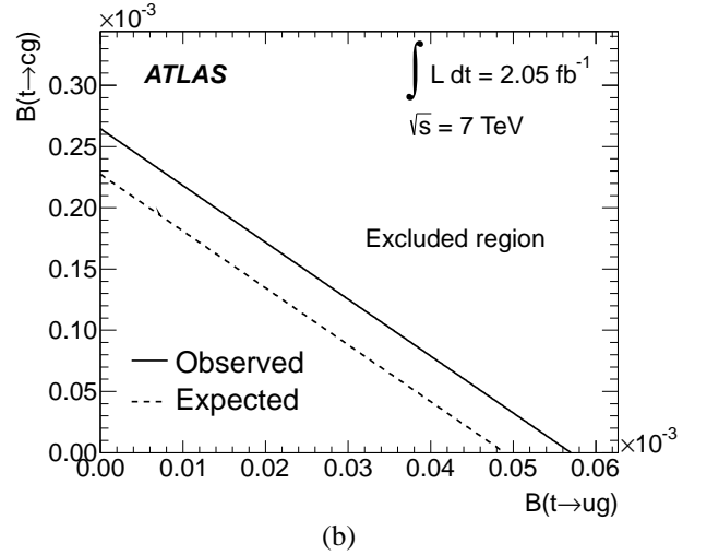
Figure 5: Upper limit (a) on the coupling constants \kappa_{ugt}/\Lambda and \kappa_{cgt}/\Lambda and (b) on the branching fractions t \rightarrow ug and t \rightarrow cg .
