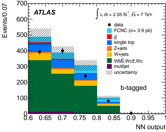
Figure 4: Distributions of the neural network output: Observed signal and simulated background output distribution normalised to the mean value of the marginalised nuisance parameters, zoomed into the signal region. The FCNC single top quark process is normalised to the observed limit of 3.9 pb. The hatched band indicates the statistical uncertainty from the sizes of the simulated samples and the uncertainty in the background normalisation.
