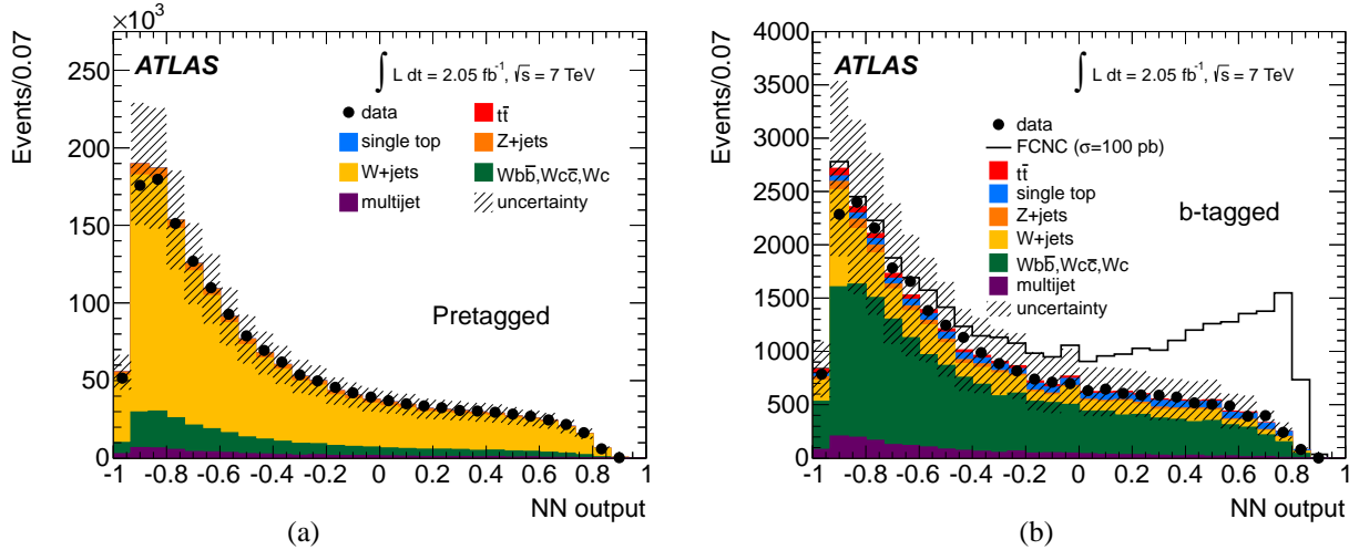
Figure 2: (a) Neural network output distribution scaled to the number of observed events in the pretagged sample. (b) Neural network output distribution scaled to the number of observed events in the b -tagged sample. In these distributions the signal contribution is shown stacked on top of the backgrounds. The hatched band indicates the statistical uncertainty from the sizes of the simulated samples and the uncertainty in the background normalisation.
