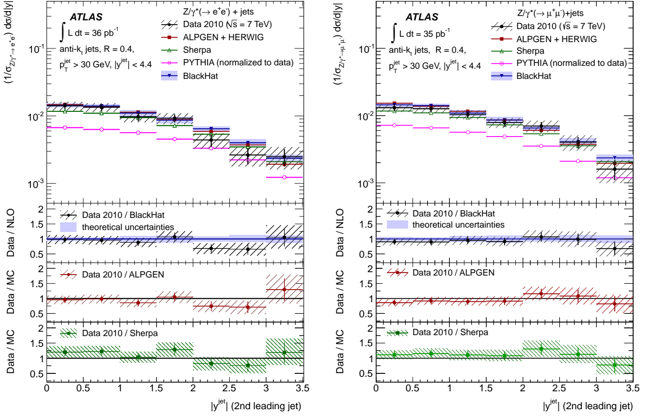
FIG. 10: Measured normalized jet cross section (1/\sigma_{Z/\gamma^* \rightarrow \ell^+\ell^-}) d^2\sigma/d|y| (black dots) in (left) Z/\gamma^* \rightarrow e^+e^- + \text{jets} and (right) Z/\gamma^* \rightarrow \mu^+\mu^- + \text{jets} production as a function of the second-leading jet |y| , in events with at least two jets with p_T > 30 GeV and |y| < 4.4 in the final state, and normalized by \sigma_{Z/\gamma^* \rightarrow e^+e^-} and \sigma_{Z/\gamma^* \rightarrow \mu^+\mu^-} Drell-Yan cross sections, respectively.
