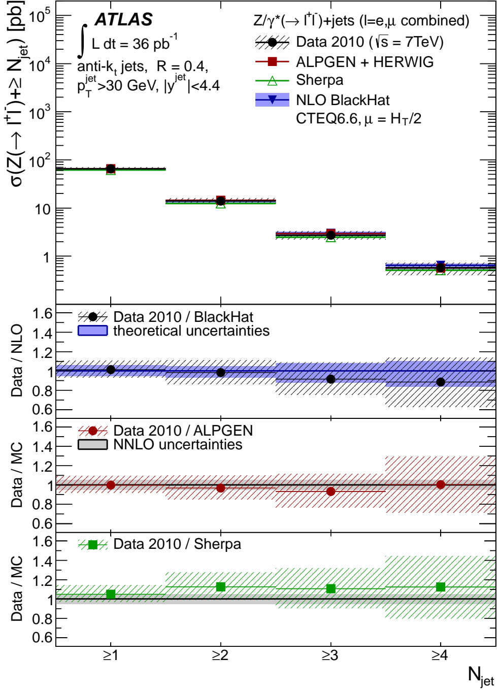
FIG. 15: Measured cross section \sigma_{N_{\text{jet}}} (black dots) in Z/\gamma^*(\rightarrow \ell^+\ell^-)+\text{jets} production as a function of the inclusive jet multiplicity, for events with at least one jet with p_T > 30 \text{ GeV} and |y| < 4.4 in the final state. In this and subsequent figures 16 - 26 the error bands indicate the total uncertainty from the combination of electron and muon results. The measurements are compared to NLO pQCD predictions from BlackHat, as well as the predictions from ALPGEN and Sherpa (both normalized to the FEWZ value for the total cross section).
