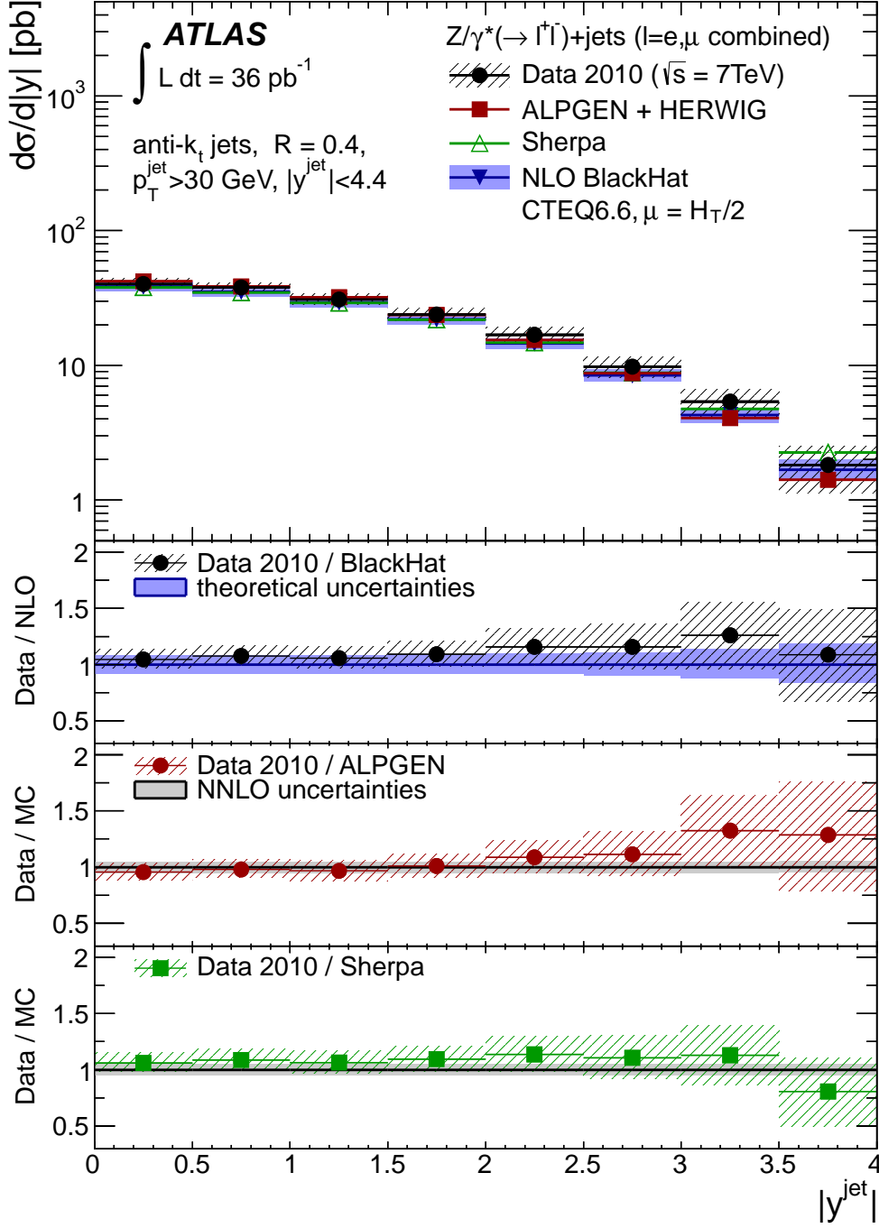
FIG. 20: Measured inclusive jet cross section d\sigma/d|y| (black dots) in Z/\gamma^*(\rightarrow \ell^+\ell^-)+\text{jets} production as a function of |y| , in events with at least one jet with p_T > 30 \text{ GeV} and |y| < 4.4 in the final state.
