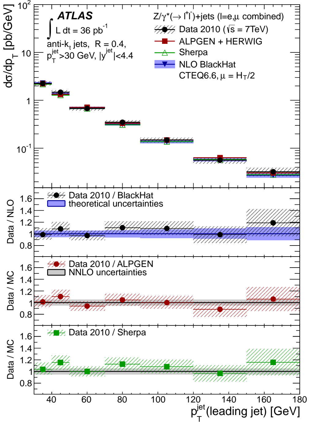
FIG. 18: Measured jet cross section d\sigma/dp_T (black dots) in Z/\gamma^*(\rightarrow \ell^+\ell^-)+\text{jets} production as a function of the leading jet p_T , in events with at least one jet with p_T > 30 \text{ GeV} and |y| < 4.4 in the final state.
