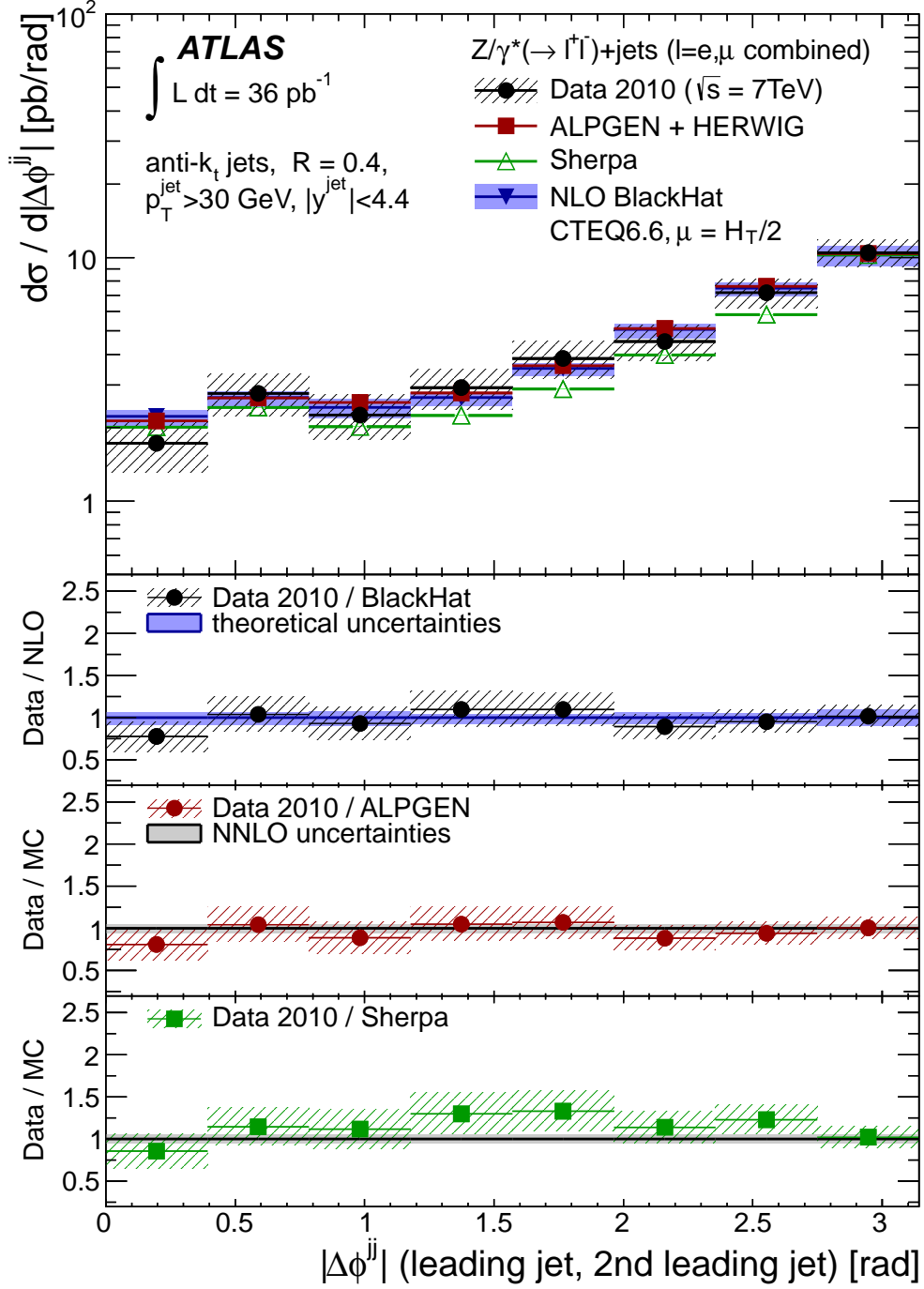
FIG. 25: Measured dijet cross section d\sigma/d|\Delta\phi^{jj}| (black dots) in Z/\gamma^*(\rightarrow \ell^+\ell^-)+\text{jets} production as a function of the azimuthal separation of the two leading jets |\Delta\phi^{jj}| , in events with at least two jets with p_T > 30 \text{ GeV} and |y| < 4.4 in the final state.
