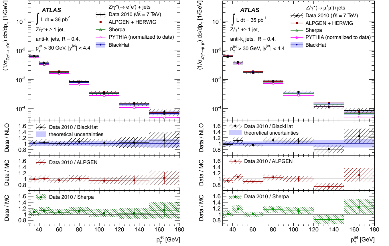
FIG. 5: Measured normalized inclusive jet cross section (1/\sigma_{Z/\gamma^* \rightarrow \ell^+ \ell^-}) d\sigma/dp_T (black dots) in (left) Z/\gamma^*(\rightarrow e^+e^-)+\text{jets} and (right) Z/\gamma^*(\rightarrow \mu^+\mu^-)+\text{jets} production as a function of p_T , in events with at least one jet with p_T > 30 GeV and |y| < 4.4 in the final state, and normalized by \sigma_{Z/\gamma^* \rightarrow e^+e^-} and \sigma_{Z/\gamma^* \rightarrow \mu^+\mu^-} Drell-Yan cross sections, respectively.
