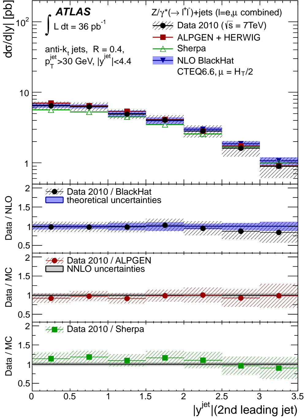
FIG. 22: Measured jet cross section d\sigma/d|y| (black dots) in Z/\gamma^*(\rightarrow \ell^+\ell^-)+\text{jets} production as a function of the second-leading jet |y| , in events with at least two jets with p_T > 30 \text{ GeV} and |y| < 4.4 in the final state.
