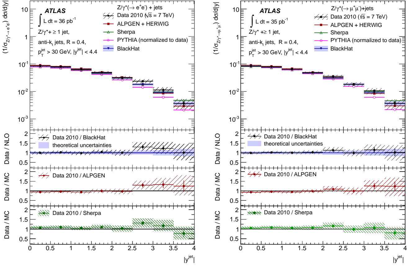
FIG. 8: Measured normalized inclusive jet cross section (1/\sigma_{Z/\gamma^* \rightarrow \ell^+ \ell^-}) d\sigma/d|y| (black dots) in (left) Z/\gamma^*(\rightarrow e^+e^-)+\text{jets} and (right) Z/\gamma^*(\rightarrow \mu^+\mu^-)+\text{jets} production as a function of |y| , in events with at least one jet with p_T > 30 GeV and |y| < 4.4 in the final state, and normalized by \sigma_{Z/\gamma^* \rightarrow e^+e^-} and \sigma_{Z/\gamma^* \rightarrow \mu^+\mu^-} Drell-Yan cross sections, respectively.
