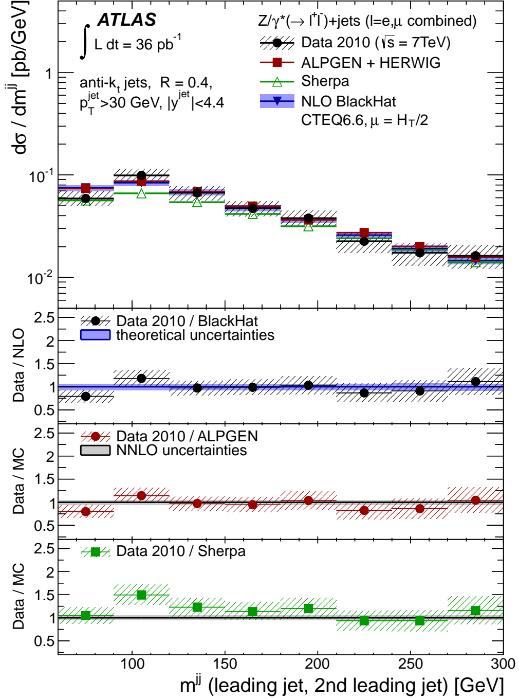
FIG. 23: Measured dijet cross section d\sigma/dm^{jj} (black dots) in Z/\gamma^*(\rightarrow \ell^+\ell^-)+\text{jets} production as a function of the invariant mass of the two leading jets m^{jj} , in events with at least two jets with p_T > 30 \text{ GeV} and |y| < 4.4 in the final state.
