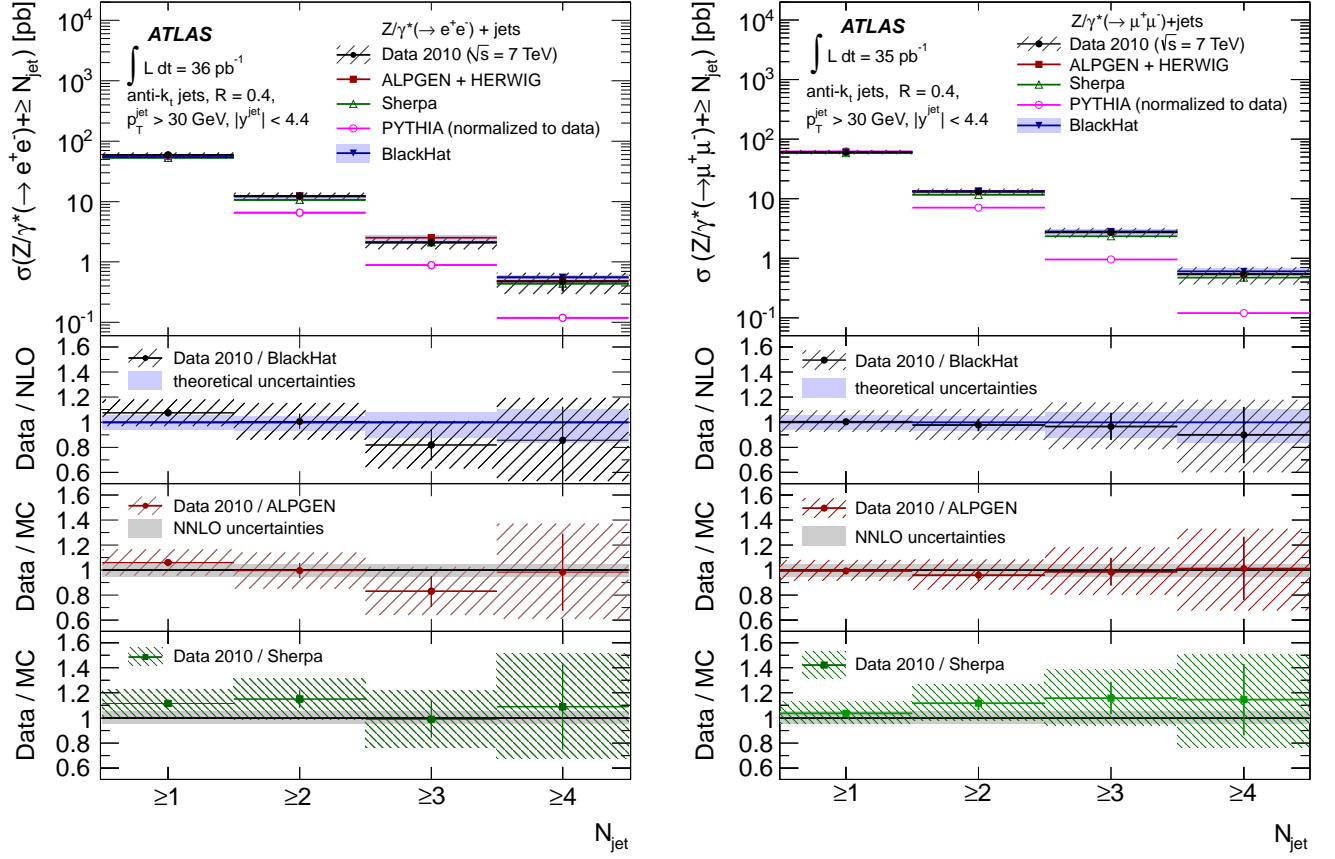
FIG. 3: Measured cross section \sigma_{N_{\text{jet}}} (black dots) for (left) Z/\gamma^* \rightarrow e^+e^- + \text{jets} and (right) Z/\gamma^* \rightarrow \mu^+\mu^- + \text{jets} production as a function of the inclusive jet multiplicity, for events with at least one jet with p_T > 30 \text{ GeV} and |y| < 4.4 in the final state. In this and subsequent figures 4 - 14 the error bars indicate the statistical uncertainty and the dashed areas the statistical and systematic uncertainties added in quadrature. The measurements are compared to NLO pQCD predictions from BlackHat, as well as the predictions from ALPGEN and Sherpa (both normalized to the FEWZ value for the total cross section), and PYTHIA (normalized to the data as discussed in Section XII).
