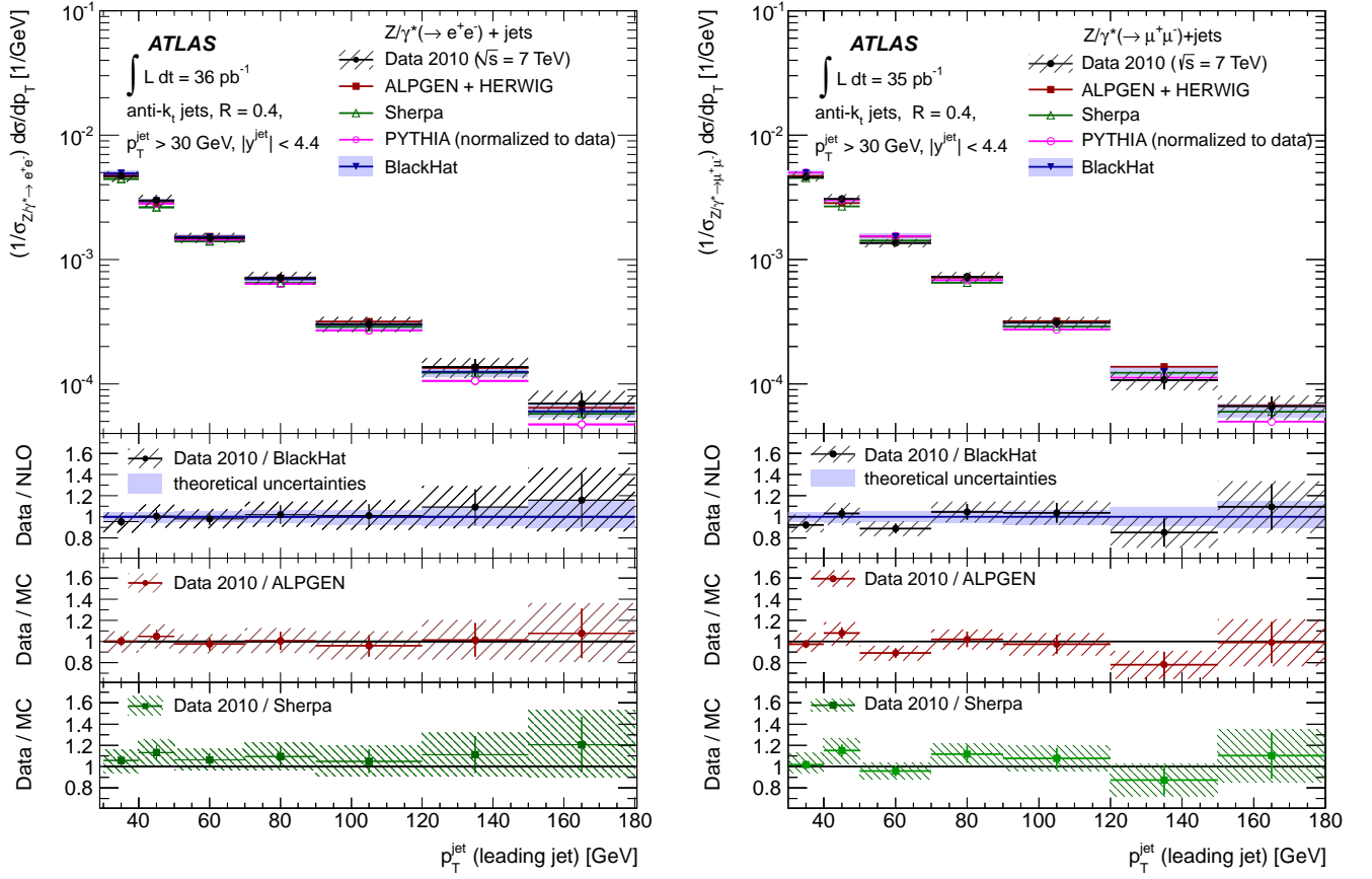
FIG. 6: Measured normalized jet cross section (1/\sigma_{Z/\gamma^* \rightarrow \ell^+ \ell^-}) d\sigma/dp_T (black dots) in (left) Z/\gamma^* (\rightarrow e^+ e^-) + \text{jets} and (right) Z/\gamma^* (\rightarrow \mu^+ \mu^-) + \text{jets} production as a function of the leading jet p_T , in events with at least one jet with p_T > 30 GeV and |y| < 4.4 in the final state, and normalized by \sigma_{Z/\gamma^* \rightarrow e^+ e^-} and \sigma_{Z/\gamma^* \rightarrow \mu^+ \mu^-} Drell-Yan cross sections, respectively.
