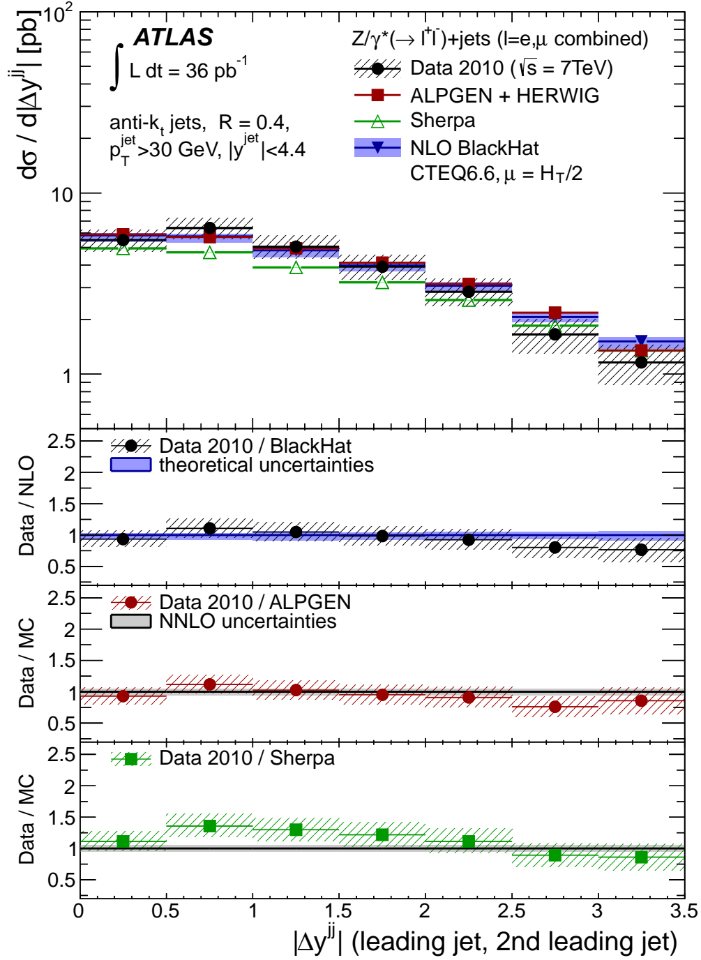
FIG. 24: Measured dijet cross section d\sigma/d|\Delta y^{\text{jj}}| (black dots) in Z/\gamma^*(\rightarrow \ell^+\ell^-)+\text{jets} production as a function of the rapidity separation of the two leading jets |\Delta y^{\text{jj}}| , in events with at least two jets with p_T > 30 \text{ GeV} and |y| < 4.4 in the final state.
