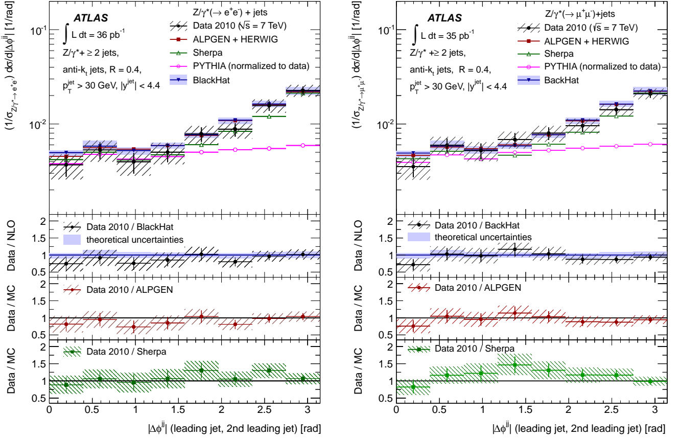
FIG. 13: Measured normalized dijet cross section (1/\sigma_{Z/\gamma^* \rightarrow \ell^+ \ell^-}) d\sigma/d|\Delta\phi^{jj}| (black dots) in (left) Z/\gamma^* (\rightarrow e^+ e^-) + \text{jets} and (right) Z/\gamma^* (\rightarrow \mu^+ \mu^-) + \text{jets} production as a function of the azimuthal separation of the two leading jets |\Delta\phi^{jj}| , in events with at least two jets with p_T > 30 GeV and |y| < 4.4 in the final state, and normalized by \sigma_{Z/\gamma^* \rightarrow e^+ e^-} and \sigma_{Z/\gamma^* \rightarrow \mu^+ \mu^-} Drell-Yan cross sections, respectively.
