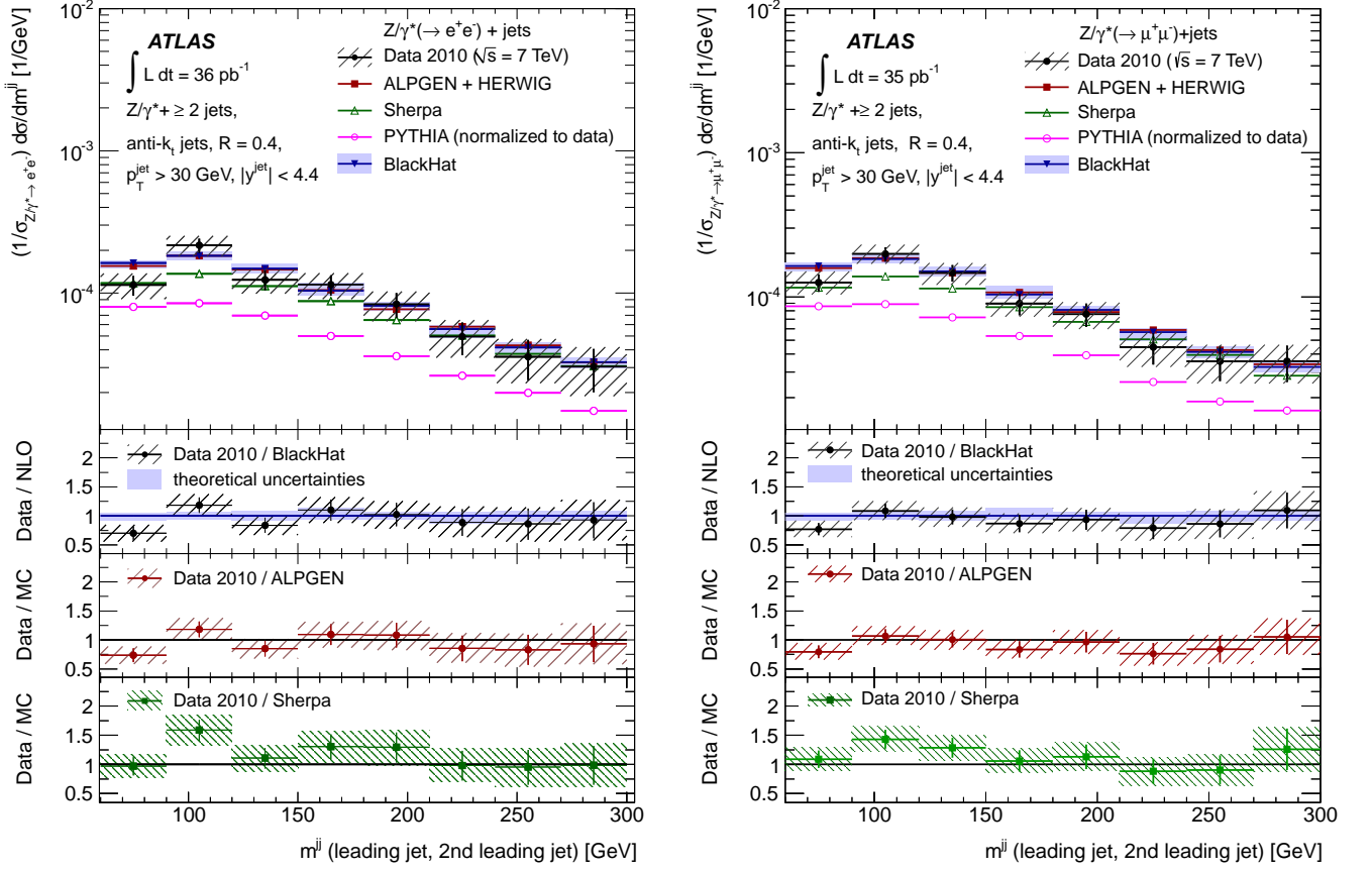
FIG. 11: Measured normalized dijet cross section (1/\sigma_{Z/\gamma^* \rightarrow \ell^+ \ell^-}) d\sigma/dm^{jj} (black dots) in (left) Z/\gamma^* (\rightarrow e^+ e^-) + \text{jets} and (right) Z/\gamma^* (\rightarrow \mu^+ \mu^-) + \text{jets} production as a function of the invariant mass of the two leading jets m^{jj} , in events with at least two jets with p_T > 30 GeV and |y| < 4.4 in the final state, and normalized by \sigma_{Z/\gamma^* \rightarrow e^+ e^-} and \sigma_{Z/\gamma^* \rightarrow \mu^+ \mu^-} Drell-Yan cross sections, respectively.
