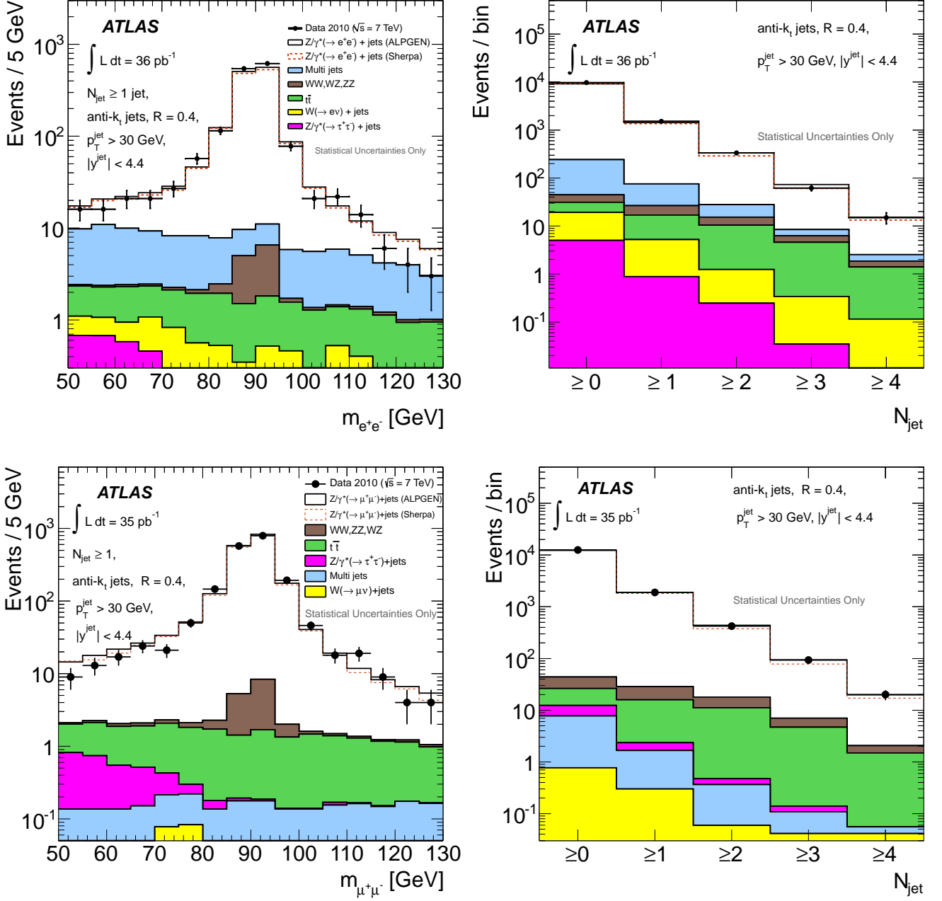
FIG. 1: Uncorrected dilepton invariant mass in (top) Z/\gamma^* \rightarrow e^+e^- and (bottom) Z/\gamma^* \rightarrow \mu^+\mu^- events with at least one jet in the final state, shown in a wider dilepton mass region than the one selected (left), and uncorrected inclusive jet multiplicity (right), for jets with p_T > 30 GeV and |y| < 4.4 (black dots), and in the mass range 66 \text{ GeV} < m_{\ell^+\ell^-} < 116 \text{ GeV} ( \ell = e, \mu ). Only statistical uncertainties are shown. The data are compared to predictions for signal (ALPGEN and Sherpa, both normalized to the FEWZ value for the total cross section) and background processes (filled histograms).
