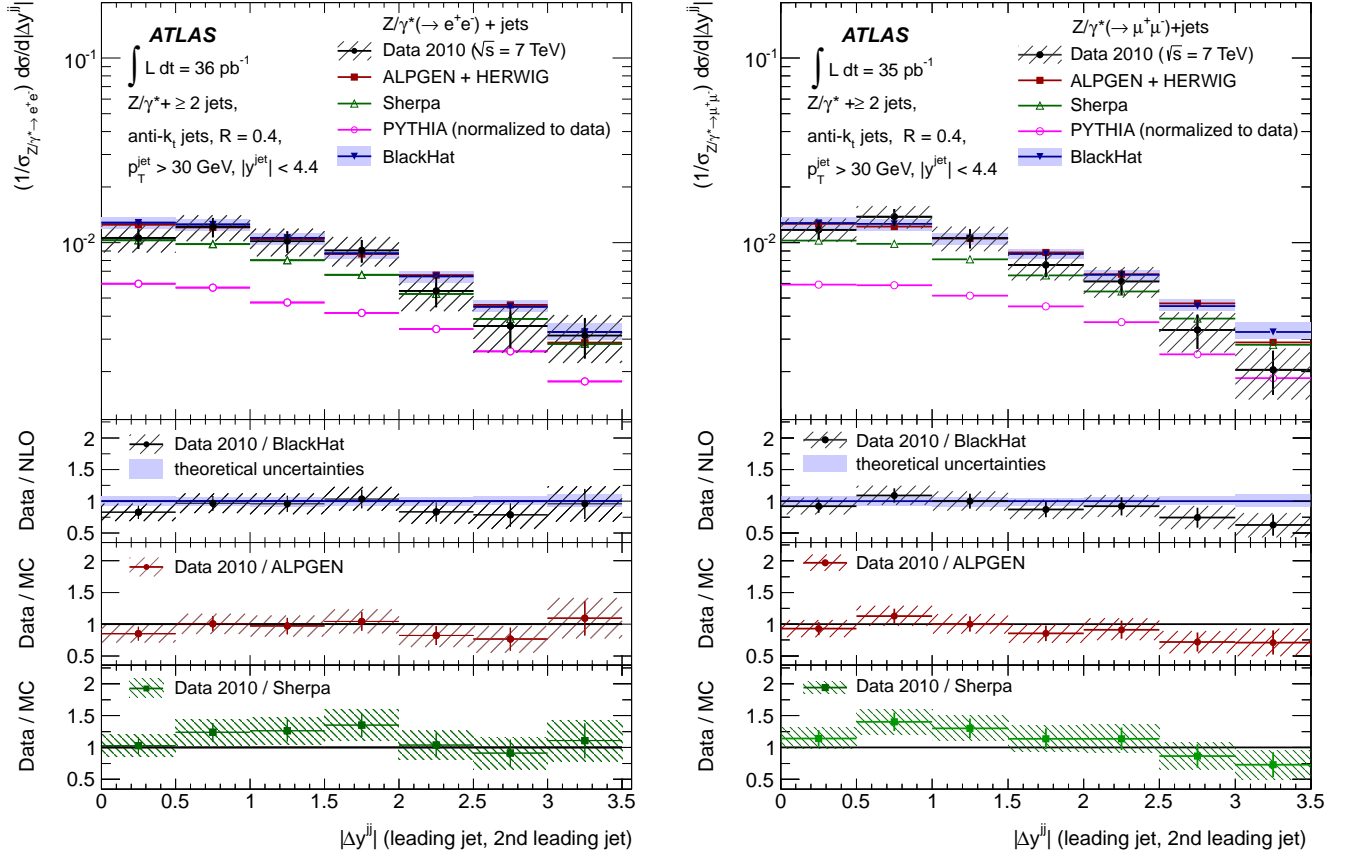
FIG. 12: Measured normalized dijet cross section (1/\sigma_{Z/\gamma^* \rightarrow \ell^+ \ell^-}) d\sigma/d|\Delta y^{jj}| (black dots) in (left) Z/\gamma^* (\rightarrow e^+ e^-) + \text{jets} and (right) Z/\gamma^* (\rightarrow \mu^+ \mu^-) + \text{jets} production as a function of the rapidity separation of the two leading jets |\Delta y^{jj}| , in events with at least two jets with p_T > 30 GeV and |y| < 4.4 in the final state, and normalized by \sigma_{Z/\gamma^* \rightarrow e^+ e^-} and \sigma_{Z/\gamma^* \rightarrow \mu^+ \mu^-} Drell-Yan cross sections, respectively.
