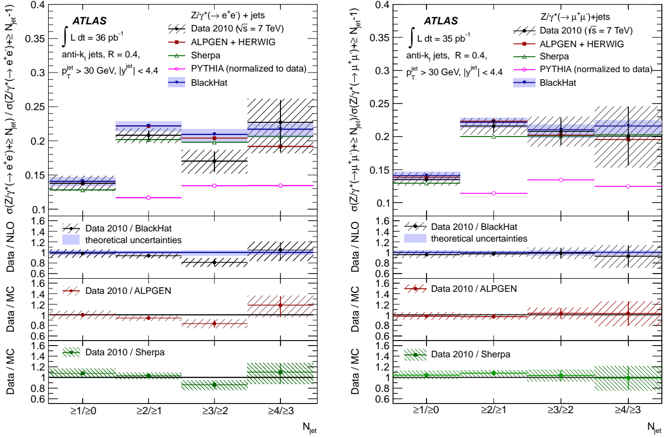
FIG. 4: Measured ratio of cross sections ( \sigma_{N_{jet}}/\sigma_{N_{jet}-1} ) (black dots) for (left) Z/\gamma^*(\rightarrow e^+e^-)+j\geq N_{jet} and (right) Z/\gamma^*(\rightarrow \mu^+\mu^-)+j\geq N_{jet} production as a function of the inclusive jet multiplicity, for events with at least one jet with p_T > 30 \text{ GeV} and |y| < 4.4 in the final state.
