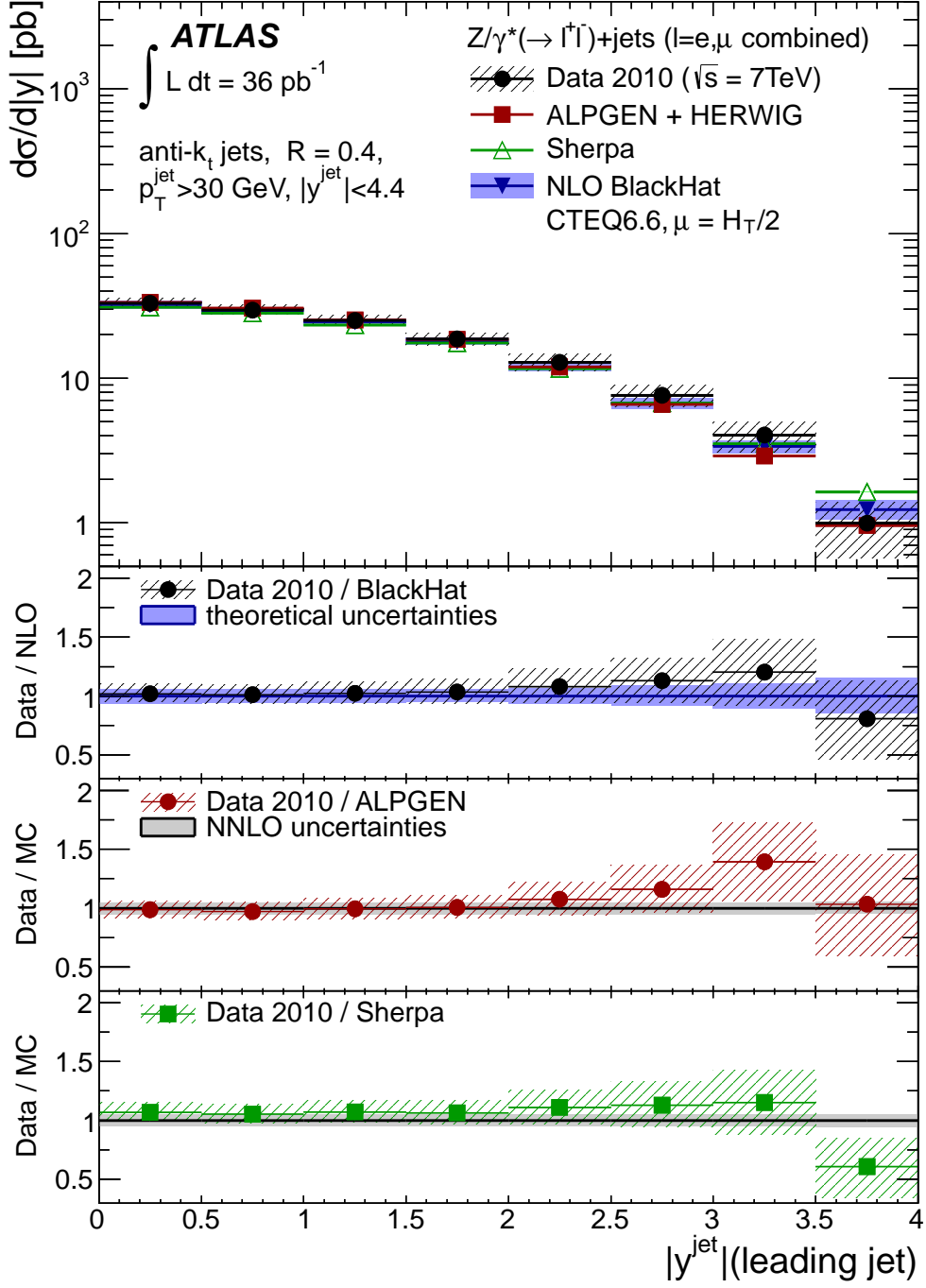
FIG. 21: Measured jet cross section d\sigma/d|y| (black dots) in Z/\gamma^*(\rightarrow \ell^+\ell^-)+\text{jets} production as a function of the leading jet |y| , in events with at least one jet with p_T > 30 \text{ GeV} and |y| < 4.4 in the final state.
