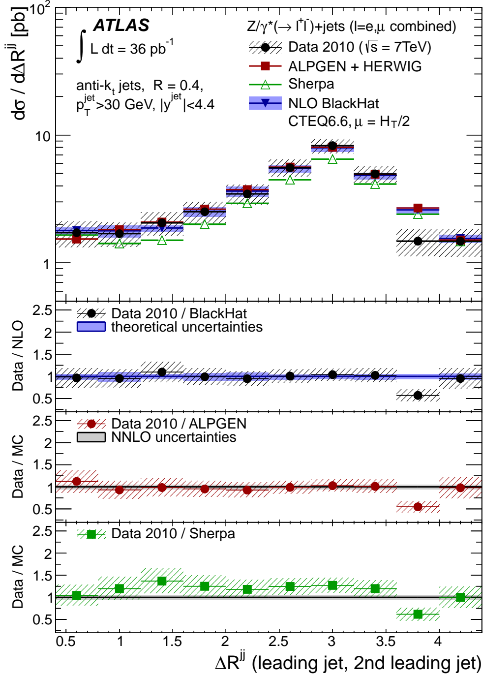
FIG. 26: Measured dijet cross section d\sigma/d\Delta R^{jj} (black dots) in Z/\gamma^*(\rightarrow \ell^+\ell^-)+\text{jets} production as a function of the angular separation ( y - \phi space) of the two leading jets \Delta R^{jj} , in events with at least two jets with p_T > 30 \text{ GeV} and |y| < 4.4 in the final state.
