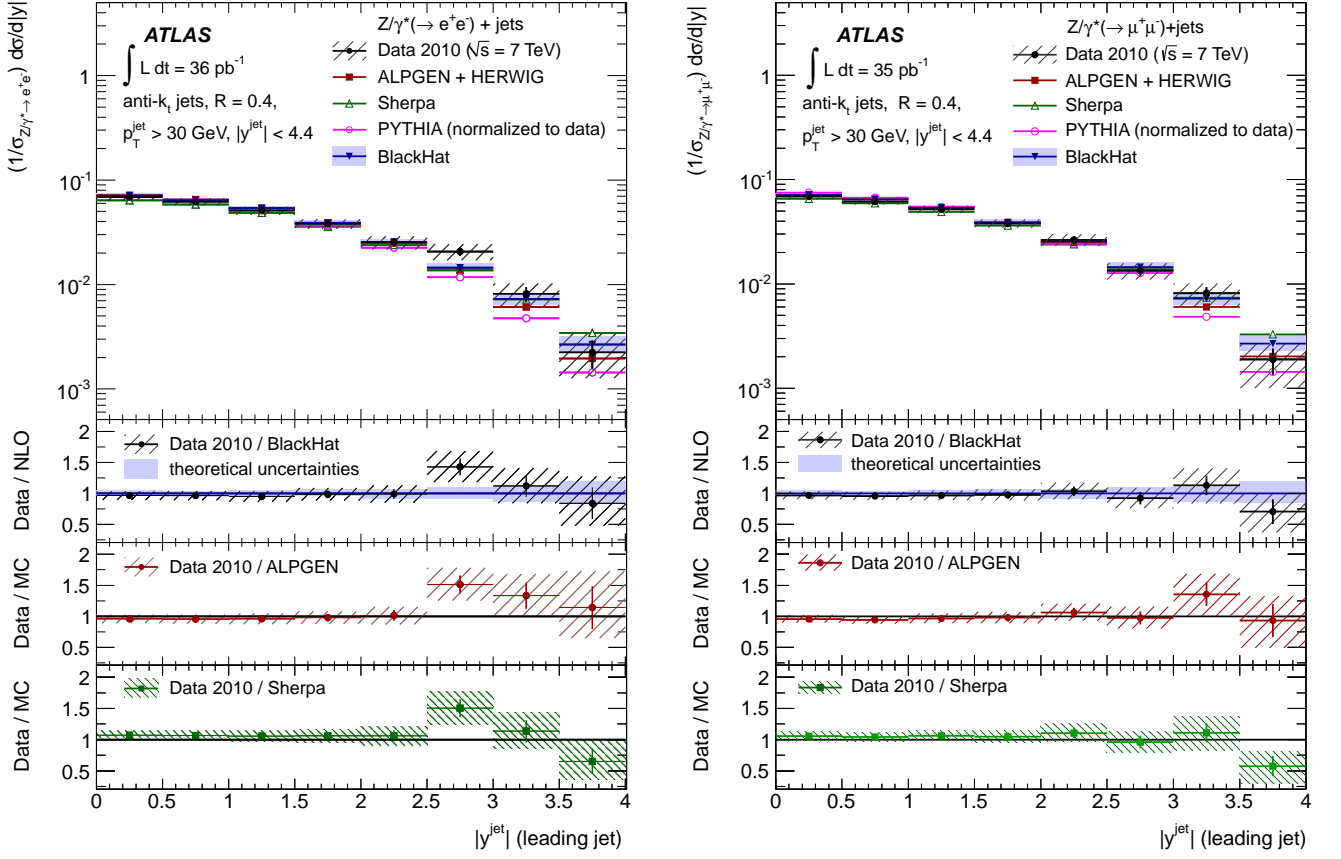
FIG. 9: Measured normalized jet cross section (1/\sigma_{Z/\gamma^* \rightarrow \ell^+\ell^-})d\sigma/d|y| (black dots) in (left) Z/\gamma^* \rightarrow e^+e^- + \text{jets} and (right) Z/\gamma^* \rightarrow \mu^+\mu^- + \text{jets} production as a function of the leading jet |y| , in events with at least one jet with p_T > 30 \text{ GeV} and |y| < 4.4 in the final state, and normalized by \sigma_{Z/\gamma^* \rightarrow e^+e^-} and \sigma_{Z/\gamma^* \rightarrow \mu^+\mu^-} Drell-Yan cross sections, respectively.
