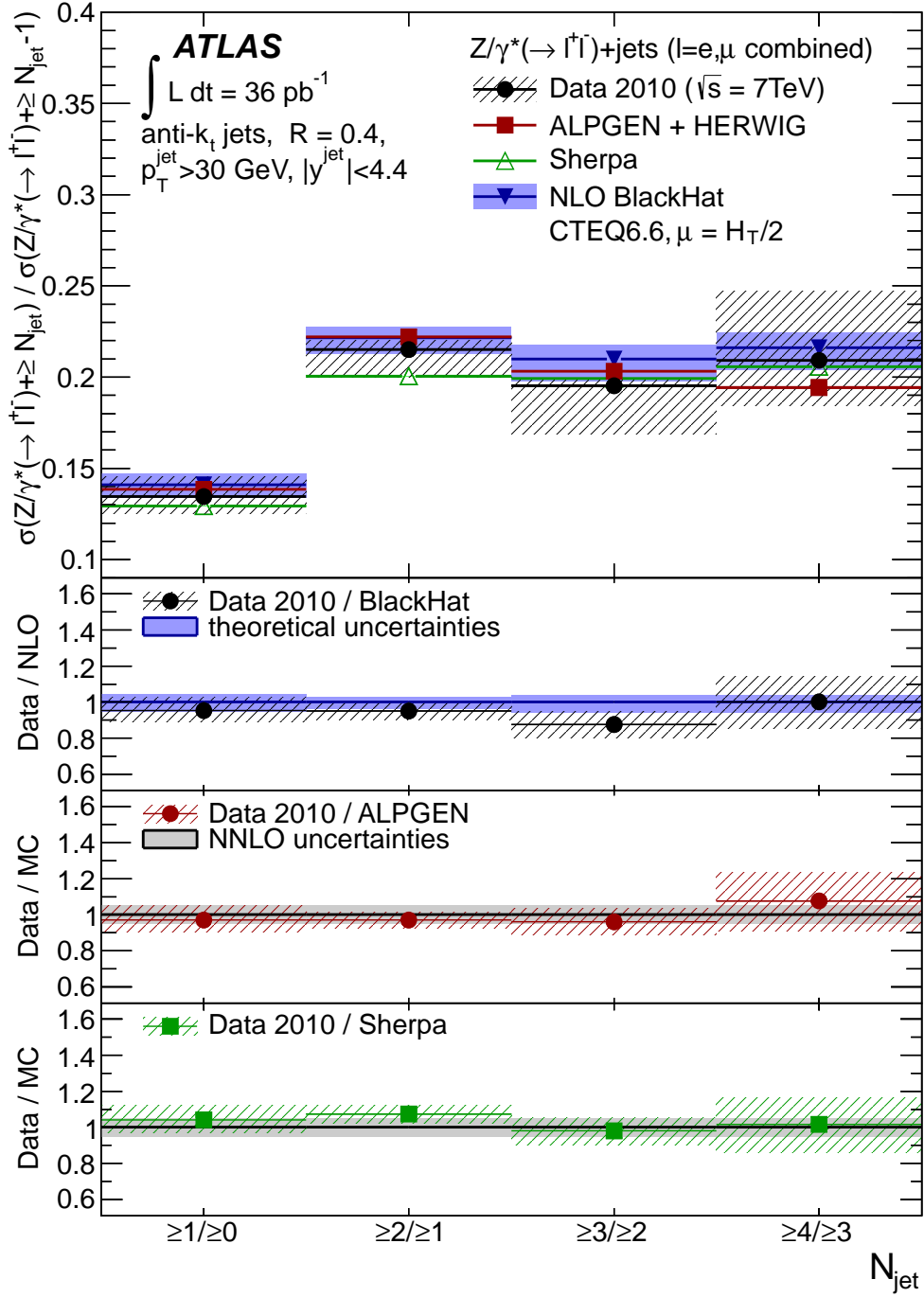
FIG. 16: Measured ratio of cross sections ( \sigma_{N_{\text{jet}}}/\sigma_{N_{\text{jet}}-1} ) (black dots) in Z/\gamma^*(\rightarrow \ell^+\ell^-)+\text{jets} production as a function of the inclusive jet multiplicity, for events with at least one jet with p_T > 30 \text{ GeV} and |y| < 4.4 in the final state.
