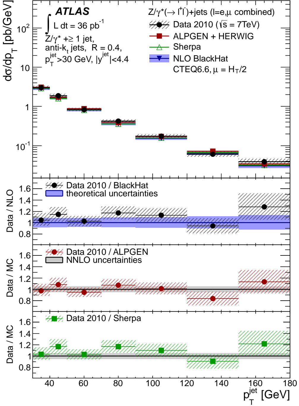
FIG. 17: Measured inclusive jet cross section d\sigma/dp_T (black dots) in Z/\gamma^*(\rightarrow \ell^+\ell^-)+\text{jets} production as a function of p_T , in events with at least one jet with p_T > 30 \text{ GeV} and |y| < 4.4 in the final state.
