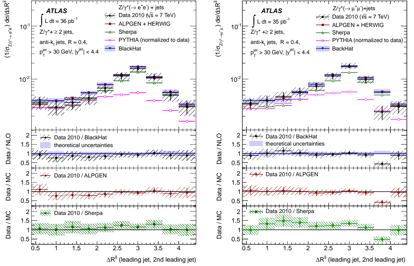
FIG. 14: Measured normalized dijet cross section (1/\sigma_{Z/\gamma^* \rightarrow \ell^+ \ell^-}) d\sigma/d\Delta R^{jj} (black dots) in (left) Z/\gamma^* (\rightarrow e^+ e^-) + \text{jets} and (right) Z/\gamma^* (\rightarrow \mu^+ \mu^-) + \text{jets} production as a function of the angular separation ( y - \phi space) of the two leading jets \Delta R^{jj} , in events with at least two jets with p_T > 30 GeV and |y| < 4.4 in the final state, and normalized by \sigma_{Z/\gamma^* \rightarrow e^+ e^-} and \sigma_{Z/\gamma^* \rightarrow \mu^+ \mu^-} Drell-Yan cross sections, respectively.
