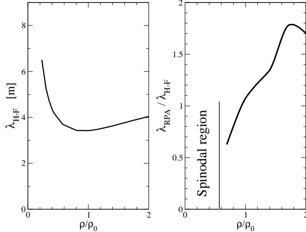
Fig. 4. The neutrino mean-free path is plotted as a function of the density for asymmetric nuclear matter at T=10 MeV and Y_l=0.285 . Left panel: HF result, right panel: ratio between RPA and HF mean-free paths.
