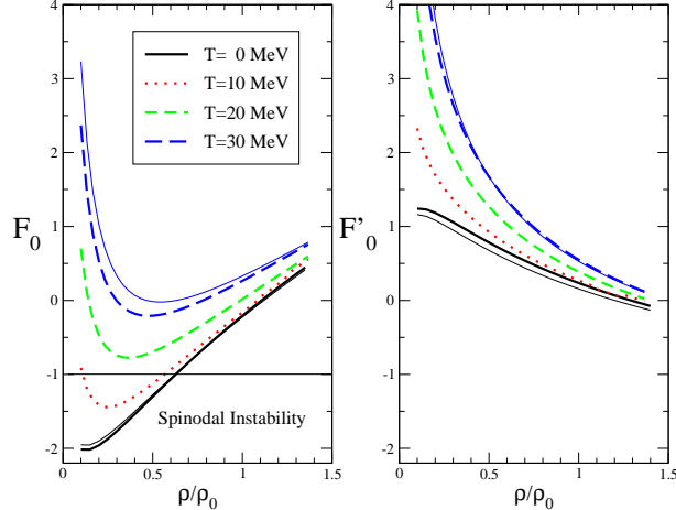
Fig. 1. (color online) The adimensional Landau parameters F_0 and F'_0 are plotted as a function of the density at several values of temperature. The thin line represent a calculation of the same quantity in asymmetric nuclear matter with x_p = 0.25 and for T = 0 and 30 MeV. The definitions F_0 = (F_0^{nn} + F_0^{pp} + 2F_0^{np})/2 and F'_0 = (F_0^{nn} + F_0^{pp} - 2F_0^{np})/2 has been taken and the coefficients F_0^{\tau\tau'} are the second derivative of the free energy density with respect to the densities. The onset for the spinodal instability is given by F_0 = -1 .
