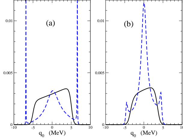
Fig. 3. (color online) The density-density response function \mathcal{S}^{(0)}(q, T) is plotted as a function of the transferred energy for two values of the density: (a) \rho_0 and (b) 0.75\rho_0 . The calculations have been done for momentum q = 10 MeV, temperature T = 10 MeV and leptonic fraction Y_l=0.285 . The solid and dashed lines stand for the HF and the RPA results respectively.
