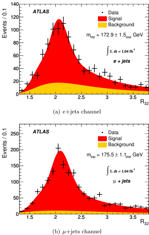
Fig. 7 1d-analysis: The R_{32} distribution observed in the data together with the signal and background contributions determined by the fit. The distributions are for (a) the e+jets channel and (b) the \mu+jets channel. The data points are shown with their statistical uncertainties.
