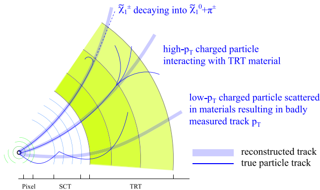
Fig. 2 Origins of disappearing high- p_{\text{T}} tracks.
