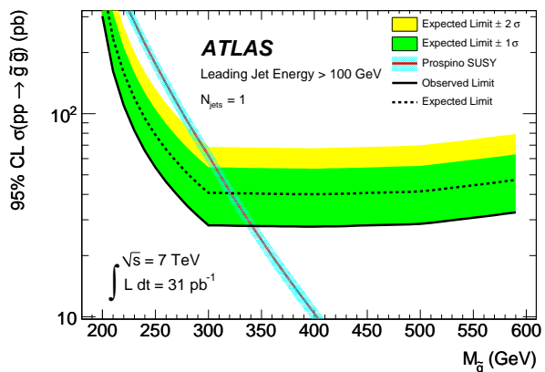
Fig. 4 The 95% C.L. limit on the gluino pair production cross-section as a function of gluino mass, m_{\tilde{g}} , assuming m_{\tilde{\chi}_1^0} = 100 \text{ GeV} . Limits are shown for the Generic stopping model and \tilde{g} \rightarrow g\tilde{\chi}^0 decay.
