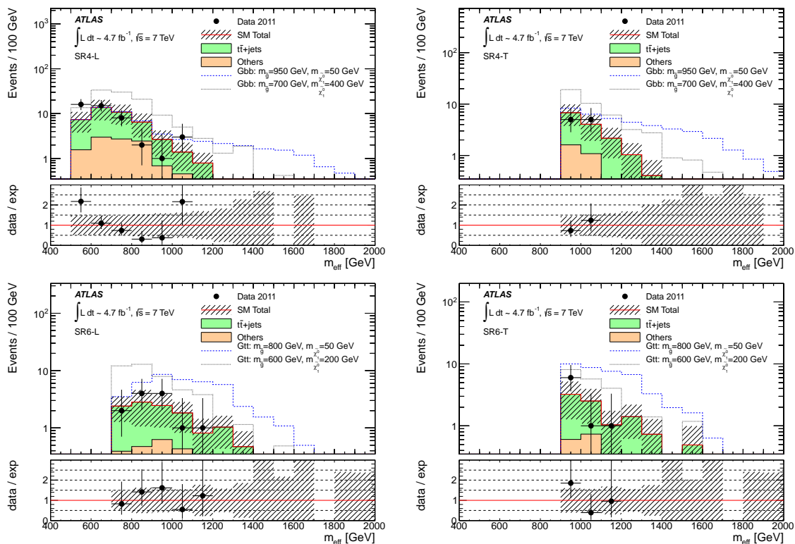
Fig. 1 Distribution of m_{\text{eff}} for SR4-L and SR4-T (top) and SR6-L and SR6-T (bottom). The hatched band shows the systematic uncertainty on the MC prediction, which includes both experimental uncertainties (among which JES and b -tagging uncertainties are dominant) and theoretical uncertainties on the background normalisation and shape. The label “others” includes the contributions from single top, t\bar{t}+b\bar{b} , t\bar{t}+W/Z , W/Z +jets and multi-jet processes. The lower plot in each figure shows the ratio of the observed distribution to that expected for the SM background. Two signal points (with small and large mass splitting between the gluino and the LSP) for the Gbb and Gtt models described in the text are overlaid.
